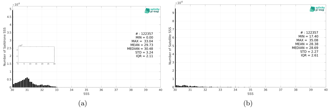
Figure 2: Histograms of SSS from Saildrone (a) and SMOS SSS L3 Arctic v1.1 - 7-Day running mean (CATDS-CEC-LOCEAN) (b) considering all match-up pairs per bins of 0.1 over the Global Ocean Pi-MEP region and for the full satellite product period.
