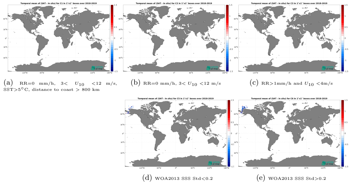
Figure 12: Temporal mean gridded over spatial boxes of size 1^{\circ}\times 1^{\circ} of \Delta\text{SSS} (SMOS SSS L3 Arctic v1.1 - 7-Day running mean (CATDS-CEC-LOCEAN) - Saildrone) for 5 different subdatasets corresponding to:RR=0 mm/h, 3 < U_{10} < 12 m/s, SST >5^{\circ}\text{C} , distance to coast > 800 km (a), RR=0 mm/h, 3 < U_{10} < 12 m/s (b), RR >1 mm/h and U_{10} < 4 m/s (c), WOA2013 SSS Std <0.2 (d), WOA2013 SSS Std >0.2 (e).
