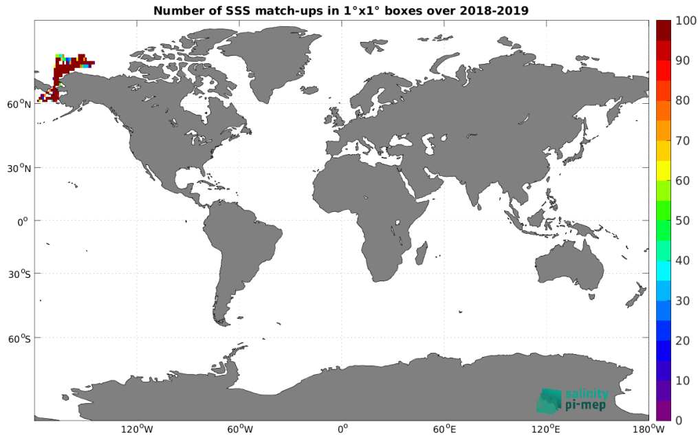
Figure 4: Number of SSS match-ups between Sairdrone SSS and the SMOS SSS L3 Arctic v1.1 - 7-Day running mean (CATDS-CEC-LOCEAN) SSS product for the Global Ocean Pi-MEP region over 1^\circ \times 1^\circ boxes and for the full satellite product period.
