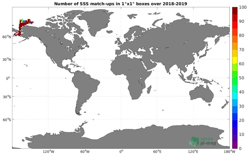
Figure 4: Number of SSS match-ups between Saildrone SSS and the SMOS SSS L3 Arctic v1.1 - 7-Day running mean (CATDS-CECOS-LOCEAN) SSS product for the Global Ocean Pi-MEP region over 1^\circ \times 1^\circ boxes and for the full satellite product period.
