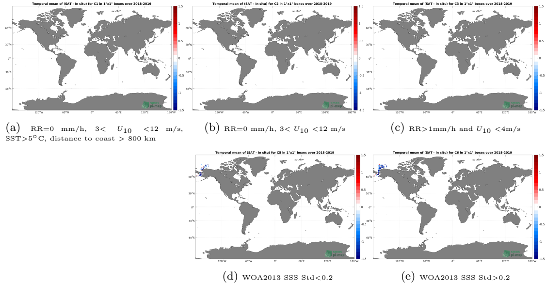
Figure 12: Temporal mean gridded over spatial boxes of size 1^{\circ}\times 1^{\circ} of \Delta\text{SSS} (SMOS SSS L3 Arctic v1.1 - 7-Day running mean (CATDS-CECOS-LOCEAN) - Saildrone) for 5 different subdatasets corresponding to:RR=0 mm/h, 3 < U_{10} < 12 m/s, SST >5^{\circ}\text{C} , distance to coast > 800 km (a), RR=0 mm/h, 3 < U_{10} < 12 m/s (b), RR >1 mm/h and U_{10} < 4 m/s (c), WOA2013 SSS Std <0.2 (d), WOA2013 SSS Std >0.2 (e).
