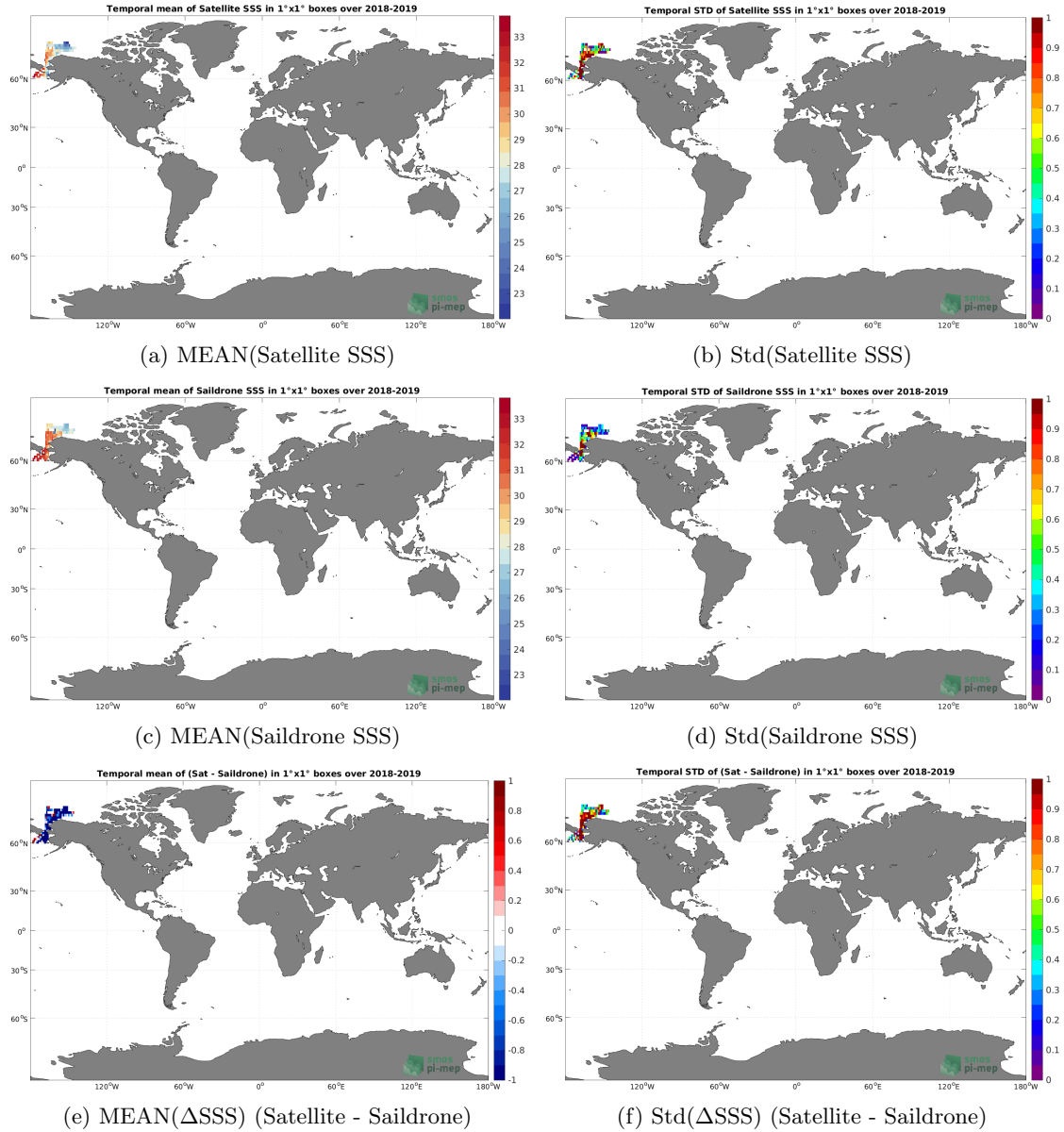
Figure 6: Temporal mean (left) and Std (right) of SSS from SMOS SSS L3 Arctic v1.1 - 7-Day running mean (CATDS-CECOS-LOCEAN) (top), Saildrone (middle), and of \Delta SSS (Satellite - Saildrone). Only match-up pairs are used to generate these maps.
