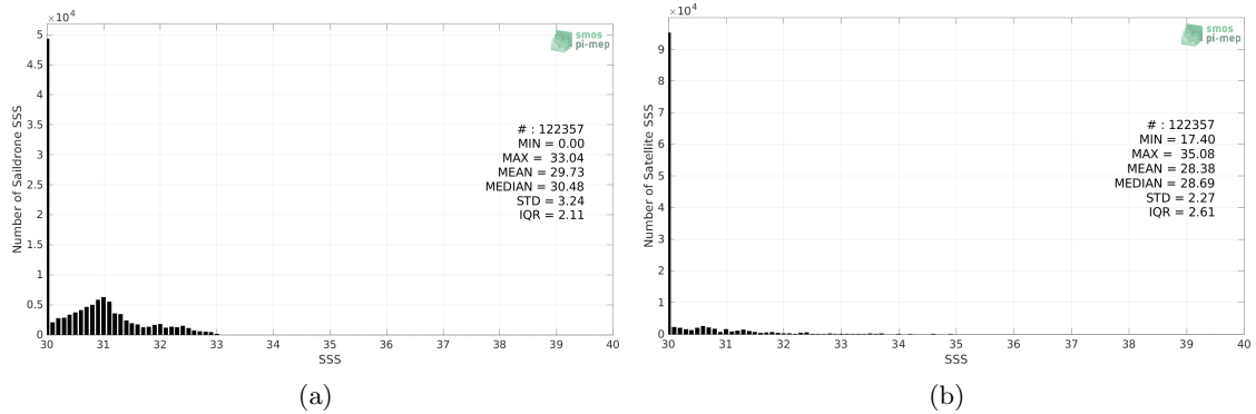
Figure 2: Histograms of SSS from Saildrone (a) and SMOS SSS L3 Arctic v1.1 - 7-Day running mean (CATDS-CECOS-LOCEAN) (b) considering all match-up pairs per bins of 0.1 over the Global Ocean Pi-MEP region and for the full satellite product period.
