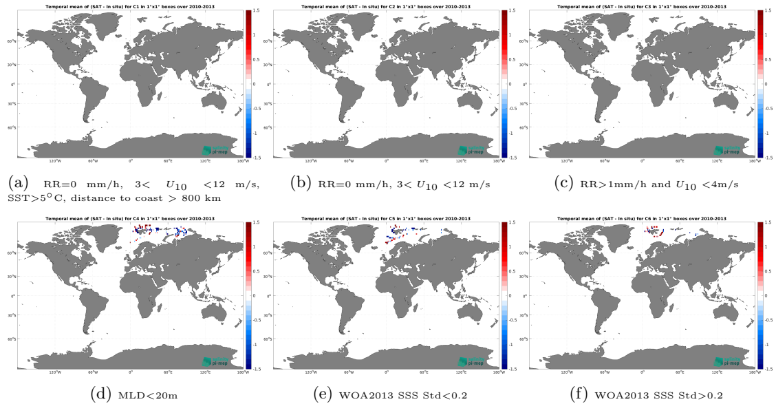
Figure 12: Temporal mean gridded over spatial boxes of size 1^{\circ}\times 1^{\circ} of \Delta\text{SSS} (SMOS SSS L3 Arctic v1.1 - 7-Day running mean (CATDS-CEC-LOCEAN) - Marine mammals) for 6 different subdatasets corresponding to:RR=0 mm/h, 3 < U_{10} < 12 m/s, SST > 5^{\circ}\text{C} , distance to coast > 800 km (a), RR=0 mm/h, 3 < U_{10} < 12 m/s (b), RR > 1\text{mm/h} and U_{10} < 4\text{m/s} (c),MLD < 20\text{m} (d),WOA2013 SSS Std < 0.2 (e),WOA2013 SSS Std > 0.2 (f).
