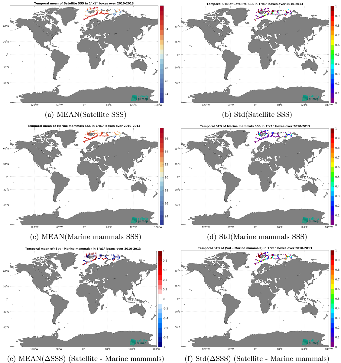
Figure 6: Temporal mean (left) and Std (right) of SSS from SMOS SSS L3 Arctic v1.1 - 7-Day running mean (CATDS-CEC-LOCEAN) (top), Marine mammals (middle), and of \Delta SSS (Satellite - Marine mammals). Only match-up pairs are used to generate these maps.
