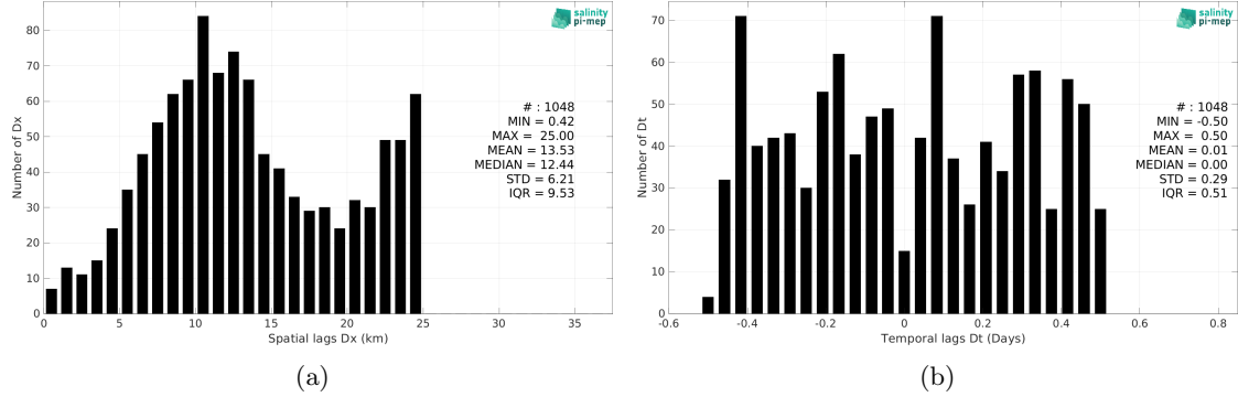
Figure 5: Histograms of the spatial (a) and temporal (b) lags between the location/time of the Marine mammals measurement and the date of the corresponding SMOS SSS L3 Arctic v1.1 - 7-Day running mean (CATDS-CEC-LOCEAN) SSS pixel.
