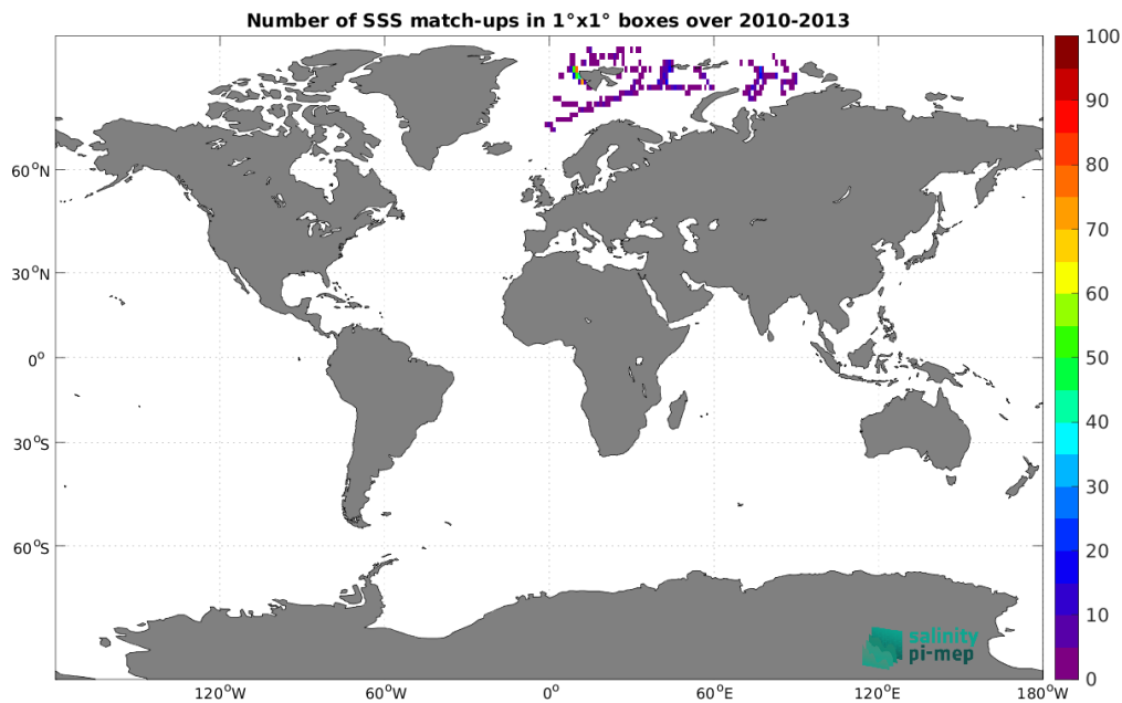
Figure 4: Number of SSS match-ups between Marine mammals SSS and the SMOS SSS L3 Arctic v1.1 - 7-Day running mean (CATDS-CEC-LOCEAN) SSS product for the Global Ocean Pi-MEP region over 1^\circ \times 1^\circ boxes and for the full satellite product period.
