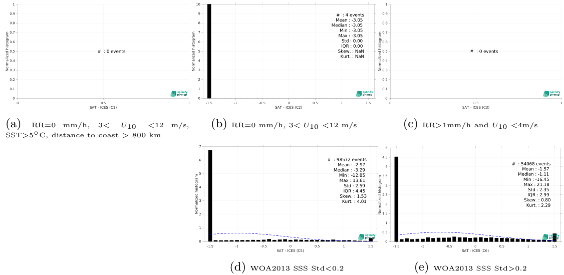
Figure 13: Normalized histogram of \Delta SSS (SMOS SSS L3 Arctic v1.1 - 7-Day runing mean (CATDS-CEC-LOCEAN) - ICES) for 5 different subdatasets corresponding to: RR=0 mm/h, 3 < U_{10} < 12 m/s, SST>5°C, distance to coast > 800 km (a), RR=0 mm/h, 3 < U_{10} < 12 m/s (b), RR>1mm/h and U_{10} < 4 m/s (c), WOA2013 SSS Std<0.2 (d), WOA2013 SSS Std>0.2 (e).
