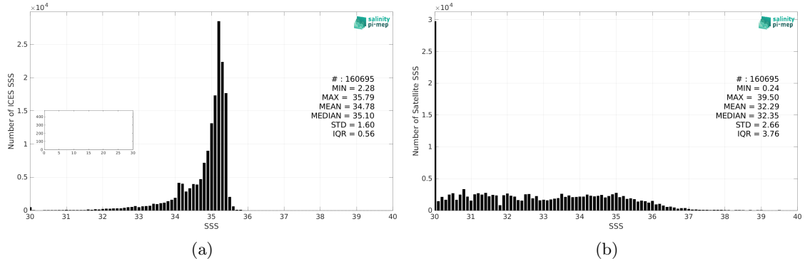
Figure 2: Histograms of SSS from ICES (a) and SMOS SSS L3 Arctic v1.1 - 7-Day running mean (CATDS-CEC-LOCEAN) (b) considering all match-up pairs per bins of 0.1 over the Global Ocean Pi-MEP region and for the full satellite product period.
