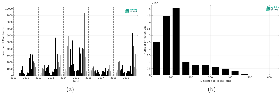
Figure 1: Number of match-ups between ICES and SMOS SSS L3 Arctic v1.1 - 7-Day running mean (CATDS-CEC-LOCEAN) SSS as a function of time (a) and as function of the distance to coast (b) over the Global Ocean Pi-MEP region and for the full satellite product period.
