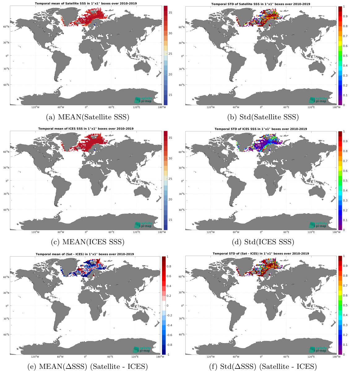
Figure 6: Temporal mean (left) and Std (right) of SSS from SMOS SSS L3 Arctic v1.1 - 7-Day running mean (CATDS-CEC-LOCEAN) (top), ICES (middle), and of \Delta SSS (Satellite - ICES). Only match-up pairs are used to generate these maps.
