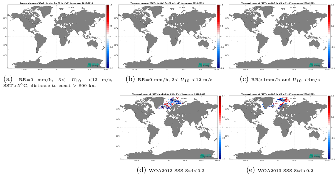
Figure 12: Temporal mean gridded over spatial boxes of size 1^{\circ}\times 1^{\circ} of \Delta\text{SSS} (SMOS SSS L3 Arctic v1.1 - 7-Day running mean (CATDS-CEC-LOCEAN) - ICES) for 5 different subdatasets corresponding to:RR=0 mm/h, 3 < U_{10} < 12 m/s, SST >5^{\circ}\text{C} , distance to coast > 800 km (a), RR=0 mm/h, 3 < U_{10} < 12 m/s (b), RR >1 mm/h and U_{10} < 4 m/s (c), WOA2013 SSS Std <0.2 (d), WOA2013 SSS Std >0.2 (e).
