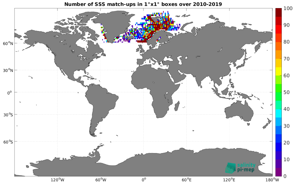
Figure 4: Number of SSS match-ups between ICES SSS and the SMOS SSS L3 Arctic v1.1 - 7-Day running mean (CATDS-CEC-LOCEAN) SSS product for the Global Ocean Pi-MEP region over 1^\circ \times 1^\circ boxes and for the full satellite product period.
