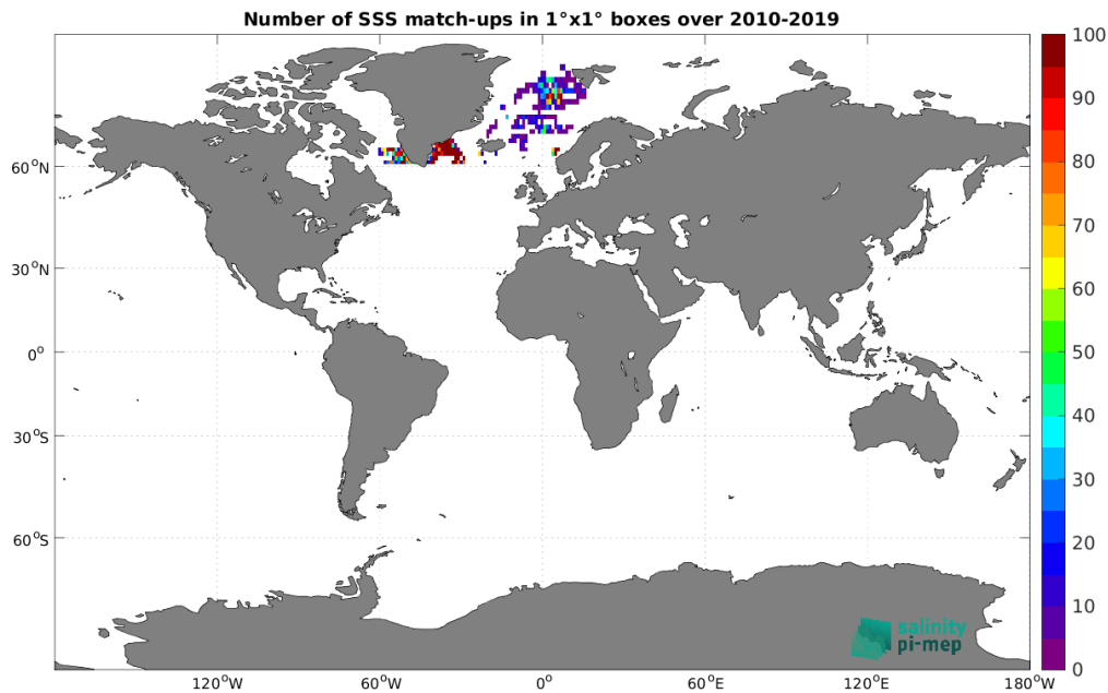
Figure 3: Number of SSS match-ups between Surface drifters SSS and the SMOS SSS L3 Arctic v1.1 - 7-Day running mean (CATDS-CEC-LOCEAN) SSS product for the Global Ocean Pi-MEP region over 1^\circ \times 1^\circ boxes and for the full satellite product period.
