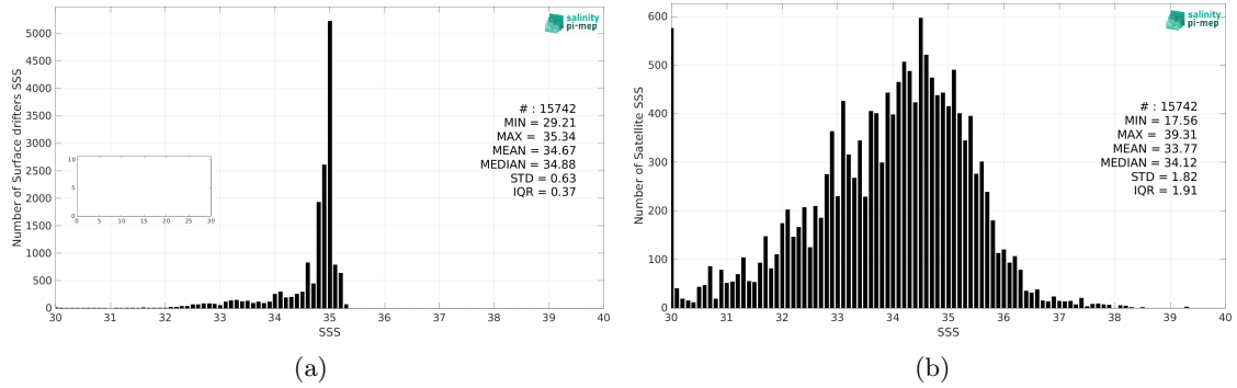
Figure 2: Histograms of SSS from Surface drifters (a) and SMOS SSS L3 Arctic v1.1 - 7-Day running mean (CATDS-CEC-LOCEAN) (b) considering all match-up pairs per bins of 0.1 over the Global Ocean Pi-MEP region and for the full satellite product period.
