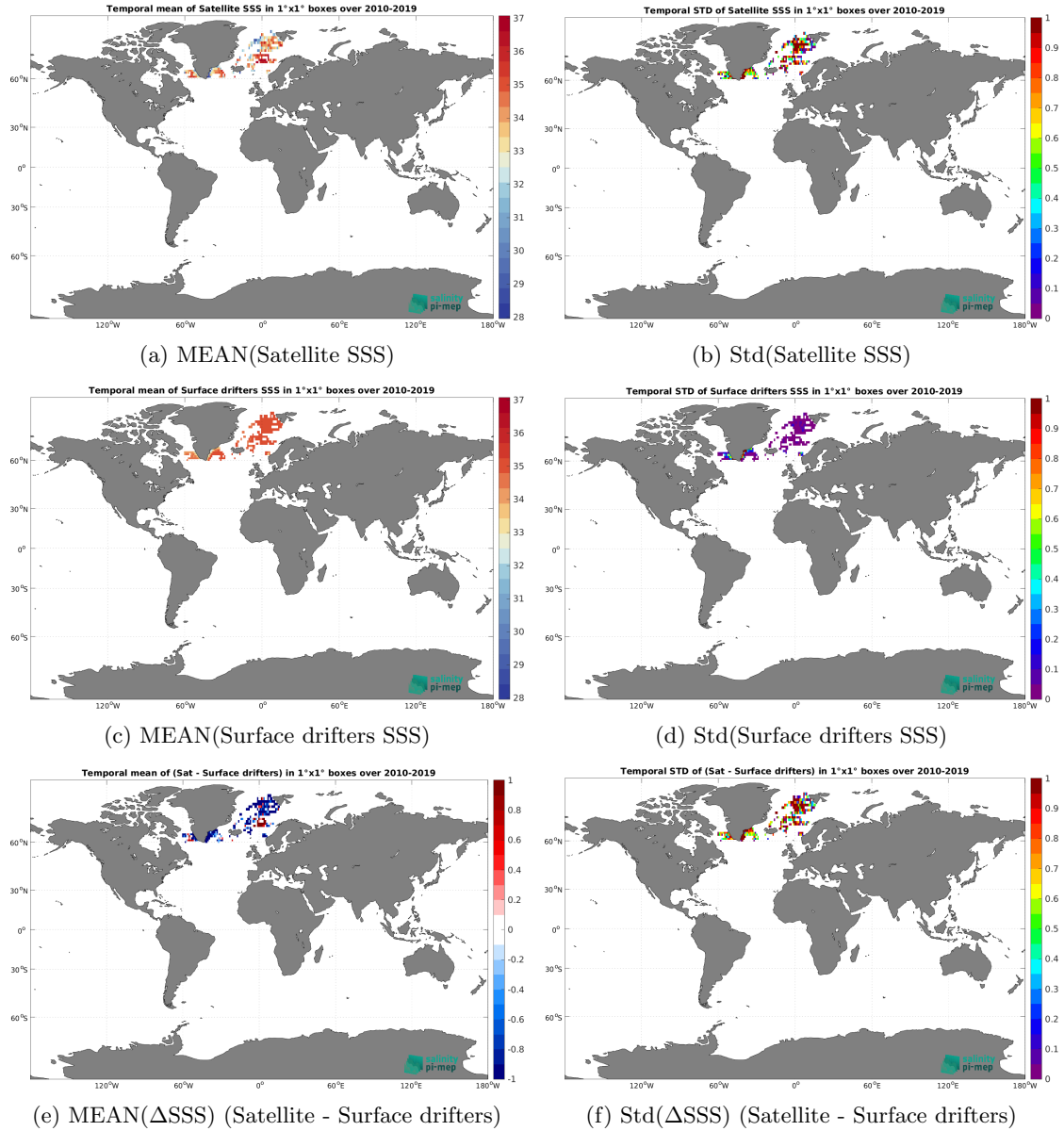
Figure 5: Temporal mean (left) and Std (right) of SSS from SMOS SSS L3 Arctic v1.1 - 7-Day running mean (CATDS-CEC-LOCEAN) (top), Surface drifters (middle), and of \Delta SSS (Satellite - Surface drifters). Only match-up pairs are used to generate these maps.
