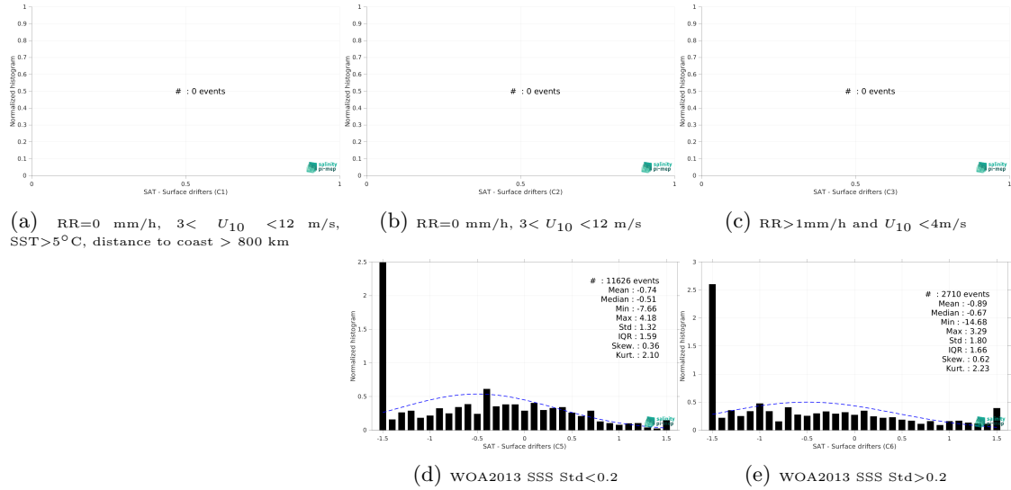
Figure 12: Normalized histogram of \Delta SSS (SMOS SSS L3 Arctic v1.1 - 7-Day runing mean (CATDS-CEC-LOCEAN) - Surface drifters) for 5 different subdatasets corresponding to: RR=0 mm/h, 3 < U_{10} < 12 m/s, SST>5°C, distance to coast > 800 km (a), RR=0 mm/h, 3 < U_{10} < 12 m/s (b), RR>1mm/h and U_{10} < 4 m/s (c), WOA2013 SSS Std<0.2 (d), WOA2013 SSS Std>0.2 (e).
