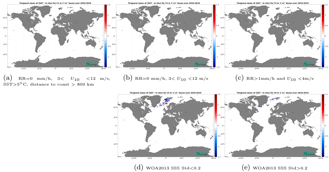
Figure 11: Temporal mean gridded over spatial boxes of size 1^{\circ}\times 1^{\circ} of \Delta\text{SSS} (SMOS SSS L3 Arctic v1.1 - 7-Day running mean (CATDS-CEC-LOCEAN) - Surface drifters) for 5 different subdatasets corresponding to:RR=0 mm/h, 3 < U_{10} < 12 m/s, SST >5^{\circ}\text{C} , distance to coast > 800 km (a), RR=0 mm/h, 3 < U_{10} < 12 m/s (b), RR >1 mm/h and U_{10} < 4 m/s (c), WOA2013 SSS Std <0.2 (d), WOA2013 SSS Std >0.2 (e).
