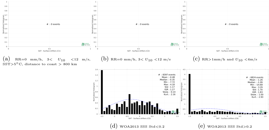
Figure 12: Normalized histogram of \Delta SSS (SMOS SSS L3 Arctic v1.1 - 7-Day running mean (CATDS-CECOS-LOCEAN) - Surface drifters) for 5 different subdatasets corresponding to: RR=0 mm/h, 3 < U_{10} < 12 m/s, SST > 5°C, distance to coast > 800 km (a), RR=0 mm/h, 3 < U_{10} < 12 m/s (b), RR > 1mm/h and U_{10} < 4 m/s (c), WOA2013 SSS Std < 0.2 (d), WOA2013 SSS Std > 0.2 (e).
