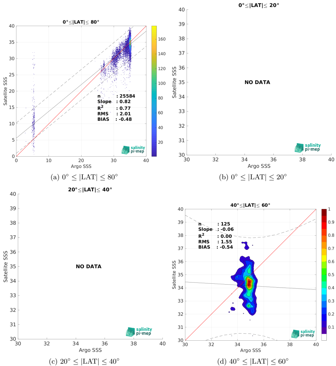
Figure 9: Contour maps of the concentration of SMOS SSS L3 Arctic v1.1 - 7-Day runing mean (CATDS-CEC-LOCEAN) SSS (y-axis) versus Argo SSS (x-axis) at match-up pairs for different latitude bands. For each plot, the red line shows x=y . The black thin and dashed lines indicate a linear fit through the data cloud and the \pm 95\% confidence levels, respectively. The number match-up pairs n , the slope and R^2 coefficient of the linear fit, the root mean square (RMS) and the mean bias between satellite and in situ data are indicated for each latitude band in each plots.
