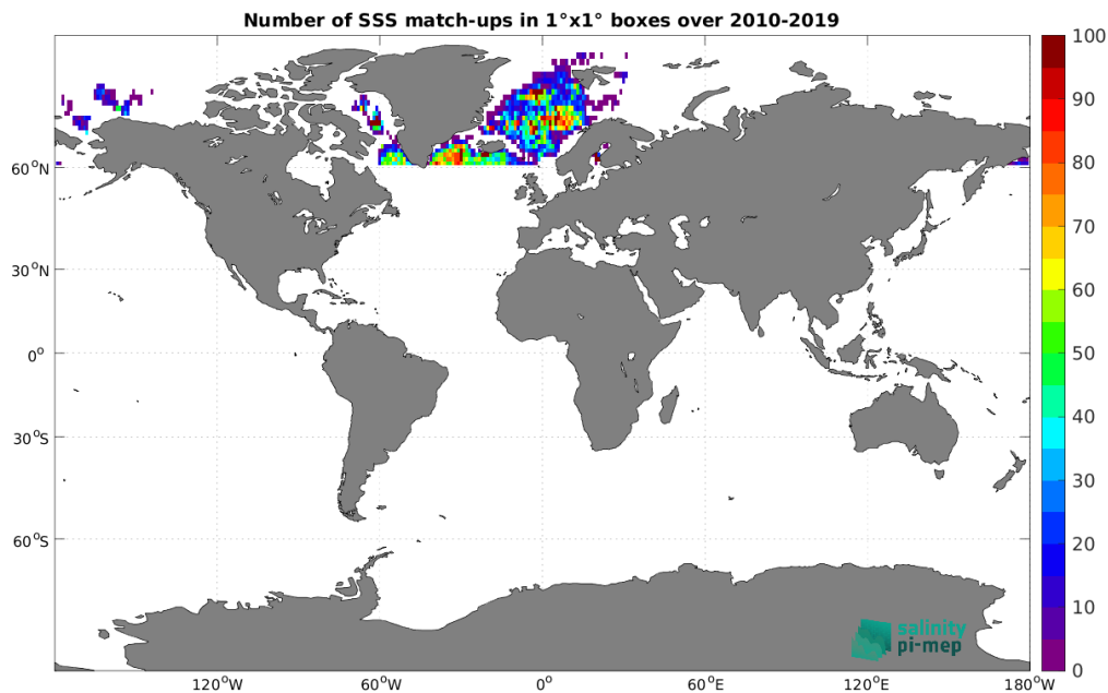
Figure 4: Number of SSS match-ups between Argo SSS and the SMOS SSS L3 Arctic v1.1 - 7-Day running mean (CATDS-CEC-LOCEAN) SSS product for the Global Ocean Pi-MEP region over 1^\circ \times 1^\circ boxes and for the full satellite product period.
