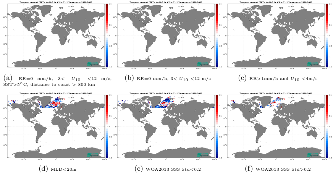
Figure 12: Temporal mean gridded over spatial boxes of size 1^{\circ}\times 1^{\circ} of \Delta\text{SSS} (SMOS SSS L3 Arctic v1.1 - 7-Day running mean (CATDS-CEC-LOCEAN) - Argo) for 6 different subdatasets corresponding to:RR=0 mm/h, 3 < U_{10} < 12 m/s, SST > 5^{\circ}\text{C} , distance to coast > 800 km (a), RR=0 mm/h, 3 < U_{10} < 12 m/s (b), RR > 1\text{mm/h} and U_{10} < 4\text{m/s} (c),MLD < 20\text{m} (d),WOA2013 SSS Std < 0.2 (e),WOA2013 SSS Std > 0.2 (f).
