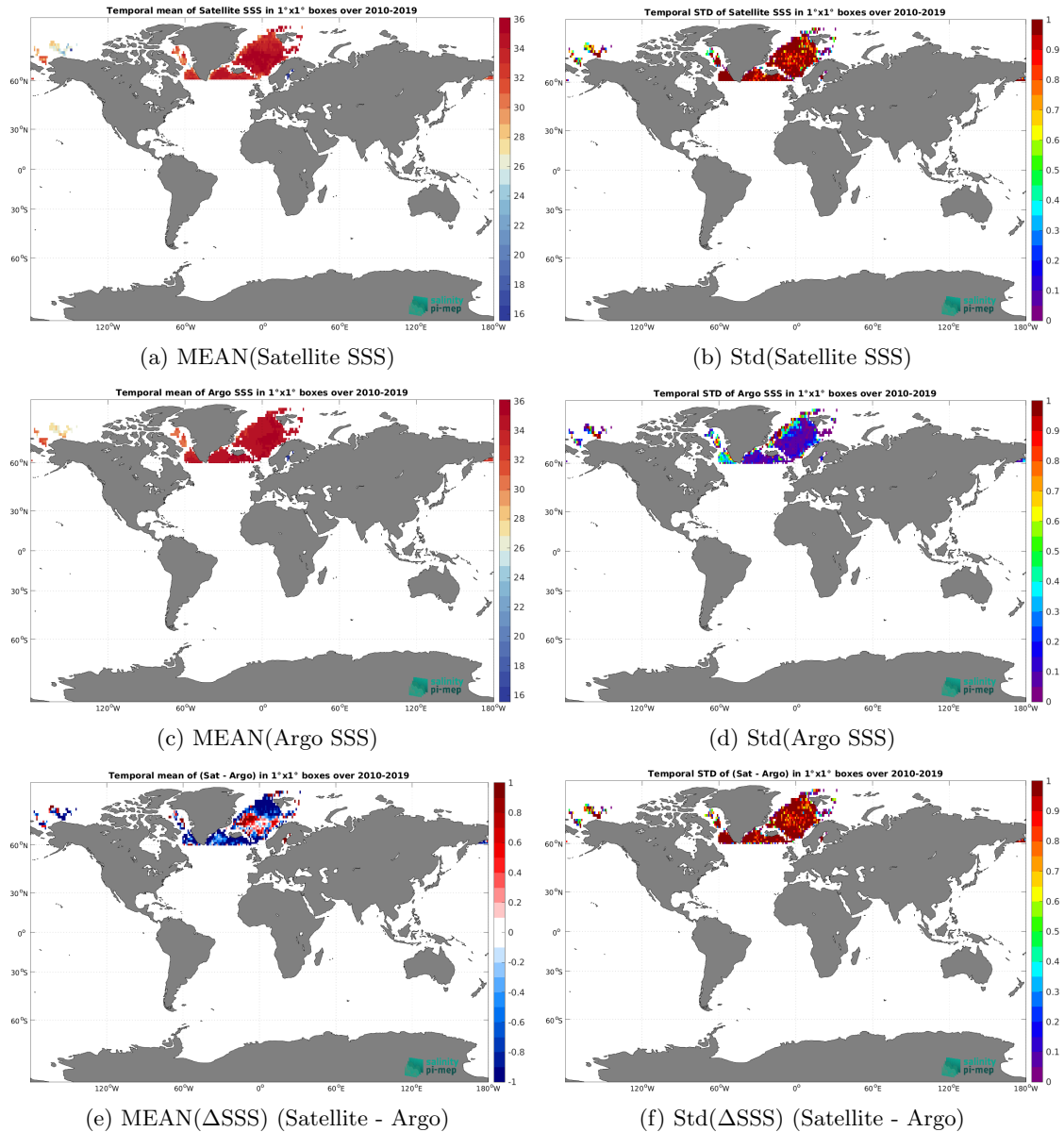
Figure 6: Temporal mean (left) and Std (right) of SSS from SMOS SSS L3 Arctic v1.1 - 7-Day running mean (CATDS-CEC-LOCEAN) (top), Argo (middle), and of \Delta SSS (Satellite - Argo). Only match-up pairs are used to generate these maps.
