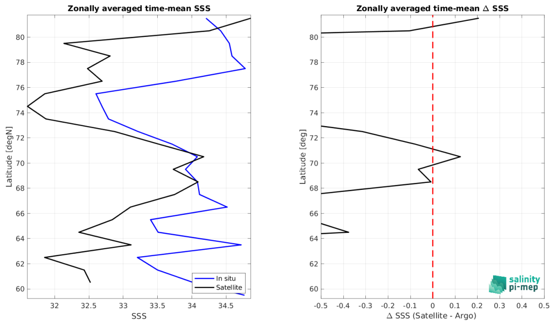
Figure 8: Left panel: Zonal mean SSS from SMOS SSS L3 Arctic v1.1 - 7-Day running mean (CATDS-CEC-LOCEAN) satellite product (black) and from Argo (blue). Right panel: Zonal mean of \Delta SSS (Satellite - Argo) for all the collected Pi-MEP match-up pairs estimated over the full satellite product period.
