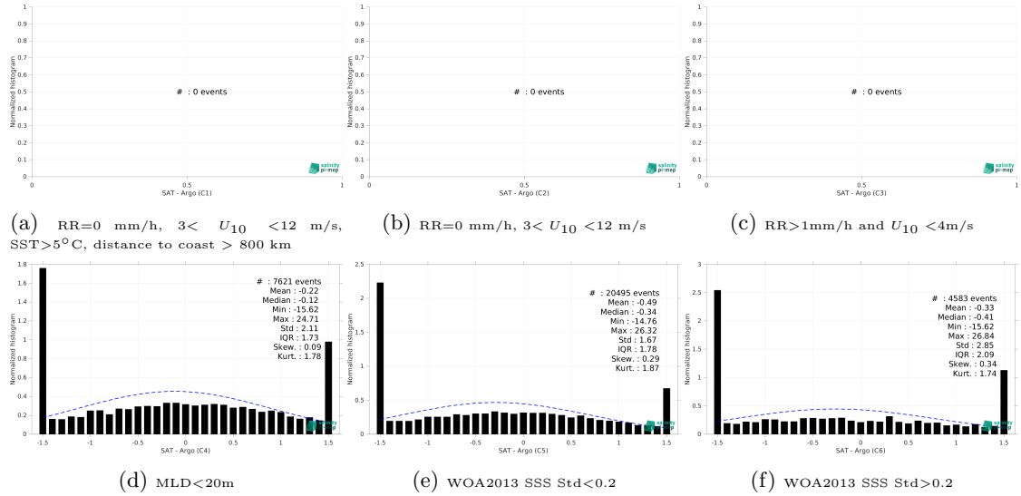
Figure 13: Normalized histogram of \Delta SSS (SMOS SSS L3 Arctic v1.1 - 7-Day runing mean (CATDS-CEC-LOCEAN) - Argo) for 6 different subdatasets corresponding to: RR=0 mm/h, 3 < U_{10} < 12 m/s, SST > 5°C, distance to coast > 800 km (a), RR=0 mm/h, 3 < U_{10} < 12 m/s (b), RR > 1mm/h and U_{10} < 4 m/s (c), MLD < 20m (d), WOA2013 SSS Std < 0.2 (e), WOA2013 SSS Std > 0.2 (f).
