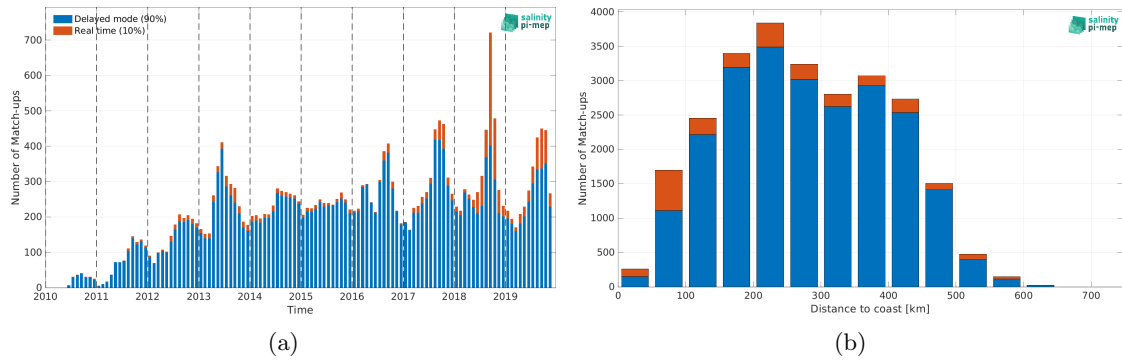
Figure 1: Number of match-ups between Argo and SMOS SSS L3 Arctic v1.1 - 7-Day running mean (CATDS-CEC-LOCEAN) SSS as a function of time (a) and as function of the distance to coast (b) over the Global Ocean Pi-MEP region and for the full satellite product period.
