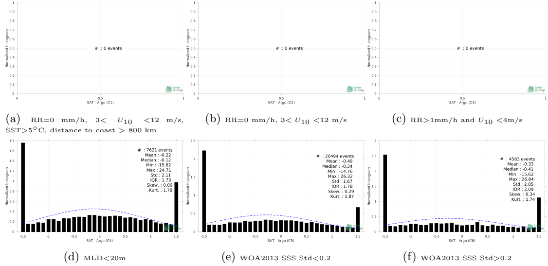
Figure 13: Normalized histogram of \Delta SSS (SMOS SSS L3 Arctic v1.1 - 7-Day running mean (CATDS-CECOS-LOCEAN) - Argo) for 6 different subdatasets corresponding to: RR=0 mm/h, 3 < U_{10} < 12 m/s, SST > 5°C, distance to coast > 800 km (a), RR=0 mm/h, 3 < U_{10} < 12 m/s (b), RR > 1mm/h and U_{10} < 4 m/s (c), MLD < 20m (d), WOA2013 SSS Std < 0.2 (e), WOA2013 SSS Std > 0.2 (f).
