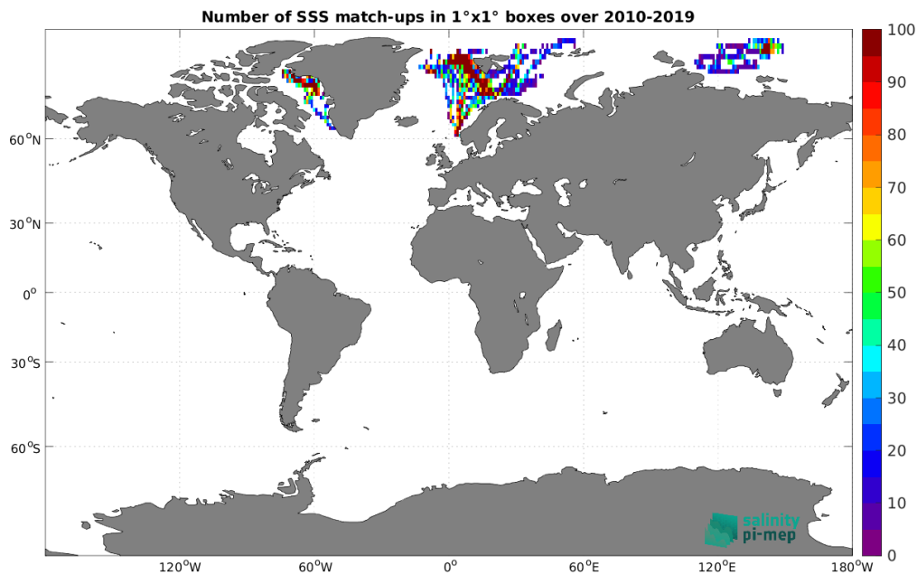
Figure 4: Number of SSS match-ups between TSG (Polarstern) SSS and the SMOS SSS L3 Arctic v1.1 - Monthly (CATDS-CECOS-LOCEAN) SSS product for the Global Ocean Pi-MEP region over 1^\circ \times 1^\circ boxes and for the full satellite product period.
