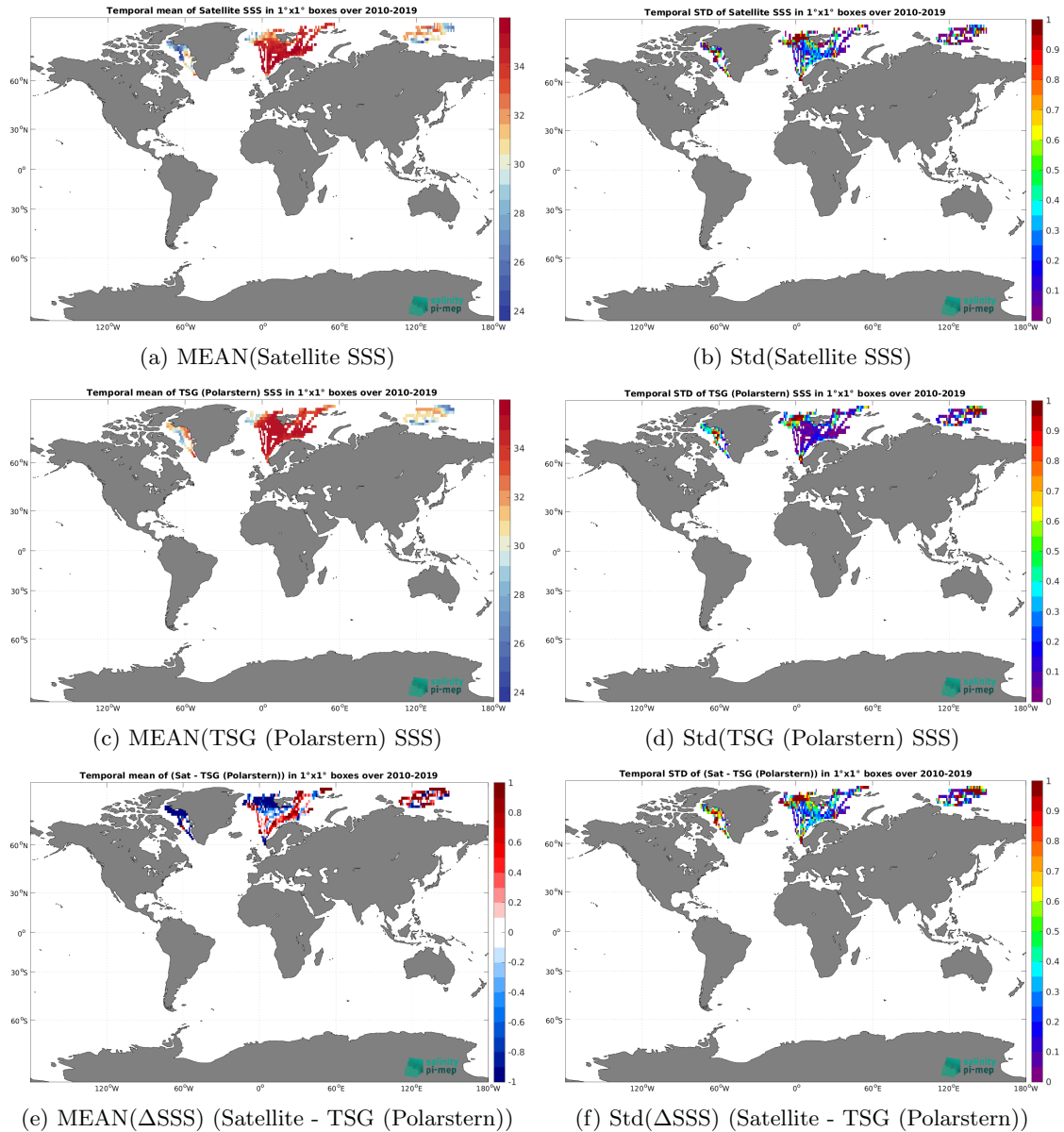
Figure 6: Temporal mean (left) and Std (right) of SSS from SMOS SSS L3 Arctic v1.1 - Monthly (CATDS-CECOS-LOCEAN) (top), TSG (Polarstern) (middle), and of \Delta SSS (Satellite - TSG (Polarstern)). Only match-up pairs are used to generate these maps.
