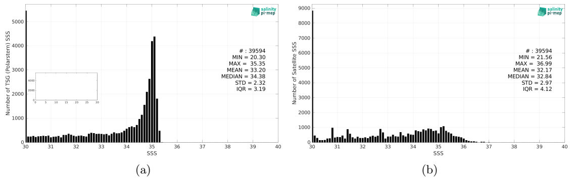
Figure 2: Histograms of SSS from TSG (Polarstern) (a) and SMOS SSS L3 Arctic v1.1 - Monthly (CATDS-CECOS-LOCEAN) (b) considering all match-up pairs per bins of 0.1 over the Global Ocean Pi-MEP region and for the full satellite product period.
