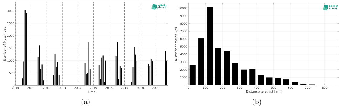
Figure 1: Number of match-ups between TSG (Polarstern) and SMOS SSS L3 Arctic v1.1 - Monthly (CATDS-CECOS-LOCEAN) SSS as a function of time (a) and as function of the distance to coast (b) over the Global Ocean Pi-MEP region and for the full satellite product period.
