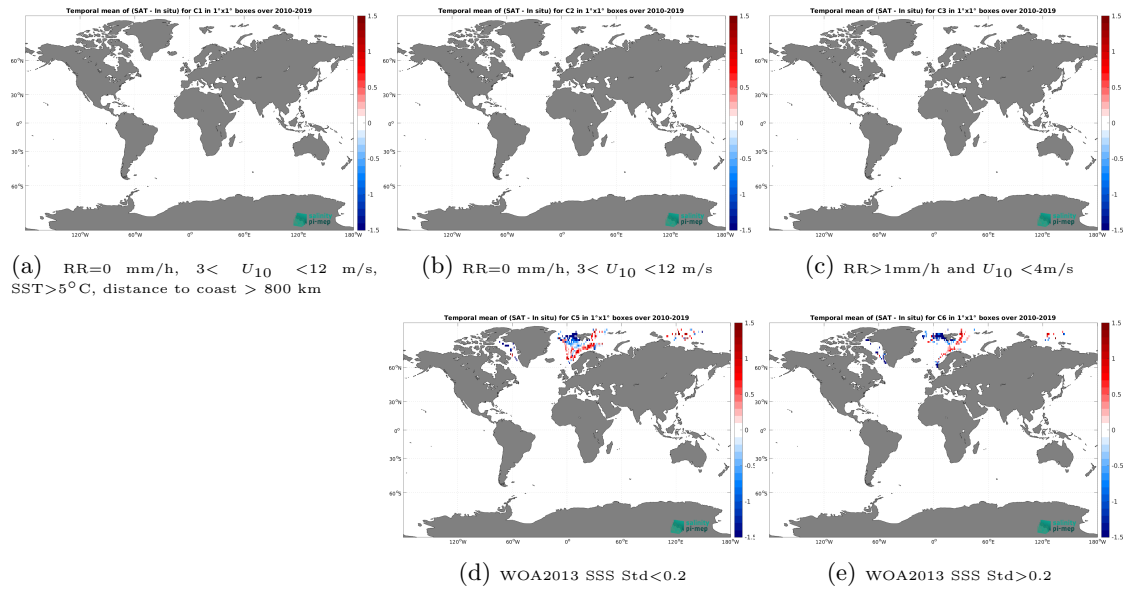
Figure 12: Temporal mean gridded over spatial boxes of size 1^{\circ}\times 1^{\circ} of \Delta\text{SSS} (SMOS SSS L3 Arctic v1.1 - Monthly (CATDS-CECOS-LOCEAN) - TSG (Polarstern)) for 5 different subdatasets corresponding to:RR=0 mm/h, 3 < U_{10} < 12 m/s, SST >5^{\circ}\text{C} , distance to coast > 800 km (a), RR=0 mm/h, 3 < U_{10} < 12 m/s (b), RR >1 mm/h and U_{10} < 4 m/s (c), WOA2013 SSS Std <0.2 (d), WOA2013 SSS Std >0.2 (e).
