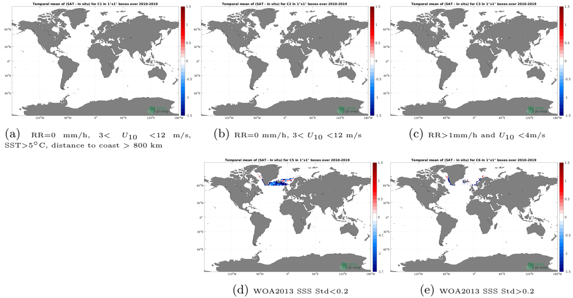
Figure 12: Temporal mean gridded over spatial boxes of size 1^{\circ}\times 1^{\circ} of \Delta\text{SSS} (SMOS SSS L3 Arctic v1.1 - Monthly (CATDS-CECOS-LOCEAN) - TSG (LEGOS-DM)) for 5 different subdatasets corresponding to:RR=0 mm/h, 3 < U_{10} < 12 m/s, SST >5^{\circ}\text{C} , distance to coast > 800 km (a), RR=0 mm/h, 3 < U_{10} < 12 m/s (b), RR >1 mm/h and U_{10} < 4 m/s (c), WOA2013 SSS Std <0.2 (d), WOA2013 SSS Std >0.2 (e).
