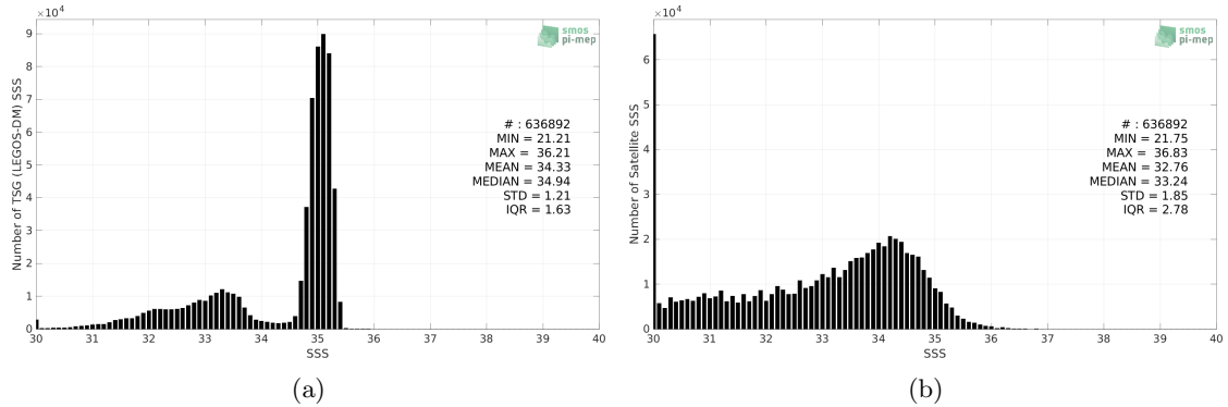
Figure 2: Histograms of SSS from TSG (LEGOS-DM) (a) and SMOS SSS L3 Arctic v1.1 - Monthly (CATDS-CECOS-LOCEAN) (b) considering all match-up pairs per bins of 0.1 over the Global Ocean Pi-MEP region and for the full satellite product period.
