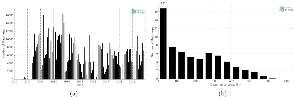
Figure 1: Number of match-ups between TSG (LEGOS-DM) and SMOS SSS L3 Arctic v1.1 - Monthly (CATDS-CECOS-LOCEAN) SSS as a function of time (a) and as function of the distance to coast (b) over the Global Ocean Pi-MEP region and for the full satellite product period.
