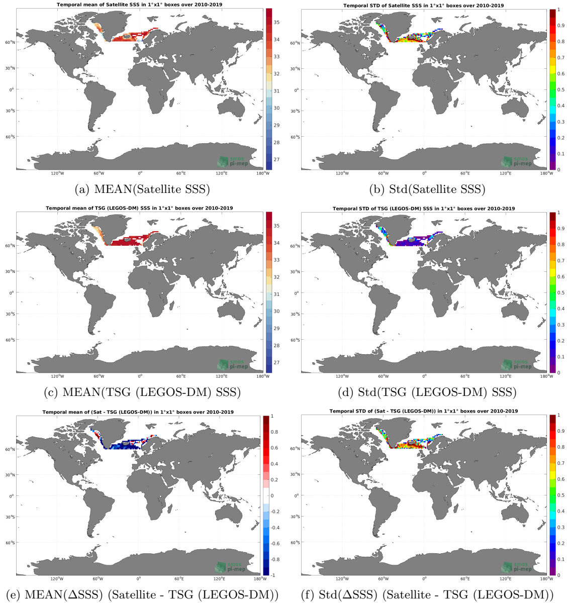
Figure 6: Temporal mean (left) and Std (right) of SSS from SMOS SSS L3 Arctic v1.1 - Monthly (CATDS-CECOS-LOCEAN) (top), TSG (LEGOS-DM) (middle), and of \Delta SSS (Satellite - TSG (LEGOS-DM)). Only match-up pairs are used to generate these maps.
