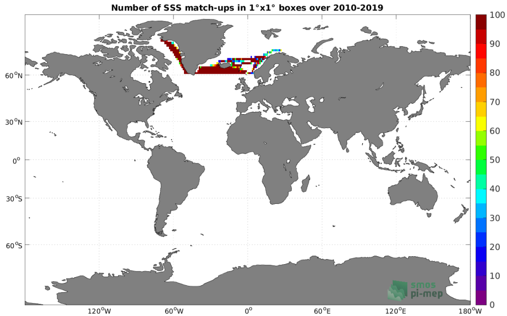
Figure 4: Number of SSS match-ups between TSG (LEGOS-DM) SSS and the SMOS SSS L3 Arctic v1.1 - Monthly (CATDS-CECOS-LOCEAN) SSS product for the Global Ocean Pi-MEP region over 1^\circ \times 1^\circ boxes and for the full satellite product period.
