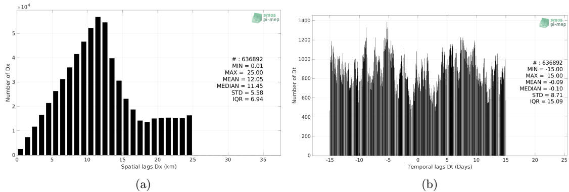
Figure 5: Histograms of the spatial (a) and temporal (b) lags between the location/time of the TSG (LEGOS-DM) measurement and the date of the corresponding SMOS SSS L3 Arctic v1.1 - Monthly (CATDS-CECOS-LOCEAN) SSS pixel.
