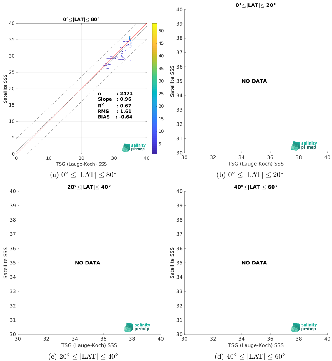
Figure 9: Contour maps of the concentration of SMOS SSS L3 Arctic v1.1 - Monthly (CATDS-CECOS-LOCEAN) SSS (y-axis) versus TSG (Lauge-Koch) SSS (x-axis) at match-up pairs for different latitude bands. For each plot, the red line shows x=y . The black thin and dashed lines indicate a linear fit through the data cloud and the \pm 95\% confidence levels, respectively. The number match-up pairs n , the slope and R^2 coefficient of the linear fit, the root mean square (RMS) and the mean bias between satellite and in situ data are indicated for each latitude band in each plots.
