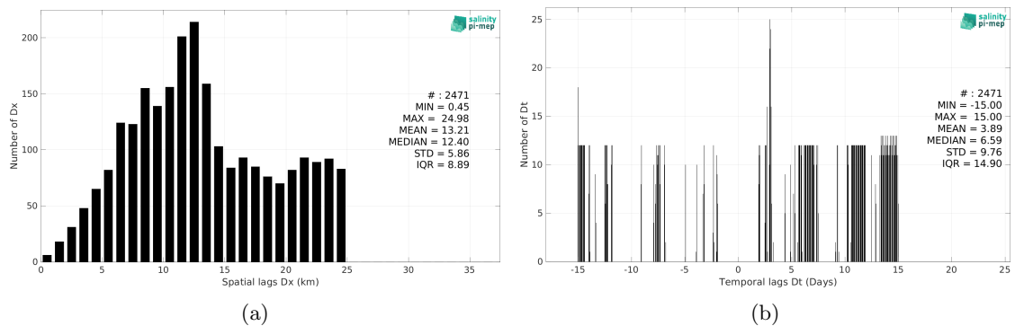
Figure 5: Histograms of the spatial (a) and temporal (b) lags between the location/time of the TSG (Lauge-Koch) measurement and the date of the corresponding SMOS SSS L3 Arctic v1.1 - Monthly (CATDS-CECOS-LOCEAN) SSS pixel.
