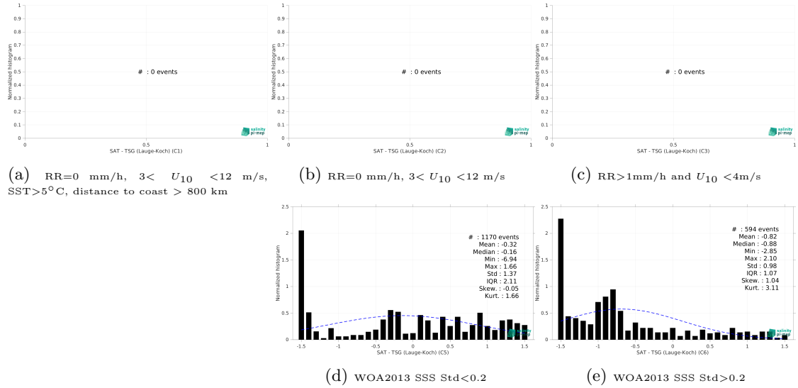
Figure 13: Normalized histogram of \Delta SSS (SMOS SSS L3 Arctic v1.1 - Monthly (CATDS-CECOS-LOCEAN) - TSG (Laue-Koch)) for 5 different subdatasets corresponding to: RR=0 mm/h, 3 < U_{10} < 12 m/s, SST > 5°C, distance to coast > 800 km (a), RR=0 mm/h, 3 < U_{10} < 12 m/s (b), RR > 1mm/h and U_{10} < 4 m/s (c), WOA2013 SSS Std < 0.2 (d), WOA2013 SSS Std > 0.2 (e).
