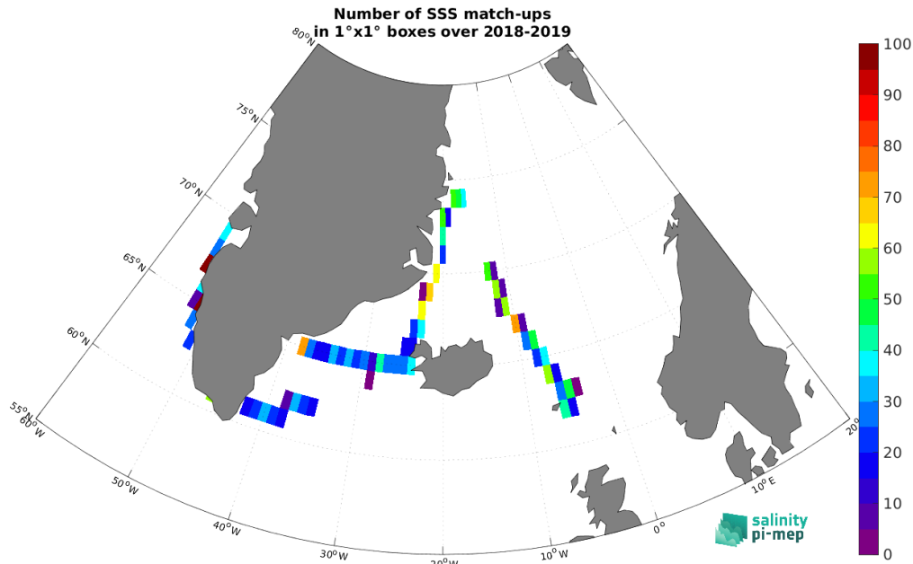
Figure 4: Number of SSS match-ups between TSG (Lauge-Koch) SSS and the SMOS SSS L3 Arctic v1.1 - Monthly (CATDS-CECOS-LOCEAN) SSS product for the Global Ocean Pi-MEP region over 1^\circ \times 1^\circ boxes and for the full satellite product period.
