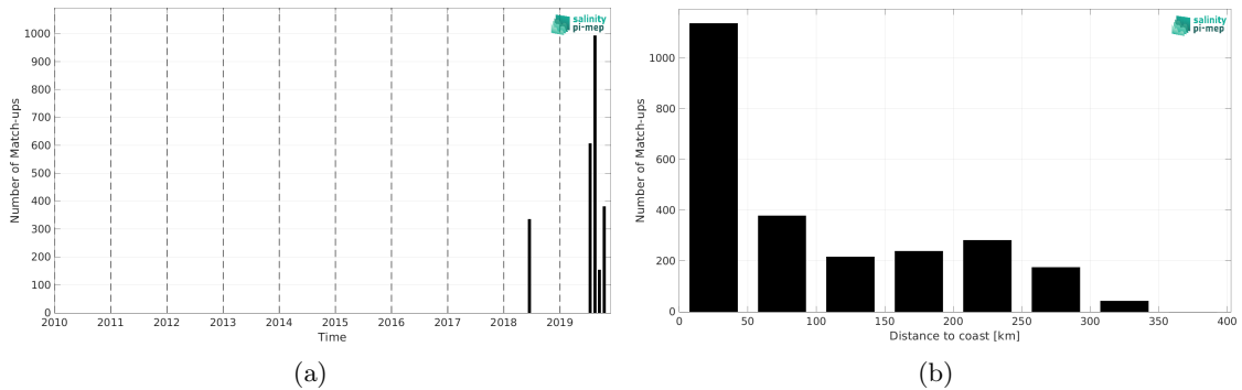
Figure 1: Number of match-ups between TSG (Lauge-Koch) and SMOS SSS L3 Arctic v1.1 - Monthly (CATDS-CECOS-LOCEAN) SSS as a function of time (a) and as function of the distance to coast (b) over the Global Ocean Pi-MEP region and for the full satellite product period.
