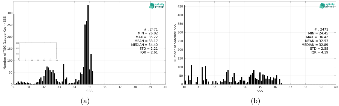
Figure 2: Histograms of SSS from TSG (Lauge-Koch) (a) and SMOS SSS L3 Arctic v1.1 - Monthly (CATDS-CECOS-LOCEAN) (b) considering all match-up pairs per bins of 0.1 over the Global Ocean Pi-MEP region and for the full satellite product period.
