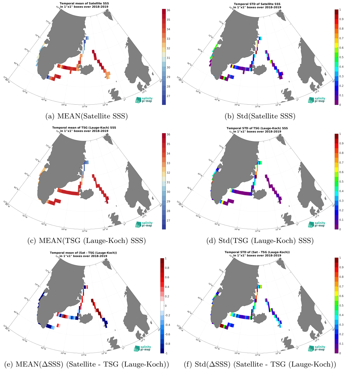
Figure 6: Temporal mean (left) and Std (right) of SSS from SMOS SSS L3 Arctic v1.1 - Monthly (CATDS-CECOS-LOCEAN) (top), TSG (Lauge-Koch) (middle), and of \Delta SSS (Satellite - TSG (Lauge-Koch)). Only match-up pairs are used to generate these maps.
