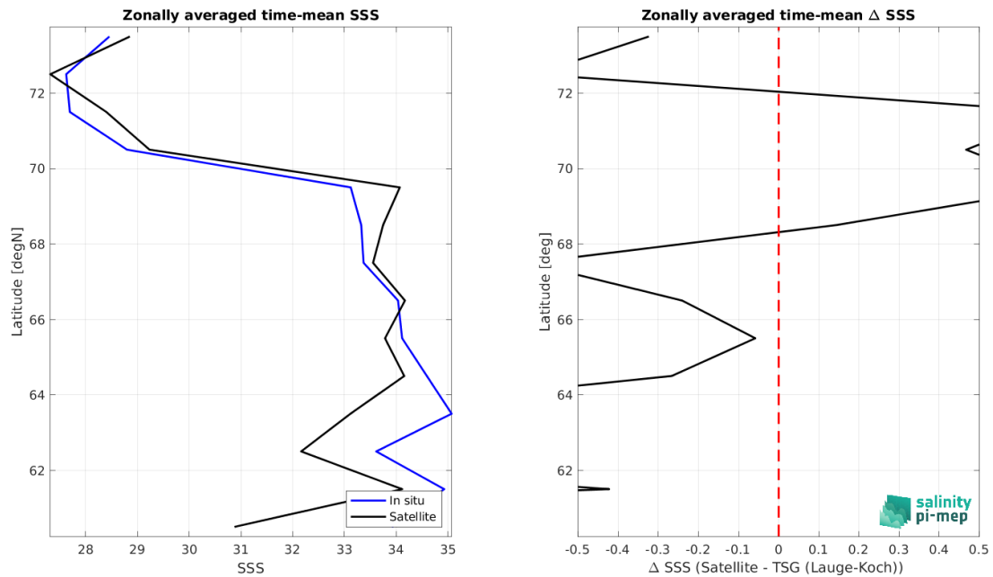
Figure 8: Left panel: Zonal mean SSS from SMOS SSS L3 Arctic v1.1 - Monthly (CATDS-CECOS-LOCEAN) satellite product (black) and from TSG (Lauge-Koch) (blue). Right panel: Zonal mean of \Delta SSS (Satellite - TSG (Lauge-Koch)) for all the collected Pi-MEP match-up pairs estimated over the full satellite product period.
