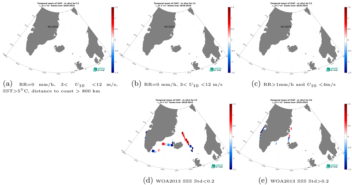
Figure 12: Temporal mean gridded over spatial boxes of size 1^{\circ}\times 1^{\circ} of \Delta\text{SSS} (SMOS SSS L3 Arctic v1.1 - Monthly (CATDS-CECOS-LOCEAN) - TSG (Lauge-Koch)) for 5 different subdatasets corresponding to:RR=0 mm/h, 3 < U_{10} < 12 m/s, SST >5^{\circ}\text{C} , distance to coast > 800 km (a), RR=0 mm/h, 3 < U_{10} < 12 m/s (b), RR >1 mm/h and U_{10} < 4 m/s (c), WOA2013 SSS Std <0.2 (d), WOA2013 SSS Std >0.2 (e).
