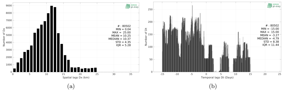
Figure 5: Histograms of the spatial (a) and temporal (b) lags between the location/time of the TSG (GOSUD-Sailing-ship) measurement and the date of the corresponding SMOS SSS L3 Arctic v1.1 - Monthly (CATDS-CECOS-LOCEAN) SSS pixel.
