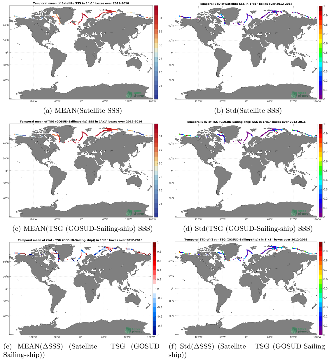
Figure 6: Temporal mean (left) and Std (right) of SSS from SMOS SSS L3 Arctic v1.1 - Monthly (CATDS-CECOS-LOCEAN) (top), TSG (GOSUD-Sailing-ship) (middle), and of \Delta SSS (Satellite - TSG (GOSUD-Sailing-ship)). Only match-up pairs are used to generate these maps.
