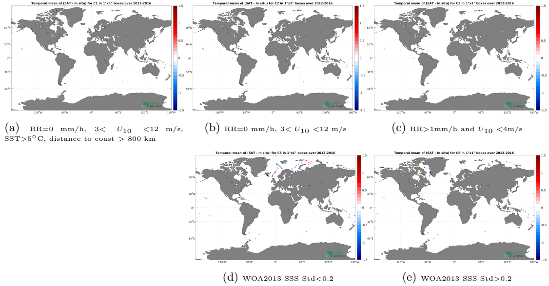
Figure 12: Temporal mean gridded over spatial boxes of size 1^{\circ}\times 1^{\circ} of \Delta SSS (SMOS SSS L3 Arctic v1.1 - Monthly (CATDS-CECOS-LOCEAN) - TSG (GOSUD-Sailing-ship)) for 5 different subdatasets corresponding to:RR=0 mm/h, 3 < U_{10} < 12 m/s, SST >5^{\circ}\text{C} , distance to coast > 800 km (a), RR=0 mm/h, 3 < U_{10} < 12 m/s (b), RR >1 mm/h and U_{10} < 4 m/s (c), WOA2013 SSS Std <0.2 (d), WOA2013 SSS Std >0.2 (e).
