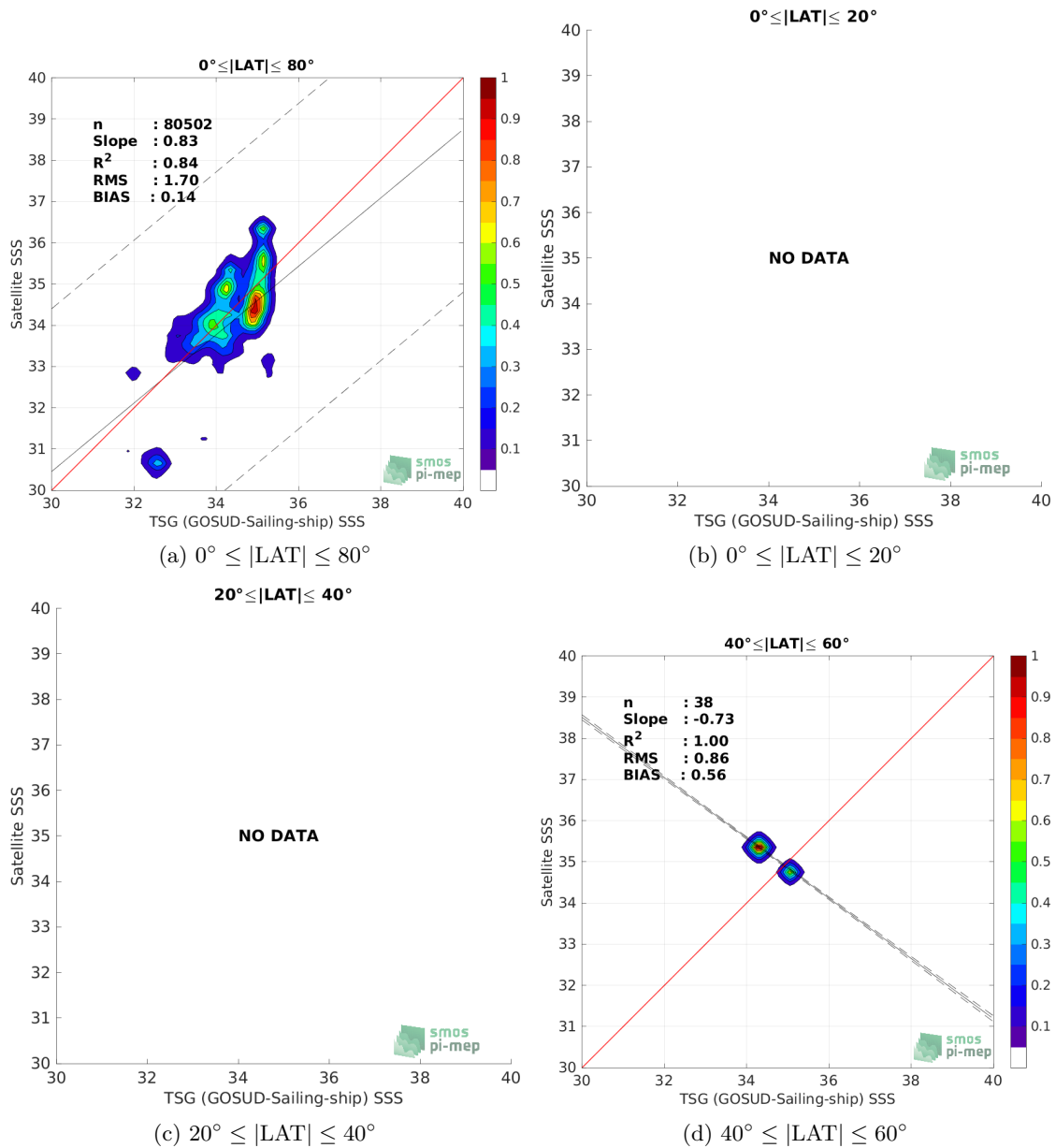
Figure 9: Contour maps of the concentration of SMOS SSS L3 Arctic v1.1 - Monthly (CATDS-CECOS-LOCEAN) SSS (y-axis) versus TSG (GOSUD-Sailing-ship) SSS (x-axis) at match-up pairs for different latitude bands. For each plot, the red line shows x=y . The black thin and dashed lines indicate a linear fit through the data cloud and the \pm 95\% confidence levels, respectively. The number match-up pairs n , the slope and R^2 coefficient of the linear fit, the root mean square (RMS) and the mean bias between satellite and in situ data are indicated for each latitude band in each plots.
