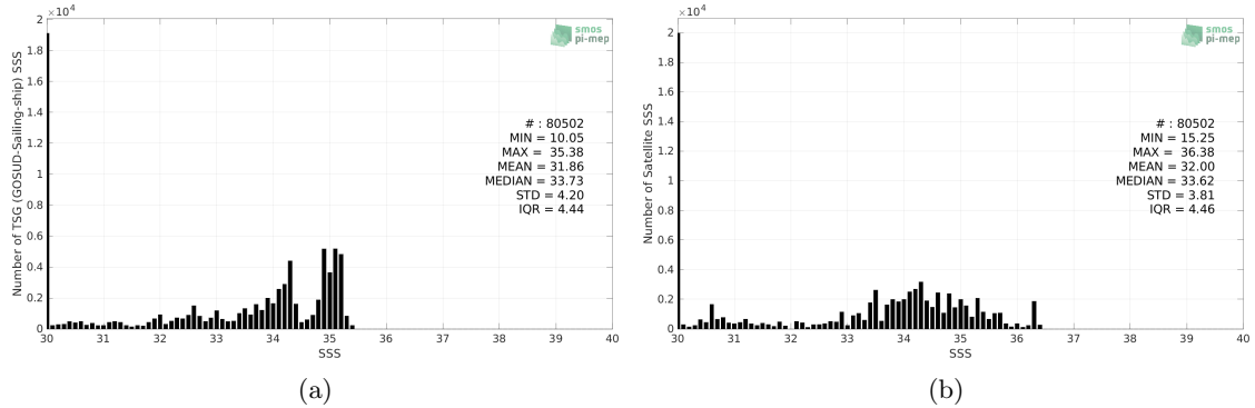
Figure 2: Histograms of SSS from TSG (GOSUD-Sailing-ship) (a) and SMOS SSS L3 Arctic v1.1 - Monthly (CATDS-CECOS-LOCEAN) (b) considering all match-up pairs per bins of 0.1 over the Global Ocean Pi-MEP region and for the full satellite product period.
