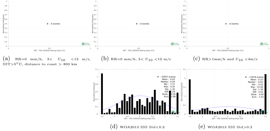
Figure 13: Normalized histogram of \Delta SSS (SMOS SSS L3 Arctic v1.1 - Monthly (CATDS-CECOS-LOCEAN) - TSG (GOSUD-Sailing-ship)) for 5 different subdatasets corresponding to: RR=0 mm/h, 3 < U_{10} < 12 m/s, SST > 5°C, distance to coast > 800 km (a), RR=0 mm/h, 3 < U_{10} < 12 m/s (b), RR > 1mm/h and U_{10} < 4 m/s (c), WOA2013 SSS Std < 0.2 (d), WOA2013 SSS Std > 0.2 (e).
