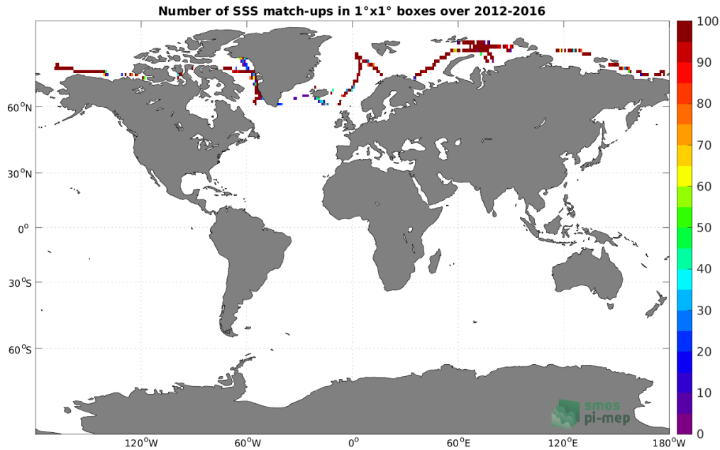
Figure 4: Number of SSS match-ups between TSG (GOSUD-Sailing-ship) SSS and the SMOS SSS L3 Arctic v1.1 - Monthly (CATDS-CECOS-LOCEAN) SSS product for the Global Ocean Pi-MEP region over 1^\circ \times 1^\circ boxes and for the full satellite product period.
