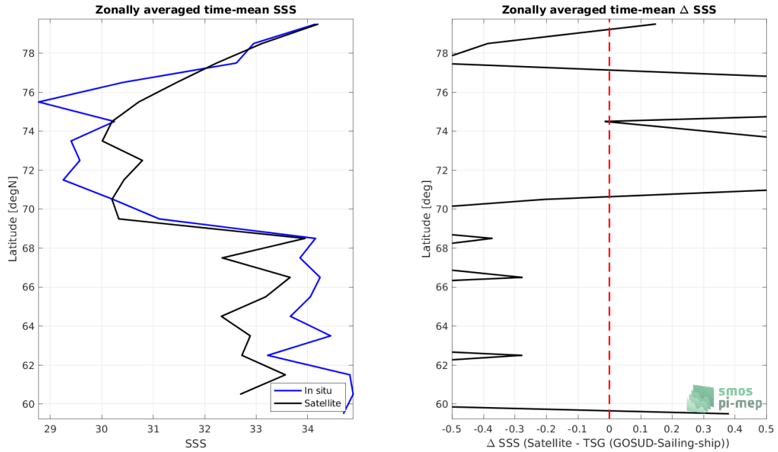
Figure 8: Left panel: Zonal mean SSS from SMOS SSS L3 Arctic v1.1 - Monthly (CATDS-CECOS-LOCEAN) satellite product (black) and from TSG (GOSUD-Sailing-ship) (blue). Right panel: Zonal mean of \Delta SSS (Satellite - TSG (GOSUD-Sailing-ship)) for all the collected Pi-MEP match-up pairs estimated over the full satellite product period.
