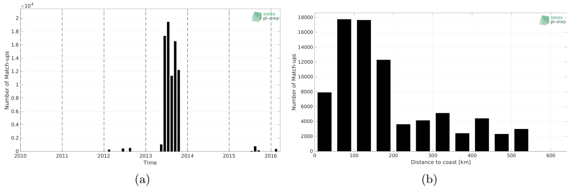
Figure 1: Number of match-ups between TSG (GOSUD-Sailing-ship) and SMOS SSS L3 Arctic v1.1 - Monthly (CATDS-CECOS-LOCEAN) SSS as a function of time (a) and as function of the distance to coast (b) over the Global Ocean Pi-MEP region and for the full satellite product period.
