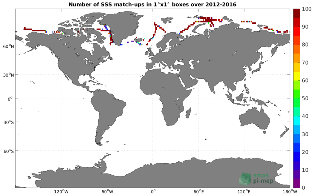
Figure 4: Number of SSS match-ups between TSG (GOSUD-Sailing-ship) SSS and the SMOS SSS L3 Arctic v1.1 - Monthly (CATDS-CECOS-LOCEAN) SSS product for the Global Ocean Pi-MEP region over 1°×1° boxes and for the full satellite product period.
