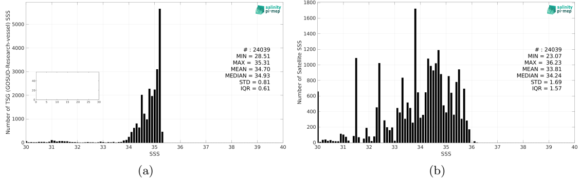
Figure 2: Histograms of SSS from TSG (GOSUD-Research-vessel) (a) and SMOS SSS L3 Arctic v1.1 - Monthly (CATDS-CECOS-LOCEAN) (b) considering all match-up pairs per bins of 0.1 over the Global Ocean Pi-MEP region and for the full satellite product period.
