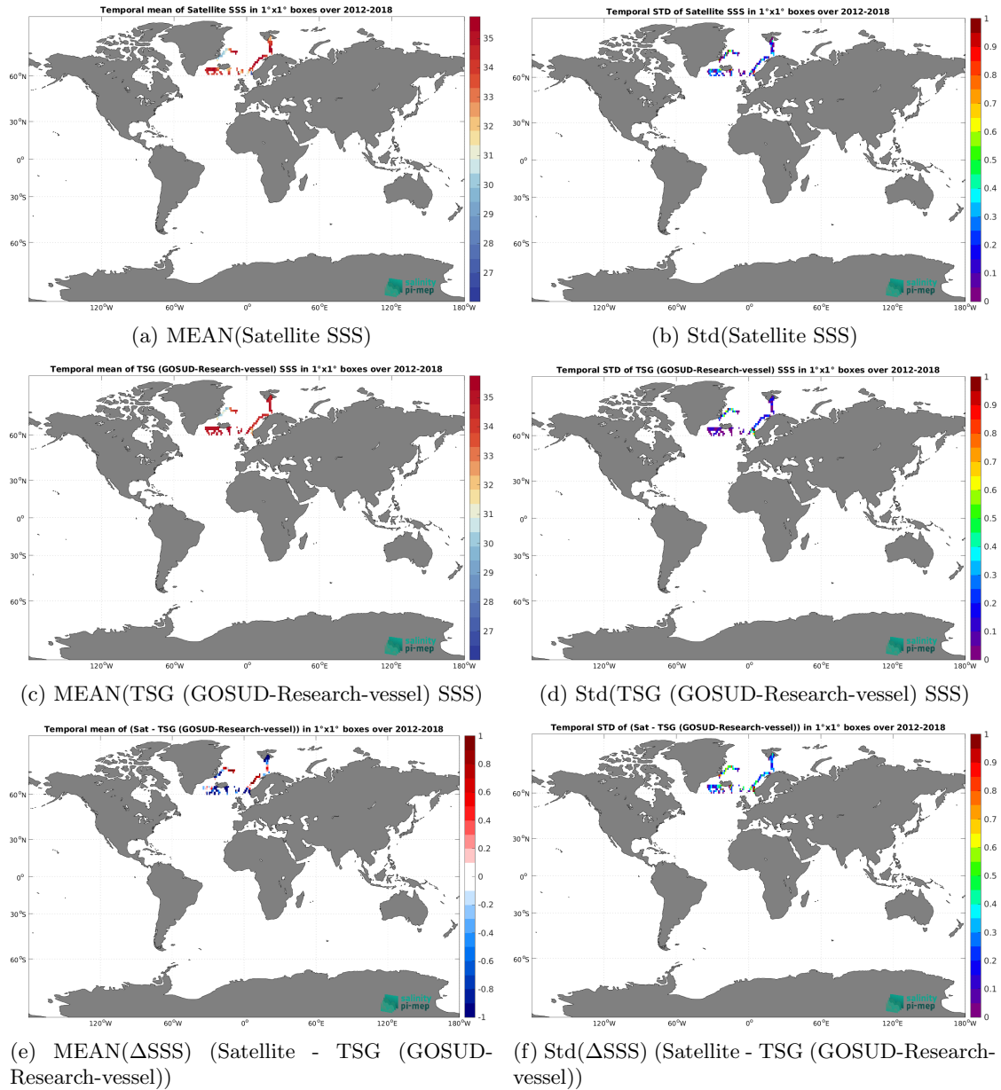
Figure 6: Temporal mean (left) and Std (right) of SSS from SMOS SSS L3 Arctic v1.1 - Monthly (CATDS-CECOS-LOCEAN) (top), TSG (GOSUD-Research-vessel) (middle), and of \Delta SSS (Satellite - TSG (GOSUD-Research-vessel)). Only match-up pairs are used to generate these maps.
