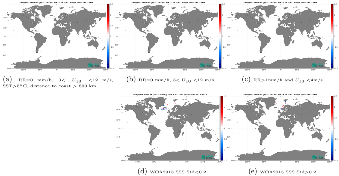
Figure 12: Temporal mean gridded over spatial boxes of size 1^{\circ}\times 1^{\circ} of \Delta SSS (SMOS SSS L3 Arctic v1.1 - Monthly (CATDS-CECOS-LOCEAN) - TSG (GOSUD-Research-vessel)) for 5 different subdatasets corresponding to:RR=0 mm/h, 3 < U_{10} < 12 m/s, SST >5^{\circ}\text{C} , distance to coast > 800 km (a), RR=0 mm/h, 3 < U_{10} < 12 m/s (b), RR >1 mm/h and U_{10} < 4 m/s (c), WOA2013 SSS Std <0.2 (d), WOA2013 SSS Std >0.2 (e).
