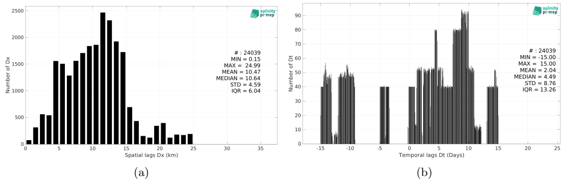
Figure 5: Histograms of the spatial (a) and temporal (b) lags between the location/time of the TSG (GOSUD-Research-vessel) measurement and the date of the corresponding SMOS SSS L3 Arctic v1.1 - Monthly (CATDS-CECOS-LOCEAN) SSS pixel.
