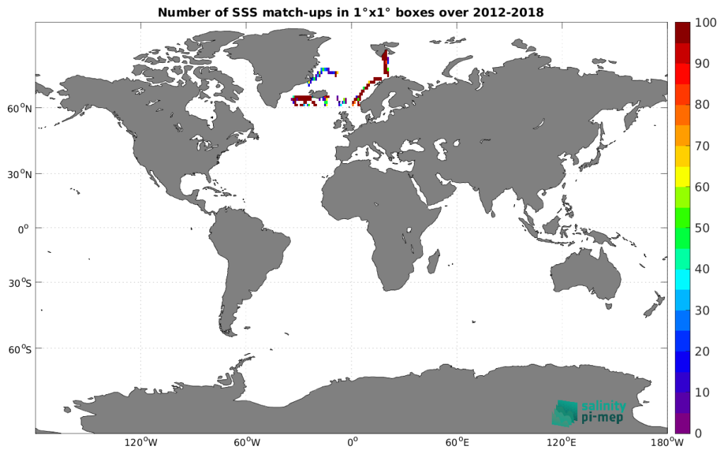
Figure 4: Number of SSS match-ups between TSG (GOSUD-Research-vessel) SSS and the SMOS SSS L3 Arctic v1.1 - Monthly (CATDS-CECOS-LOCEAN) SSS product for the Global Ocean Pi-MEP region over 1^{\circ} \times 1^{\circ} boxes and for the full satellite product period.
