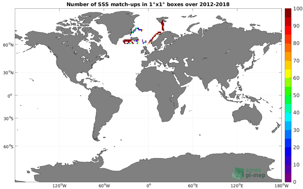
Figure 4: Number of SSS match-ups between TSG (GOSUD-Research-vessel) SSS and the SMOS SSS L3 Arctic v1.1 - Monthly (CATDS-CECOS-LOCEAN) SSS product for the Global Ocean Pi-MEP region over 1^\circ \times 1^\circ boxes and for the full satellite product period.
