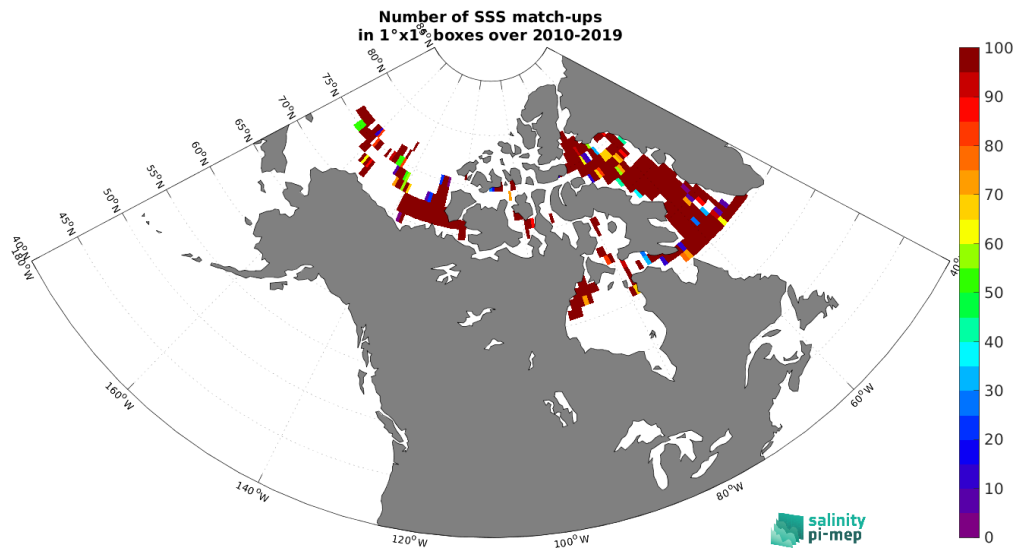
Figure 4: Number of SSS match-ups between TSG (Amundsen) SSS and the SMOS SSS L3 Arctic v1.1 - Monthly (CATDS-CECOS-LOCEAN) SSS product for the Global Ocean Pi-MEP region over 1°×1° boxes and for the full satellite product period.
