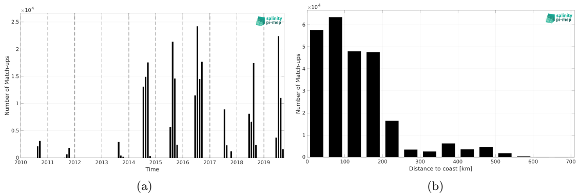
Figure 1: Number of match-ups between TSG (Amundsen) and SMOS SSS L3 Arctic v1.1 - Monthly (CATDS-CECOS-LOCEAN) SSS as a function of time (a) and as function of the distance to coast (b) over the Global Ocean Pi-MEP region and for the full satellite product period.
