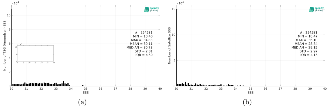
Figure 2: Histograms of SSS from TSG (Amundsen) (a) and SMOS SSS L3 Arctic v1.1 - Monthly (CATDS-CECOS-LOCEAN) (b) considering all match-up pairs per bins of 0.1 over the Global Ocean Pi-MEP region and for the full satellite product period.
