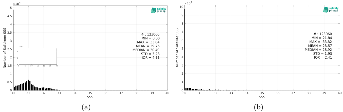
Figure 2: Histograms of SSS from Saildrone (a) and SMOS SSS L3 Arctic v1.1 - Monthly (CATDS-CECOS-LOCEAN) (b) considering all match-up pairs per bins of 0.1 over the Global Ocean Pi-MEP region and for the full satellite product period.
