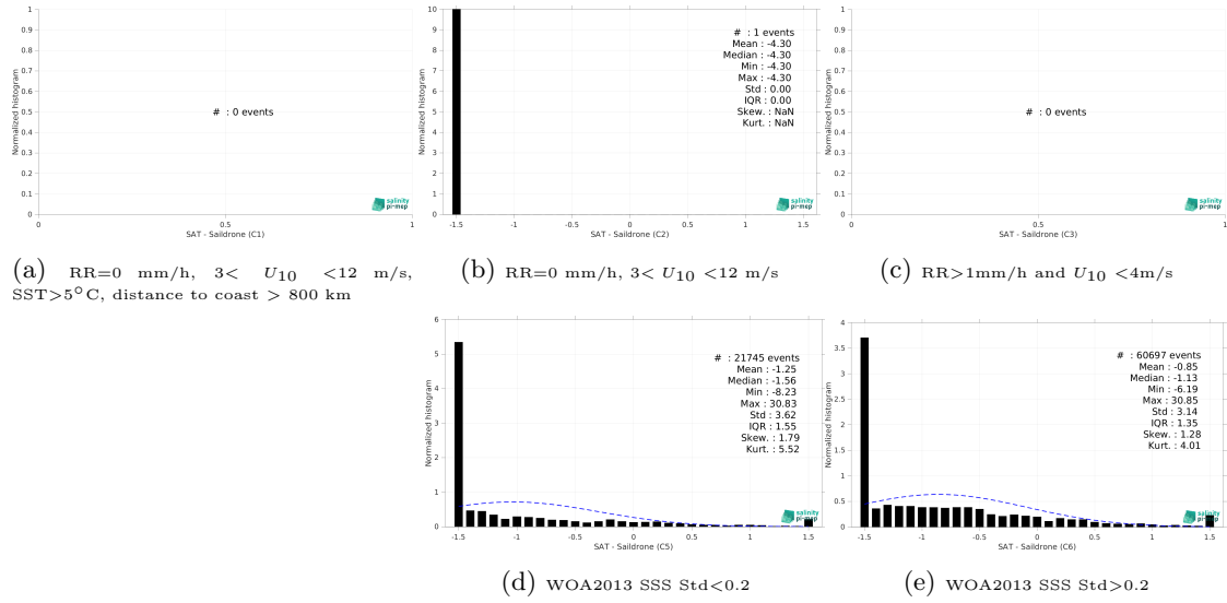
Figure 13: Normalized histogram of \Delta SSS (SMOS SSS L3 Arctic v1.1 - Monthly (CATDS-CECOS-LOCEAN) - Sairdrone) for 5 different subdatasets corresponding to: RR=0 mm/h, 3 < U_{10} < 12 m/s, SST>5°C, distance to coast > 800 km (a), RR=0 mm/h, 3 < U_{10} < 12 m/s (b), RR>1mm/h and U_{10} < 4 m/s (c), WOA2013 SSS Std<0.2 (d), WOA2013 SSS Std>0.2 (e).
