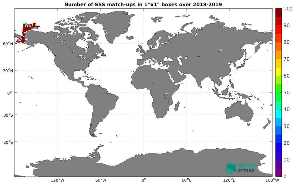
Figure 4: Number of SSS match-ups between Saildrone SSS and the SMOS SSS L3 Arctic v1.1 - Monthly (CATDS-CECOS-LOCEAN) SSS product for the Global Ocean Pi-MEP region over 1^\circ \times 1^\circ boxes and for the full satellite product period.
