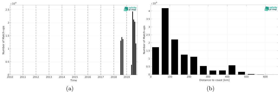
Figure 1: Number of match-ups between Saildrone and SMOS SSS L3 Arctic v1.1 - Monthly (CATDS-CECOS-LOCEAN) SSS as a function of time (a) and as function of the distance to coast (b) over the Global Ocean Pi-MEP region and for the full satellite product period.
