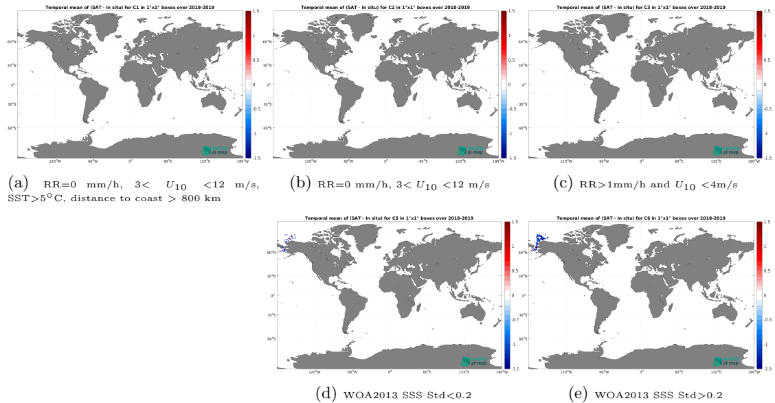
Figure 12: Temporal mean gridded over spatial boxes of size 1^{\circ}\times 1^{\circ} of \Delta\text{SSS} (SMOS SSS L3 Arctic v1.1 - Monthly (CATDS-CECOS-LOCEAN) - Saildrone) for 5 different subdatasets corresponding to:RR=0 mm/h, 3 < U_{10} < 12 m/s, SST >5^{\circ}\text{C} , distance to coast > 800 km (a), RR=0 mm/h, 3 < U_{10} < 12 m/s (b), RR >1 mm/h and U_{10} < 4 m/s (c), WOA2013 SSS Std <0.2 (d), WOA2013 SSS Std >0.2 (e).
