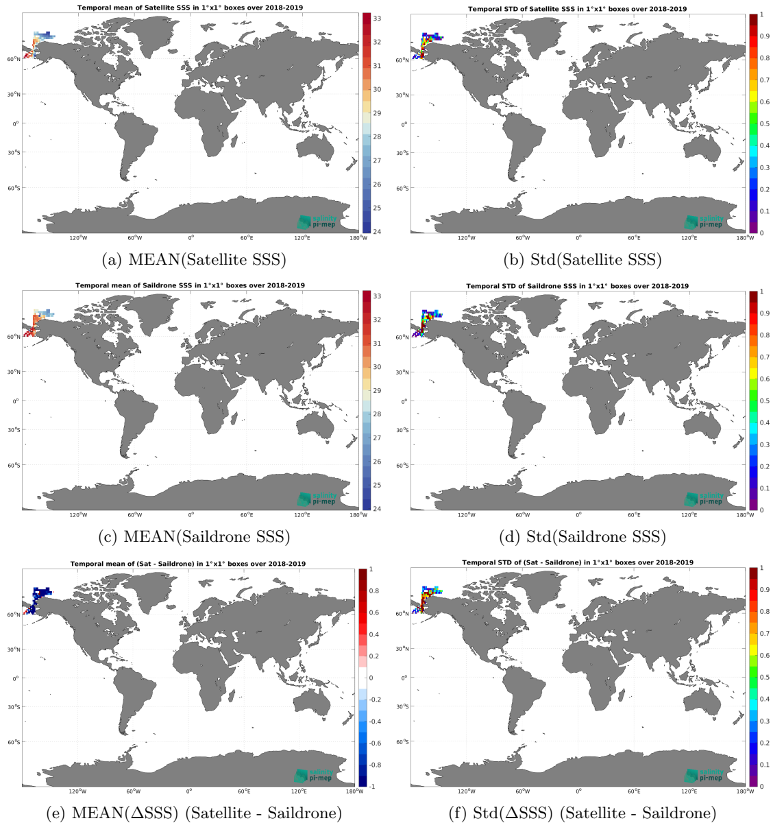
Figure 6: Temporal mean (left) and Std (right) of SSS from SMOS SSS L3 Arctic v1.1 - Monthly (CATDS-CECOS-LOCEAN) (top), Saildrone (middle), and of \Delta SSS (Satellite - Saildrone). Only match-up pairs are used to generate these maps.
