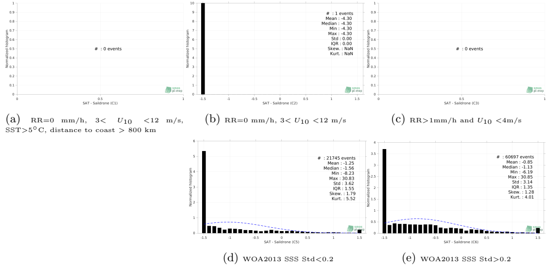
Figure 13: Normalized histogram of \Delta SSS (SMOS SSS L3 Arctic v1.1 - Monthly (CATDS-CECOS-LOCEAN) - Sairdrone) for 5 different subdatasets corresponding to: RR=0 mm/h, 3 < U_{10} < 12 m/s, SST > 5°C, distance to coast > 800 km (a), RR=0 mm/h, 3 < U_{10} < 12 m/s (b), RR > 1mm/h and U_{10} < 4 m/s (c), WOA2013 SSS Std < 0.2 (d), WOA2013 SSS Std > 0.2 (e).
