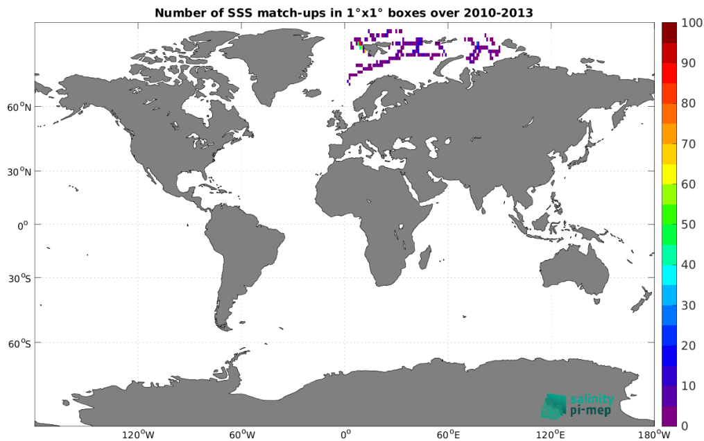
Figure 4: Number of SSS match-ups between Marine mammals SSS and the SMOS SSS L3 Arctic v1.1 - Monthly (CATDS-CECOS-LOCEAN) SSS product for the Global Ocean Pi-MEP region over 1^\circ \times 1^\circ boxes and for the full satellite product period.
