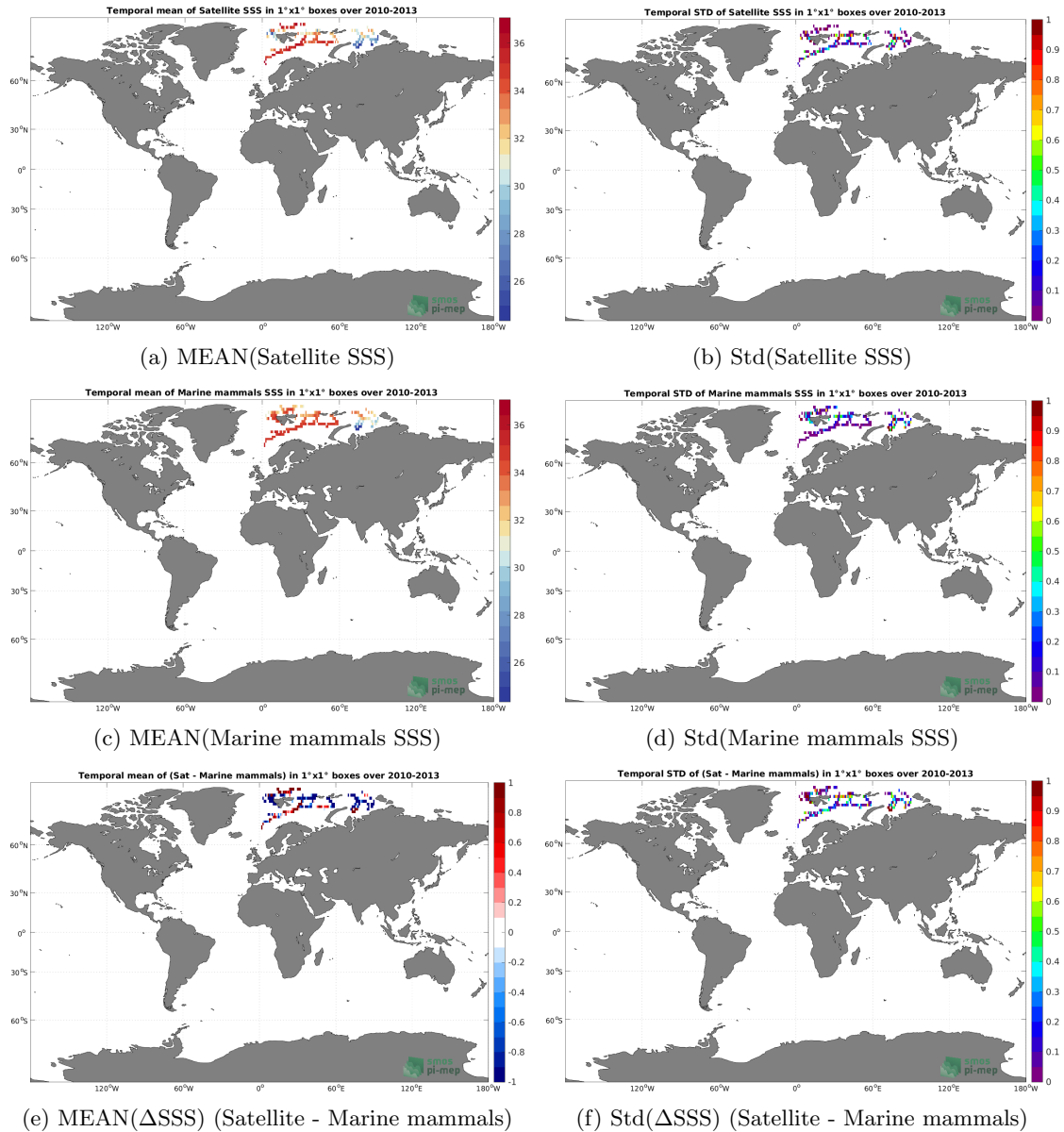
Figure 6: Temporal mean (left) and Std (right) of SSS from SMOS SSS L3 Arctic v1.1 - Monthly (CATDS-CECOS-LOCEAN) (top), Marine mammals (middle), and of \Delta SSS (Satellite - Marine mammals). Only match-up pairs are used to generate these maps.
