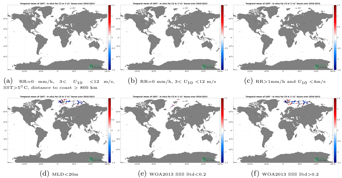
Figure 12: Temporal mean gridded over spatial boxes of size 1^{\circ}\times 1^{\circ} of \Delta\text{SSS} (SMOS SSS L3 Arctic v1.1 - Monthly (CATDS-CECOS-LOCEAN) - Marine mammals) for 6 different subdatasets corresponding to: RR=0 mm/h, 3 < U_{10} < 12 m/s, SST > 5^{\circ}\text{C} , distance to coast > 800 km (a), RR=0 mm/h, 3 < U_{10} < 12 m/s (b), RR > 1\text{mm/h} and U_{10} < 4\text{m/s} (c), MLD < 20\text{m} (d), WOA2013 SSS Std < 0.2 (e), WOA2013 SSS Std > 0.2 (f).
