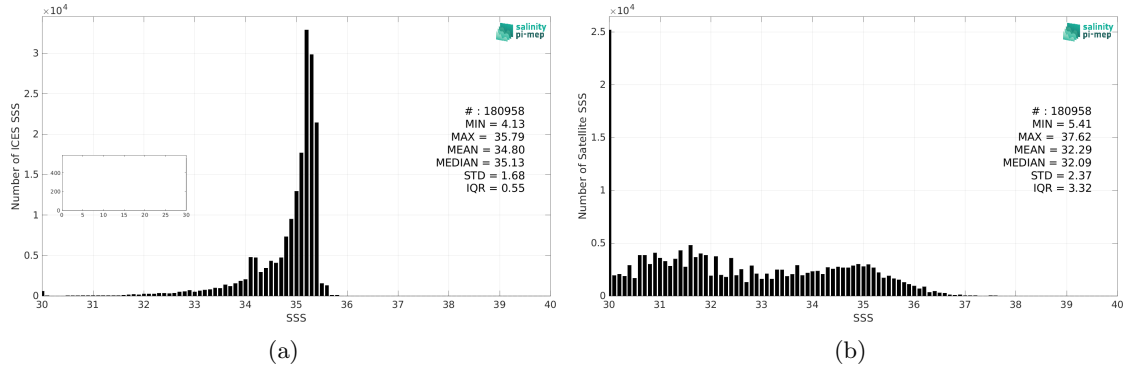
Figure 2: Histograms of SSS from ICES (a) and SMOS SSS L3 Arctic v1.1 - Monthly (CATDS-CECOS-LOCEAN) (b) considering all match-up pairs per bins of 0.1 over the Global Ocean Pi-MEP region and for the full satellite product period.
