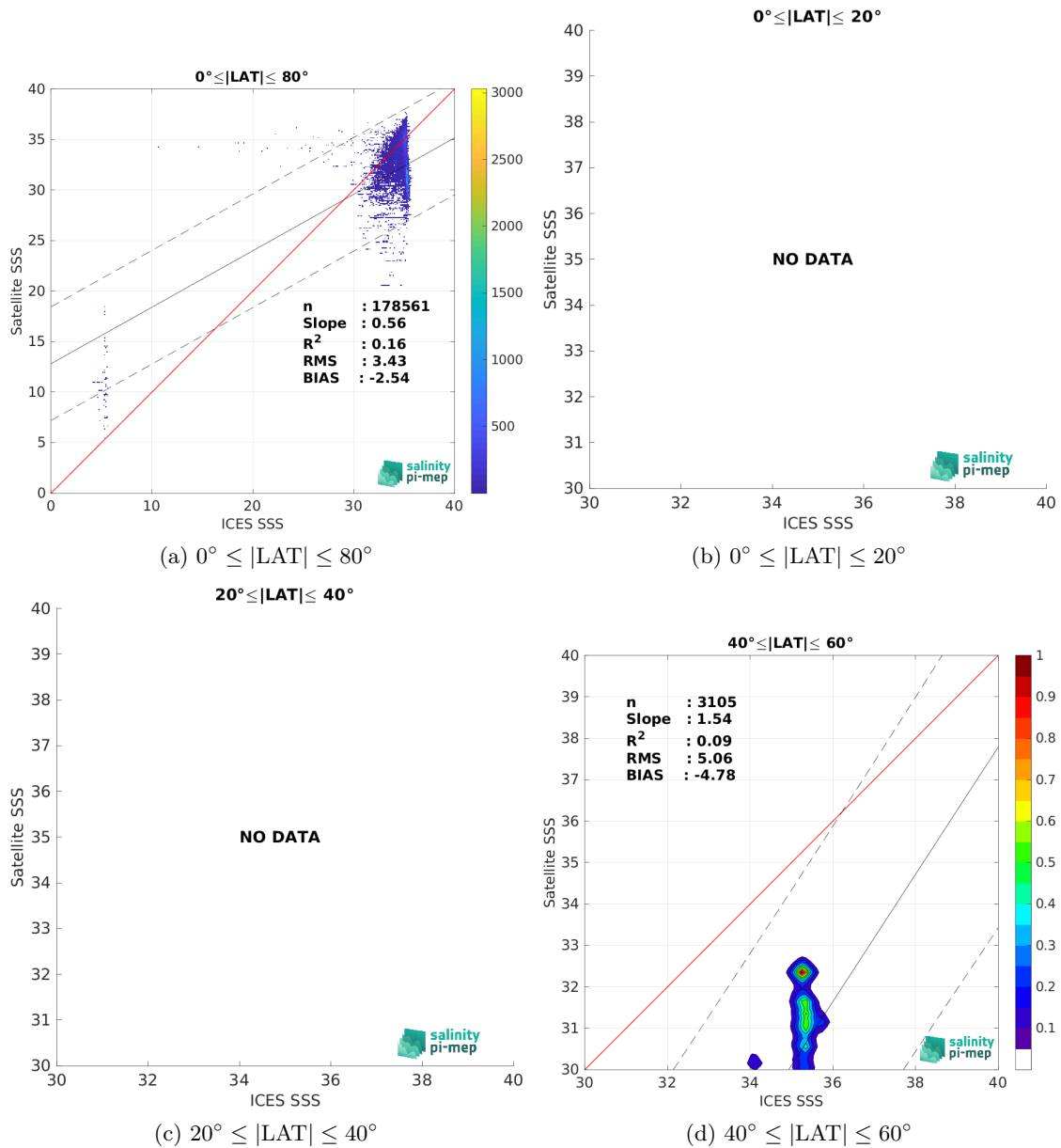
Figure 9: Contour maps of the concentration of SMOS SSS L3 Arctic v1.1 - Monthly (CATDS-CECOS-LOCEAN) SSS (y-axis) versus ICES SSS (x-axis) at match-up pairs for different latitude bands. For each plot, the red line shows x=y . The black thin and dashed lines indicate a linear fit through the data cloud and the \pm 95\% confidence levels, respectively. The number match-up pairs n , the slope and R^2 coefficient of the linear fit, the root mean square (RMS) and the mean bias between satellite and in situ data are indicated for each latitude band in each plots.
