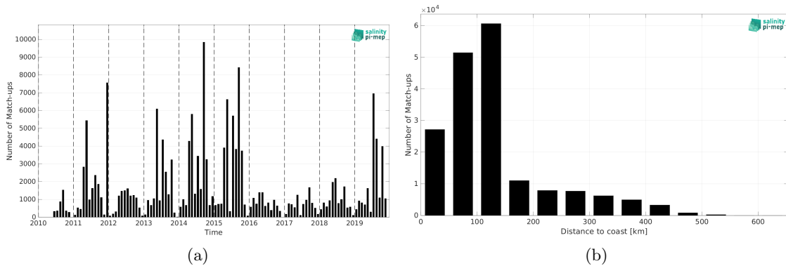
Figure 1: Number of match-ups between ICES and SMOS SSS L3 Arctic v1.1 - Monthly (CATDS-CECOS-LOCEAN) SSS as a function of time (a) and as function of the distance to coast (b) over the Global Ocean Pi-MEP region and for the full satellite product period.
