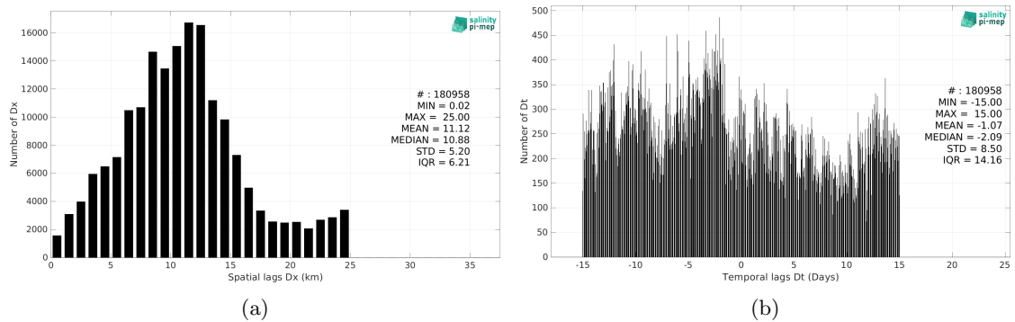
Figure 5: Histograms of the spatial (a) and temporal (b) lags between the location/time of the ICES measurement and the date of the corresponding SMOS SSS L3 Arctic v1.1 - Monthly (CATDS-CECOS-LOCEAN) SSS pixel.
