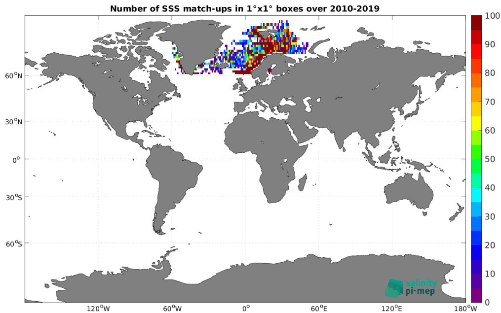
Figure 4: Number of SSS match-ups between ICES SSS and the SMOS SSS L3 Arctic v1.1 - Monthly (CATDS-CECOS-LOCEAN) SSS product for the Global Ocean Pi-MEP region over 1^\circ \times 1^\circ boxes and for the full satellite product period.
