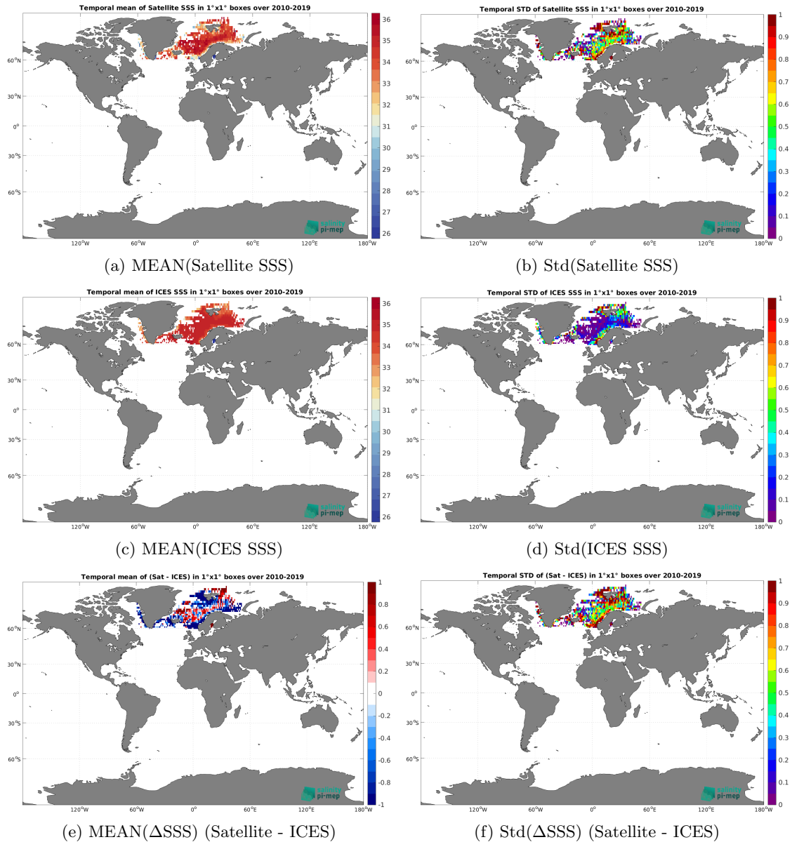
Figure 6: Temporal mean (left) and Std (right) of SSS from SMOS SSS L3 Arctic v1.1 - Monthly (CATDS-CECOS-LOCEAN) (top), ICES (middle), and of \Delta SSS (Satellite - ICES). Only match-up pairs are used to generate these maps.
