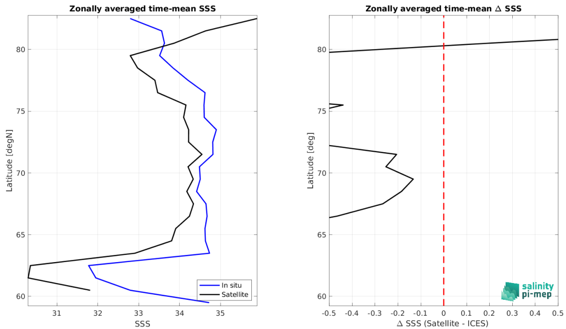
Figure 8: Left panel: Zonal mean SSS from SMOS SSS L3 Arctic v1.1 - Monthly (CATDS-CECOS-LOCEAN) satellite product (black) and from ICES (blue). Right panel: Zonal mean of \Delta SSS (Satellite - ICES) for all the collected Pi-MEP match-up pairs estimated over the full satellite product period.
