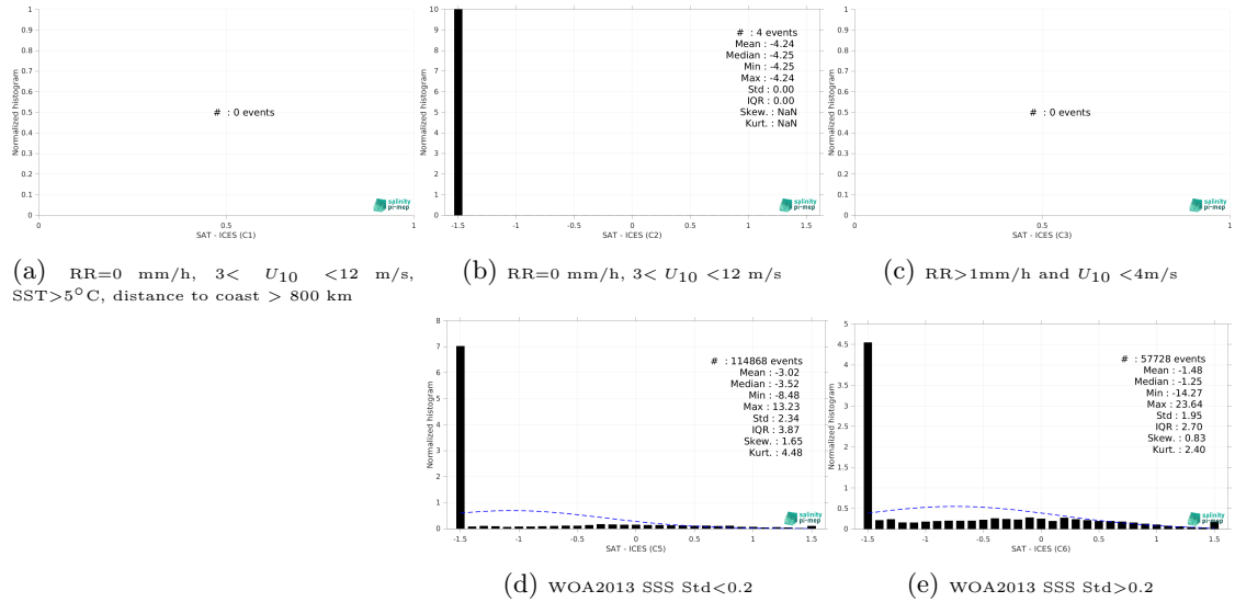
Figure 13: Normalized histogram of \Delta SSS (SMOS SSS L3 Arctic v1.1 - Monthly (CATDS-CECOS-LOCEAN) - ICES) for 5 different subdatasets corresponding to: RR=0 mm/h, 3 < U_{10} < 12 m/s, SST>5°C, distance to coast > 800 km (a), RR=0 mm/h, 3 < U_{10} < 12 m/s (b), RR>1mm/h and U_{10} < 4 m/s (c), WOA2013 SSS Std<0.2 (d), WOA2013 SSS Std>0.2 (e).
