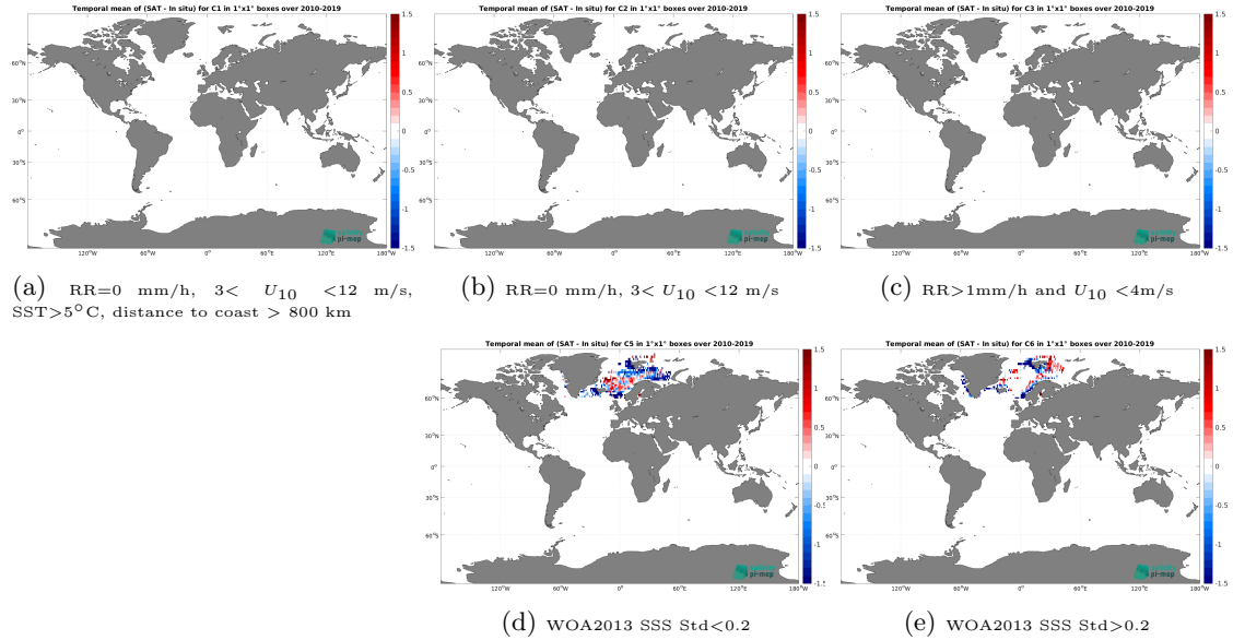
Figure 12: Temporal mean gridded over spatial boxes of size 1^{\circ}\times 1^{\circ} of \Delta\text{SSS} (SMOS SSS L3 Arctic v1.1 - Monthly (CATDS-CECOS-LOCEAN) - ICES) for 5 different subdatasets corresponding to:RR=0 mm/h, 3 < U_{10} < 12 m/s, SST > 5^{\circ}\text{C} , distance to coast > 800 km (a), RR=0 mm/h, 3 < U_{10} < 12 m/s (b), RR > 1 mm/h and U_{10} < 4 m/s (c), WOA2013 SSS Std < 0.2 (d), WOA2013 SSS Std > 0.2 (e).
