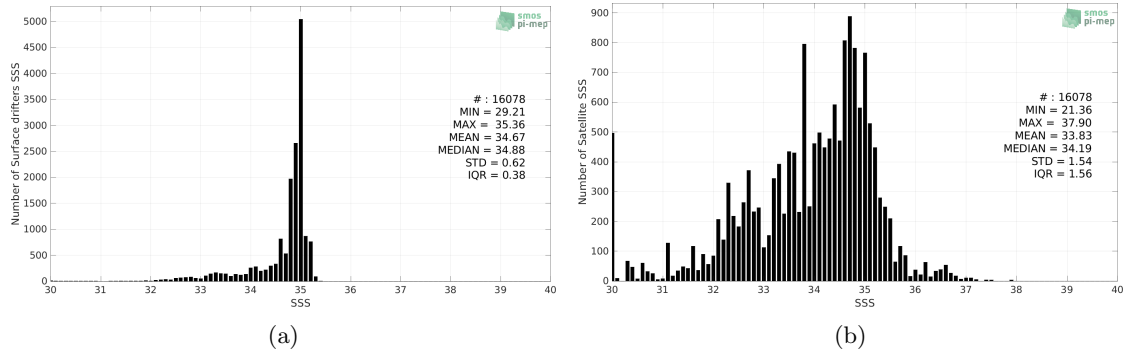
Figure 2: Histograms of SSS from Surface drifters (a) and SMOS SSS L3 Arctic v1.1 - Monthly (CATDS-CECOS-LOCEAN) (b) considering all match-up pairs per bins of 0.1 over the Global Ocean Pi-MEP region and for the full satellite product period.
