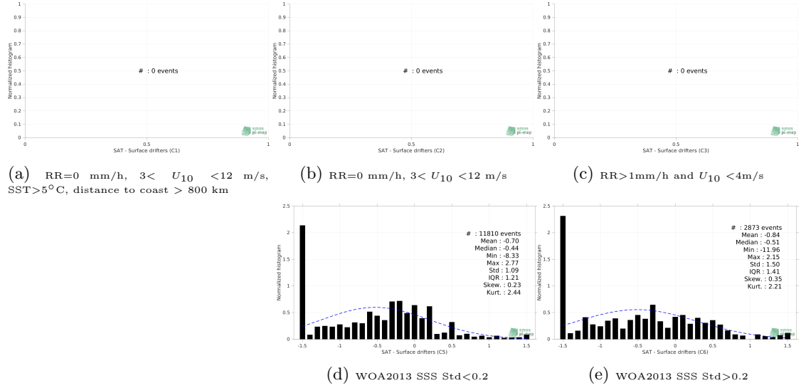
Figure 12: Normalized histogram of \Delta SSS (SMOS SSS L3 Arctic v1.1 - Monthly (CATDS-CECOS-LOCEAN) - Surface drifters) for 5 different subdatasets corresponding to: RR=0 mm/h, 3 < U_{10} < 12 m/s, SST > 5°C, distance to coast > 800 km (a), RR=0 mm/h, 3 < U_{10} < 12 m/s (b), RR > 1mm/h and U_{10} < 4 m/s (c), WOA2013 SSS Std < 0.2 (d), WOA2013 SSS Std > 0.2 (e).
