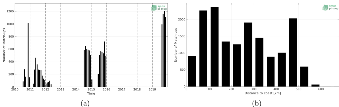
Figure 1: Number of match-ups between Surface drifters and SMOS SSS L3 Arctic v1.1 - Monthly (CATDS-CECOS-LOCEAN) SSS as a function of time (a) and as function of the distance to coast (b) over the Global Ocean Pi-MEP region and for the full satellite product period.
