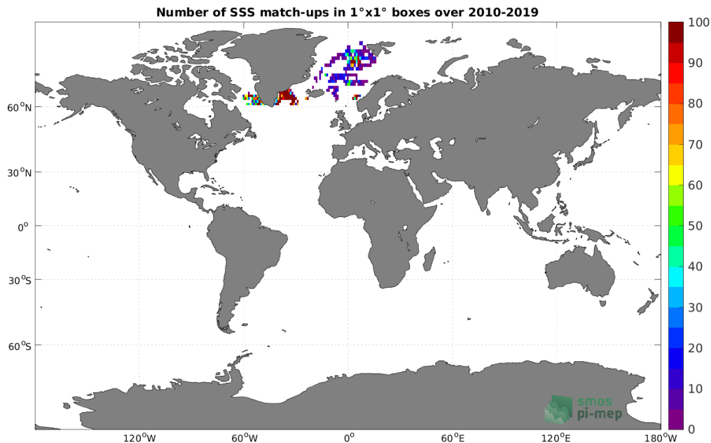
Figure 3: Number of SSS match-ups between Surface drifters SSS and the SMOS SSS L3 Arctic v1.1 - Monthly (CATDS-CECOS-LOCEAN) SSS product for the Global Ocean Pi-MEP region over 1^\circ \times 1^\circ boxes and for the full satellite product period.
