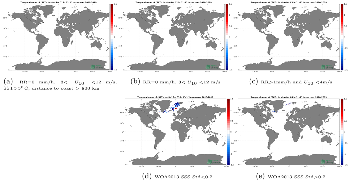
Figure 11: Temporal mean gridded over spatial boxes of size 1^{\circ}\times 1^{\circ} of \Delta\text{SSS} (SMOS SSS L3 Arctic v1.1 - Monthly (CATDS-CECOS-LOCEAN) - Surface drifters) for 5 different subdatasets corresponding to:RR=0 mm/h, 3 < U_{10} < 12 m/s, SST >5^{\circ}\text{C} , distance to coast > 800 km (a), RR=0 mm/h, 3 < U_{10} < 12 m/s (b), RR >1 mm/h and U_{10} < 4 m/s (c), WOA2013 SSS Std <0.2 (d), WOA2013 SSS Std >0.2 (e).
