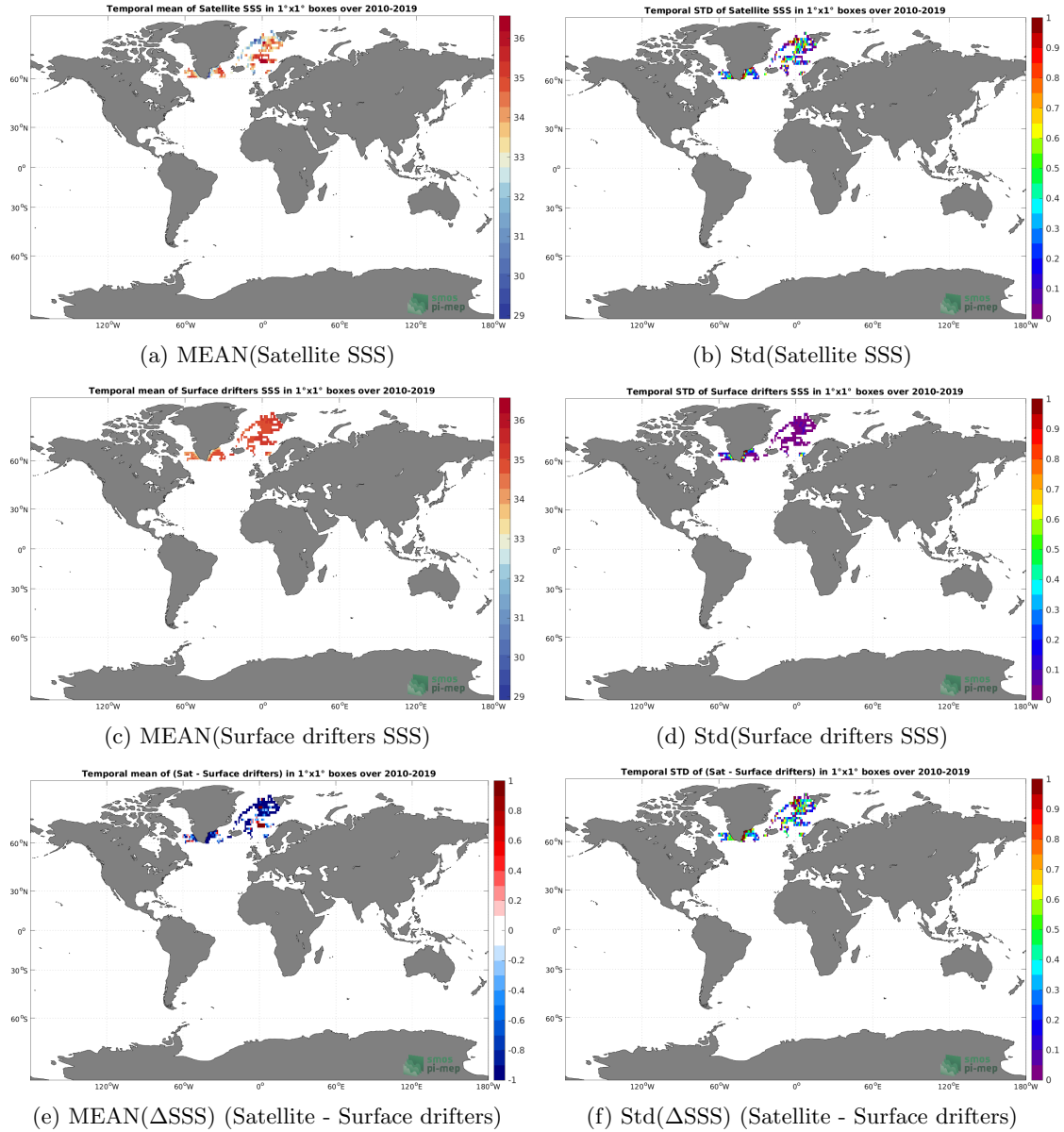
Figure 5: Temporal mean (left) and Std (right) of SSS from SMOS SSS L3 Arctic v1.1 - Monthly (CATDS-CECOS-LOCEAN) (top), Surface drifters (middle), and of \Delta SSS (Satellite - Surface drifters). Only match-up pairs are used to generate these maps.
