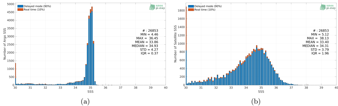
Figure 2: Histograms of SSS from Argo (a) and SMOS SSS L3 Arctic v1.1 - Monthly (CATDS-CECOS-LOCEAN) (b) considering all match-up pairs per bins of 0.1 over the Global Ocean Pi-MEP region and for the full satellite product period.
