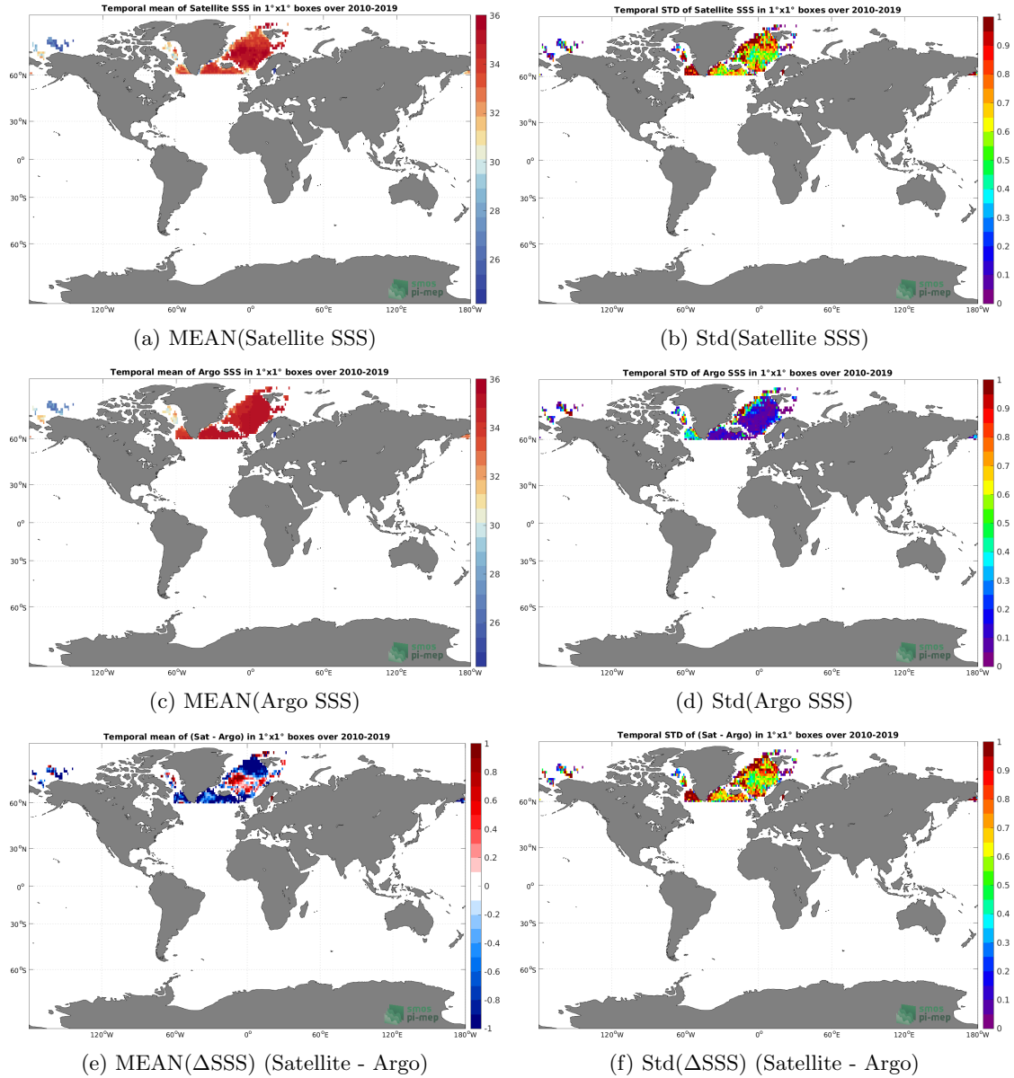
Figure 6: Temporal mean (left) and Std (right) of SSS from SMOS SSS L3 Arctic v1.1 - Monthly (CATDS-CECOS-LOCEAN) (top), Argo (middle), and of \Delta SSS (Satellite - Argo). Only match-up pairs are used to generate these maps.
