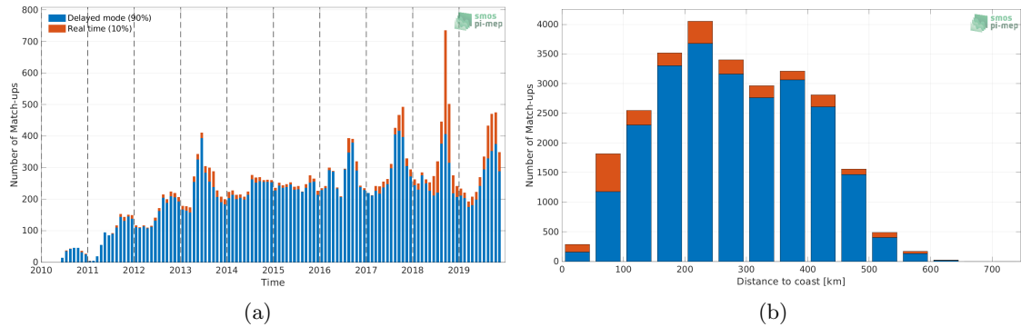
Figure 1: Number of match-ups between Argo and SMOS SSS L3 Arctic v1.1 - Monthly (CATDS-CECOS-LOCEAN) SSS as a function of time (a) and as function of the distance to coast (b) over the Global Ocean Pi-MEP region and for the full satellite product period.
