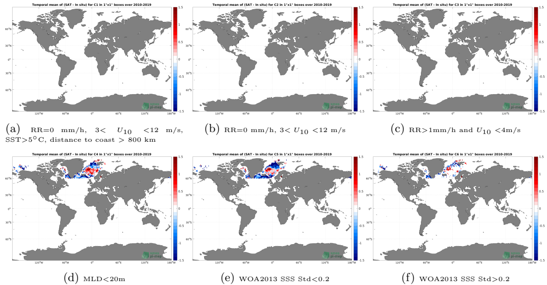
Figure 12: Temporal mean gridded over spatial boxes of size 1^{\circ}\times 1^{\circ} of \Delta\text{SSS} (SMOS SSS L3 Arctic v1.1 - Monthly (CATDS-CECOS-LOCEAN) - Argo) for 6 different subdatasets corresponding to:RR=0 mm/h, 3 < U_{10} < 12 m/s, SST > 5^{\circ}\text{C} , distance to coast > 800 km (a), RR=0 mm/h, 3 < U_{10} < 12 m/s (b), RR > 1\text{mm/h} and U_{10} < 4\text{m/s} (c),MLD < 20\text{m} (d),WOA2013 SSS Std < 0.2 (e),WOA2013 SSS Std > 0.2 (f).
