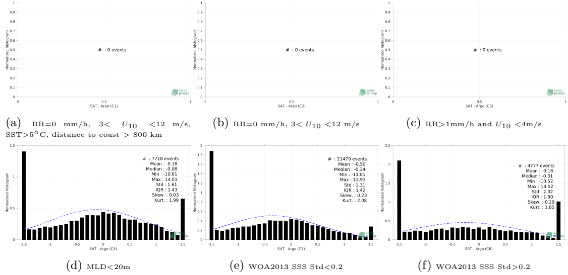
Figure 13: Normalized histogram of \Delta\text{SSS} (SMOS SSS L3 Arctic v1.1 - Monthly (CATDS-CECOS-LOCEAN) - Argo) for 6 different subdatasets corresponding to: RR=0 mm/h, 3 < U_{10} < 12 m/s, SST > 5^{\circ}\text{C} , distance to coast > 800 km (a), RR=0 mm/h, 3 < U_{10} < 12 m/s (b), RR > 1\text{mm/h} and U_{10} < 4\text{m/s} (c), MLD < 20\text{m} (d), WOA2013 SSS Std < 0.2 (e), WOA2013 SSS Std > 0.2 (f).
