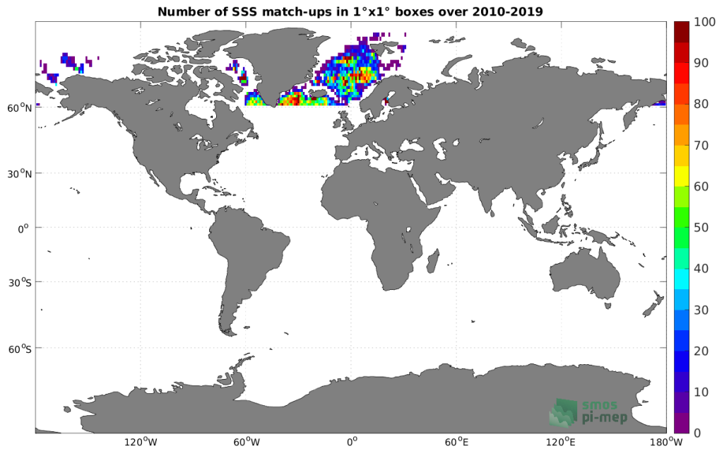
Figure 4: Number of SSS match-ups between Argo SSS and the SMOS SSS L3 Arctic v1.1 - Monthly (CATDS-CECOS-LOCEAN) SSS product for the Global Ocean Pi-MEP region over 1^\circ \times 1^\circ boxes and for the full satellite product period.
