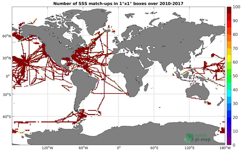
Figure 4: Number of SSS match-ups between TSG (SAMOS) SSS and the SMOS SSS L3 v2 - Monthly - 0.25 Deg (CATDS-CECOS-IFREMER) SSS product for the Global Ocean Pi-MEP region over 1^\circ \times 1^\circ boxes and for the full satellite product period.
