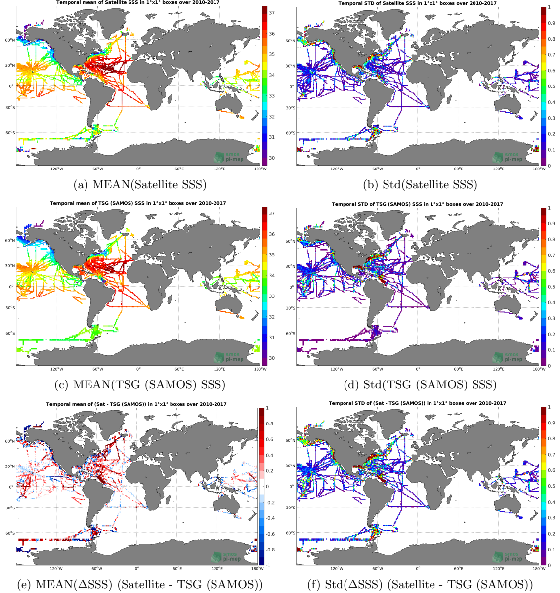
Figure 6: Temporal mean (left) and Std (right) of SSS from SMOS SSS L3 v2 - Monthly - 0.25 Deg (CATDS-CECOS-IFREMER) (top), TSG (SAMOS) (middle), and of \Delta SSS (Satellite - TSG (SAMOS)). Only match-up pairs are used to generate these maps.
