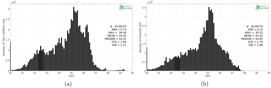
Figure 2: Histograms of SSS from TSG (SAMOS) (a) and SMOS SSS L3 v2 - Monthly - 0.25 Deg (CATDS-CECOS-IFREMER) (b) considering all match-up pairs per bins of 0.1 over the Global Ocean Pi-MEP region and for the full satellite product period.
