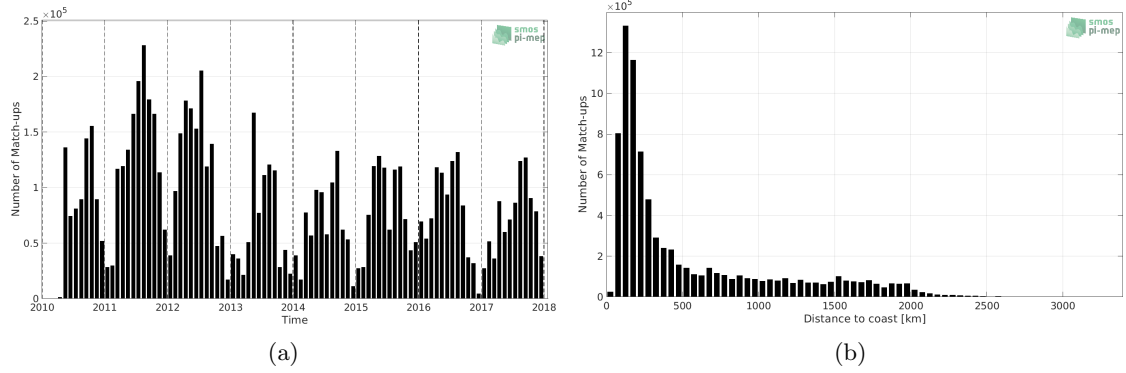
Figure 1: Number of match-ups between TSG (SAMOS) and SMOS SSS L3 v2 - Monthly - 0.25 Deg (CATDS-CECOS-IFREMER) SSS as a function of time (a) and as function of the distance to coast (b) over the Global Ocean Pi-MEP region and for the full satellite product period.
