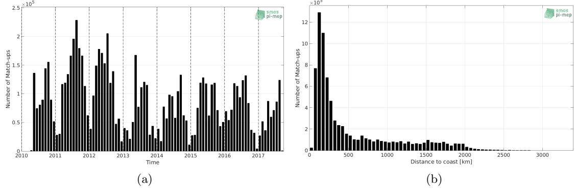
Figure 1: Number of match-ups between TSG-SAMOS and SMOS-L3-CATDS-IFREMER-CECOS-V2-MONTHLY-0.25DEG SSS as a function of time (a) and as function of the distance to coast (b) over the Global Ocean Pi-MEP region and for the full satellite product period.
