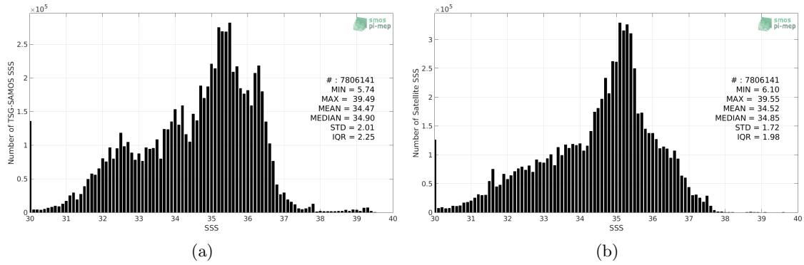
Figure 2: Histograms of SSS from TSG-SAMOS (a) and SMOS-L3-CATDS-IFREMER-CECOS-V2-MONTHLY-0.25DEG (b) considering all match-up pairs per bins of 0.1 over the Global Ocean Pi-MEP region and for the full satellite product period.
