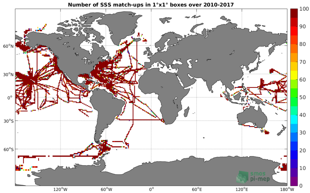
Figure 4: Number of SSS match-ups between TSG-SAMOS SSS and the SMOS-L3-CATDS-IFREMER-CECOS-V2-MONTHLY-0.25DEG SSS product for the Global Ocean Pi-MEP region over 1°x1° boxes and for the full satellite product period.
