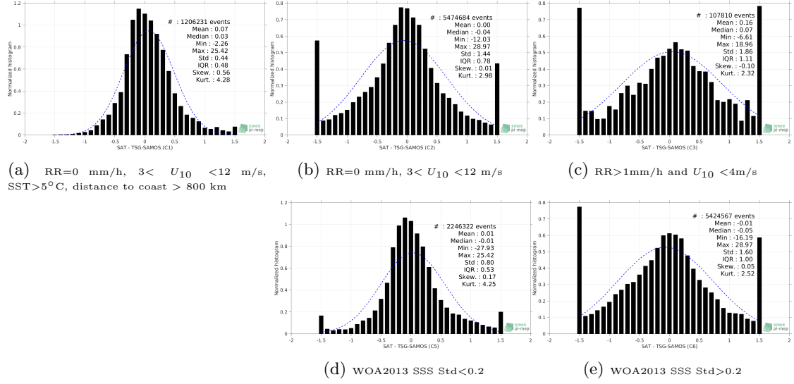
Figure 13: Normalized histogram of \Delta SSS (SMOS-L3-CATDS-IFREMER-CECOS-V2-MONTHLY-0.25DEG - TSG-SAMOS) for 5 different subdatasets corresponding to: RR=0 mm/h, 3 < U_{10} < 12 m/s, SST > 5°C, distance to coast > 800 km (a), RR=0 mm/h, 3 < U_{10} < 12 m/s (b), RR > 1mm/h and U_{10} < 4 m/s (c), WOA2013 SSS Std < 0.2 (d), WOA2013 SSS Std > 0.2 (e).
