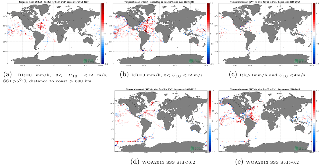
Figure 12: Temporal mean gridded over spatial boxes of size 1^\circ \times 1^\circ of \Delta SSS (SMOS-L3-CATDS-IFREMER-CECOS-V2-MONTHLY-0.25DEG - TSG-SAMOS) for 5 different subdatasets corresponding to:RR=0 mm/h, 3 < U_{10} < 12 m/s, SST >5^\circ C, distance to coast > 800 km (a), RR=0 mm/h, 3 < U_{10} < 12 m/s (b), RR >1 mm/h and U_{10} < 4 m/s (c), WOA2013 SSS Std <0.2 (d), WOA2013 SSS Std >0.2 (e).
