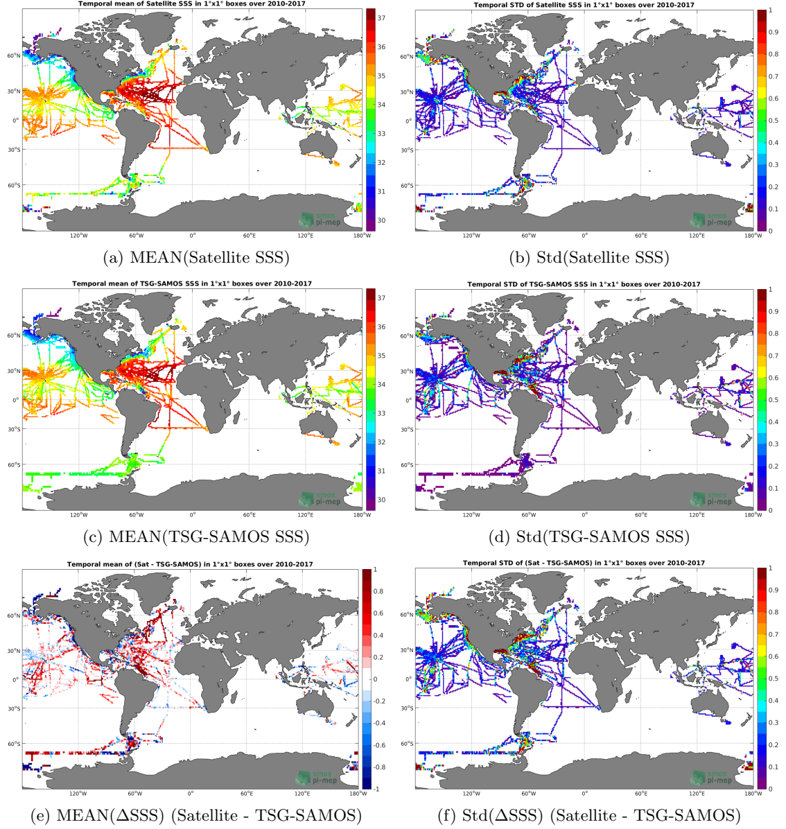
Figure 6: Temporal mean (left) and Std (right) of SSS from SMOS-L3-CATDS-IFREMER-CECOS-V2-MONTHLY-0.25DEG (top), TSG-SAMOS (middle), and of \Delta SSS (Satellite - TSG-SAMOS). Only match-up pairs are used to generate these maps.
