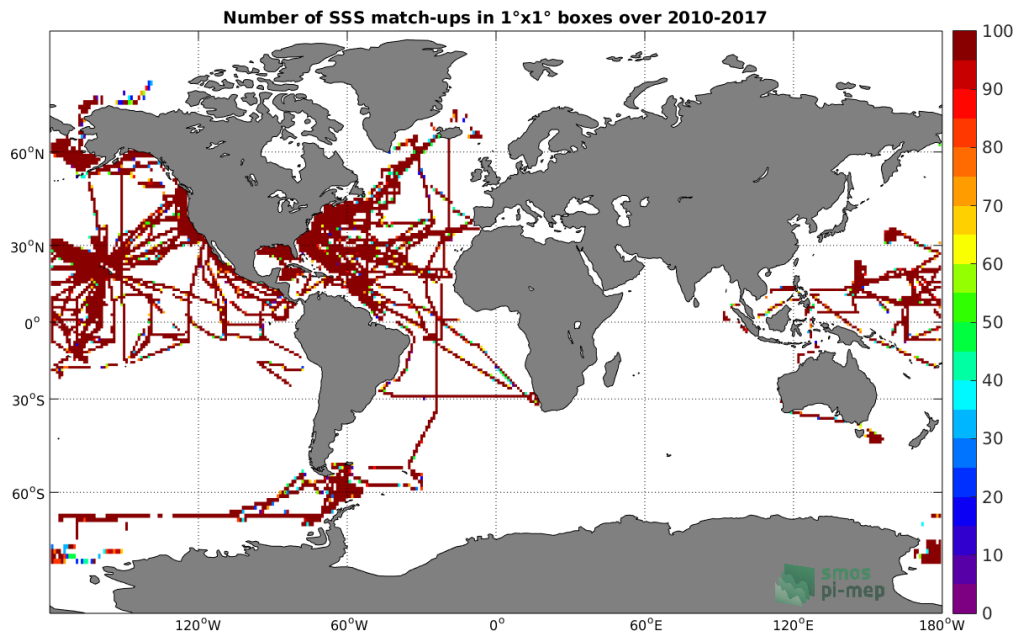
Figure 4: Number of SSS match-ups between TSG-SAMOS SSS and the SMOS-L3-CATDS-IFREMER-CECOS-V2-MONTHLY-0.25DEG SSS product for the Global Ocean Pi-MEP region over 1^\circ \times 1^\circ boxes and for the full satellite product period.
