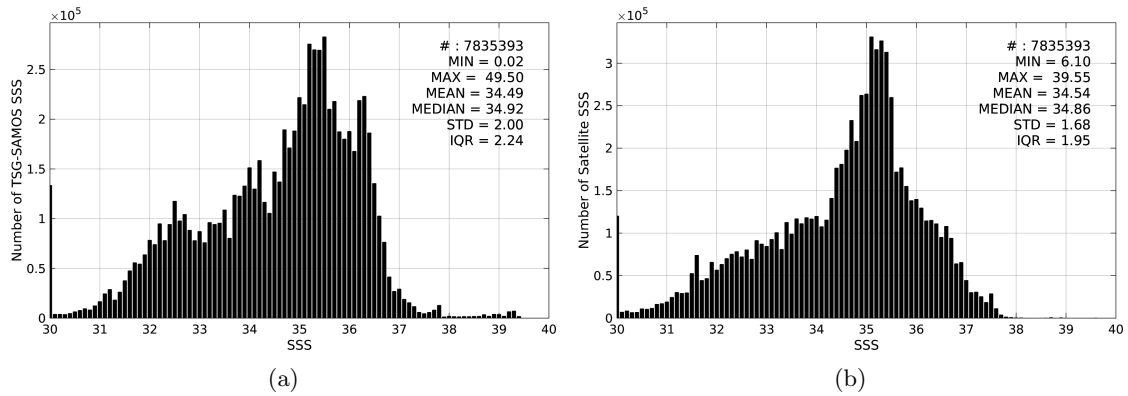
Figure 2: Histograms of SSS from TSG-SAMOS (a) and SMOS-L3-CATDS-IFREMER-CECOS-V2-MONTHLY-0.25DEG (b) considering all match-up pairs per bins of 0.1 over the Global Ocean Pi-MEP region and for the full satellite product period.
