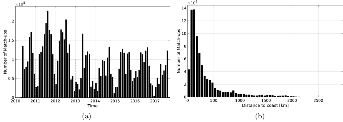
Figure 1: Number of match-ups between TSG-SAMOS and SMOS-L3-CATDS-IFREMER-CECOS-V2-MONTHLY-0.25DEG SSS as a function of time (a) and as function of the distance to coast (b) over the Global Ocean Pi-MEP region and for the full satellite product period.
