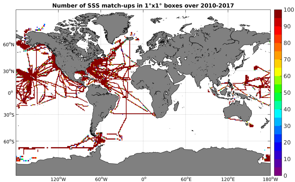
Figure 4: Number of SSS match-ups between TSG-SAMOS SSS and the SMOS-L3-CATDS-IFREMER-CECOS-V2-MONTHLY-0.25DEG SSS product for the Global Ocean Pi-MEP region over 1^\circ \times 1^\circ boxes and for the full satellite product period.
