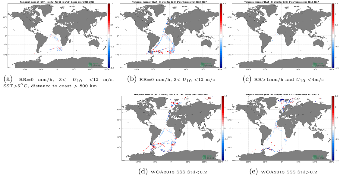
Figure 12: Temporal mean gridded over spatial boxes of size 1^\circ \times 1^\circ of \Delta SSS (SMOS SSS L3 v2 - Monthly - 0.25 Deg (CATDS-CECOS-IFREMER) - TSG (Polarstern)) for 5 different subdatasets corresponding to: RR=0 mm/h, 3 < U_{10} < 12 m/s, SST > 5^\circ C , distance to coast > 800 km (a), RR=0 mm/h, 3 < U_{10} < 12 m/s (b), RR > 1 mm/h and U_{10} < 4 m/s (c), WOA2013 SSS Std < 0.2 (d), WOA2013 SSS Std > 0.2 (e).
