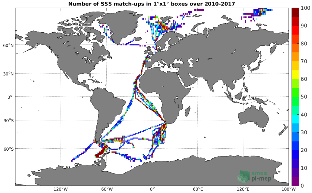
Figure 4: Number of SSS match-ups between TSG (Polarstern) SSS and the SMOS SSS L3 v2 - Monthly - 0.25 Deg (CATDS-CECOS-IFREMER) SSS product for the Global Ocean Pi-MEP region over 1^\circ \times 1^\circ boxes and for the full satellite product period.
