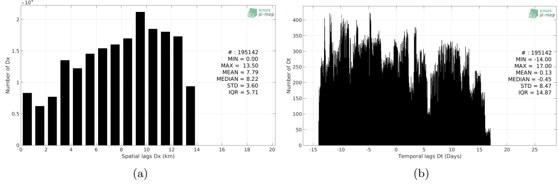
Figure 5: Histograms of the spatial (a) and temporal (b) lags between the time of the TSG (Polarstern) measurements and the date of the corresponding SMOS SSS L3 v2 - Monthly - 0.25 Deg (CATDS-CECOS-IFREMER) SSS product.
