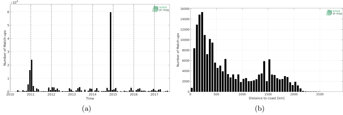
Figure 1: Number of match-ups between TSG-POLARSTERN and SMOS L3 v2 - Monthly - 0.25 Deg (CATDS-CECOS-IFREMER) SSS as a function of time (a) and as function of the distance to coast (b) over the Global Ocean Pi-MEP region and for the full satellite product period.
