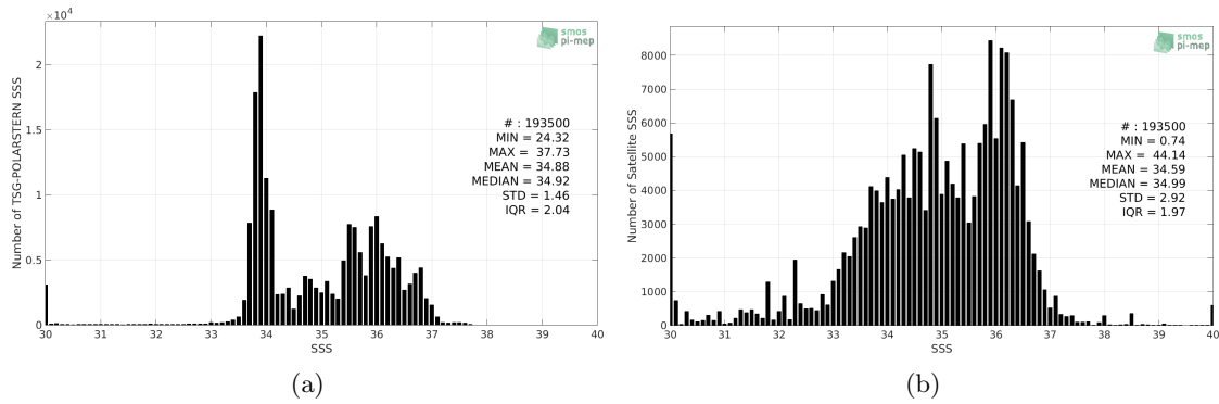
Figure 2: Histograms of SSS from TSG-POLARSTERN (a) and SMOS L3 v2 - Monthly - 0.25 Deg (CATDS-CECOS-IFREMER) (b) considering all match-up pairs per bins of 0.1 over the Global Ocean Pi-MEP region and for the full satellite product period.
