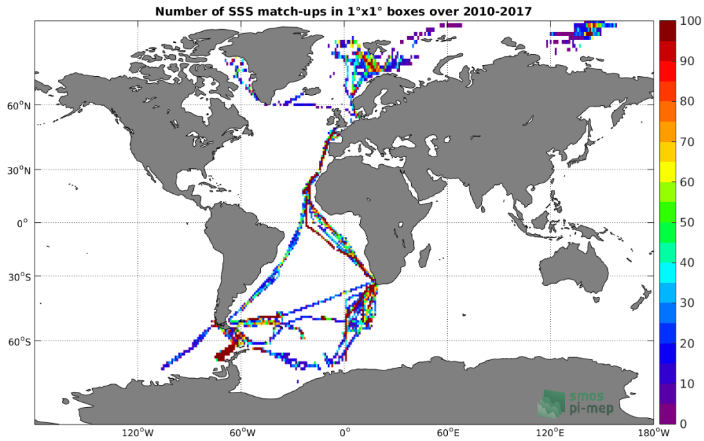
Figure 4: Number of SSS match-ups between TSG-POLARSTERN SSS and the SMOS L3 v2 - Monthly - 0.25 Deg (CATDS-CECOS-IFREMER) SSS product for the Global Ocean Pi-MEP region over 1^\circ \times 1^\circ boxes and for the full satellite product period.
