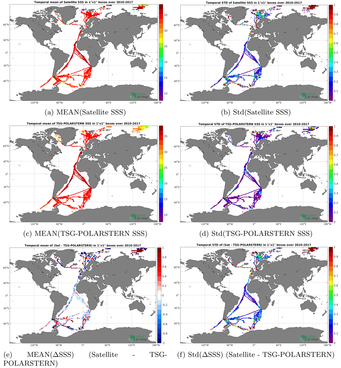
Figure 6: Temporal mean (left) and Std (right) of SSS from SMOS L3 v2 - Monthly - 0.25 Deg (CATDS-CECOS-IFREMER) (top), TSG-POLARSTERN (middle), and of \Delta SSS (Satellite - TSG-POLARSTERN). Only match-up pairs are used to generate these maps.
