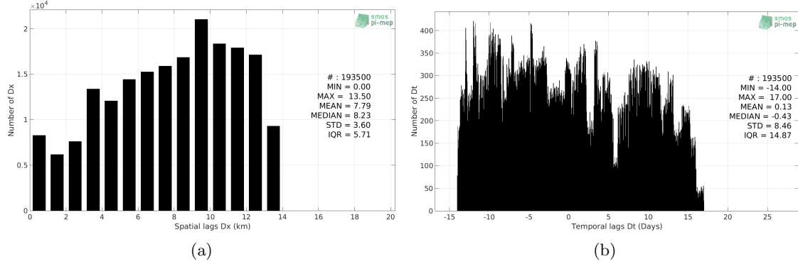
Figure 5: Histograms of the spatial (a) and temporal (b) lags between the time of the TSG-POLARSTERN measurements and the date of the corresponding SMOS L3 v2 - Monthly - 0.25 Deg (CATDS-CECOS-IFREMER) SSS product.
