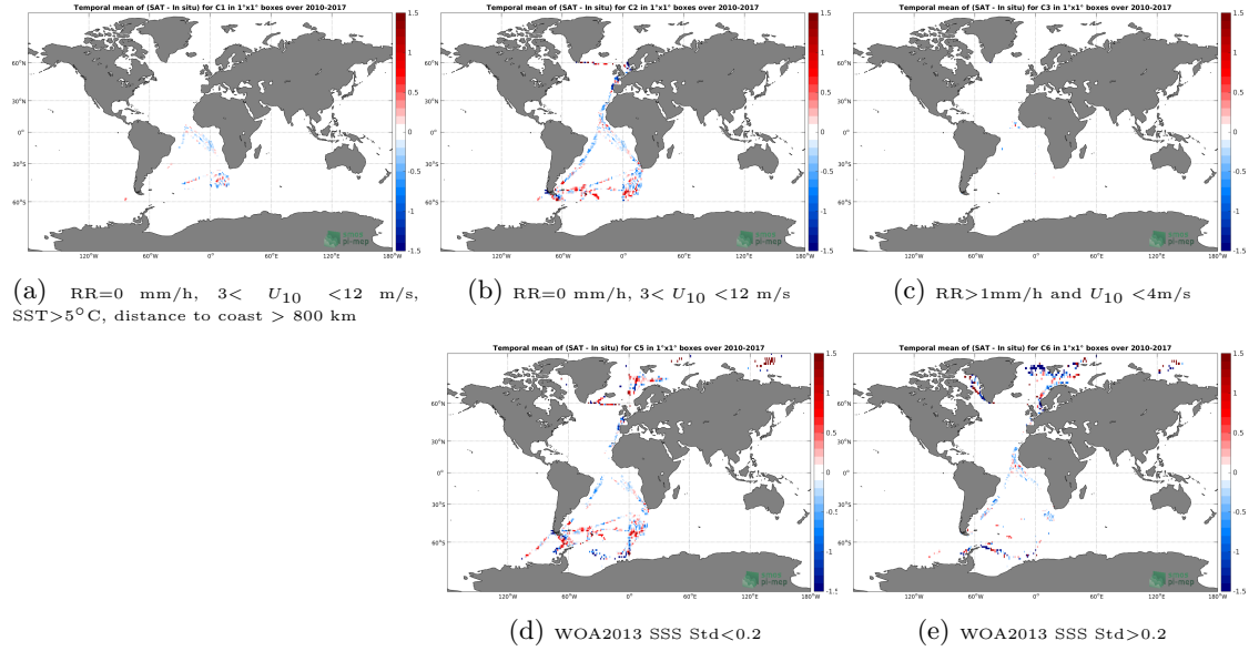
Figure 12: Temporal mean gridded over spatial boxes of size 1^\circ \times 1^\circ of \Delta SSS (SMOS L3 v2 - Monthly - 0.25 Deg (CATDS-CECOS-IFREMER) - TSG-POLARSTERN) for 5 different sub-datasets corresponding to: RR=0 mm/h, 3 < U_{10} < 12 m/s, SST >5^\circ\text{C} , distance to coast > 800 km (a), RR=0 mm/h, 3 < U_{10} < 12 m/s (b), RR >1 mm/h and U_{10} < 4 m/s (c), WOA2013 SSS Std <0.2 (d), WOA2013 SSS Std >0.2 (e).
