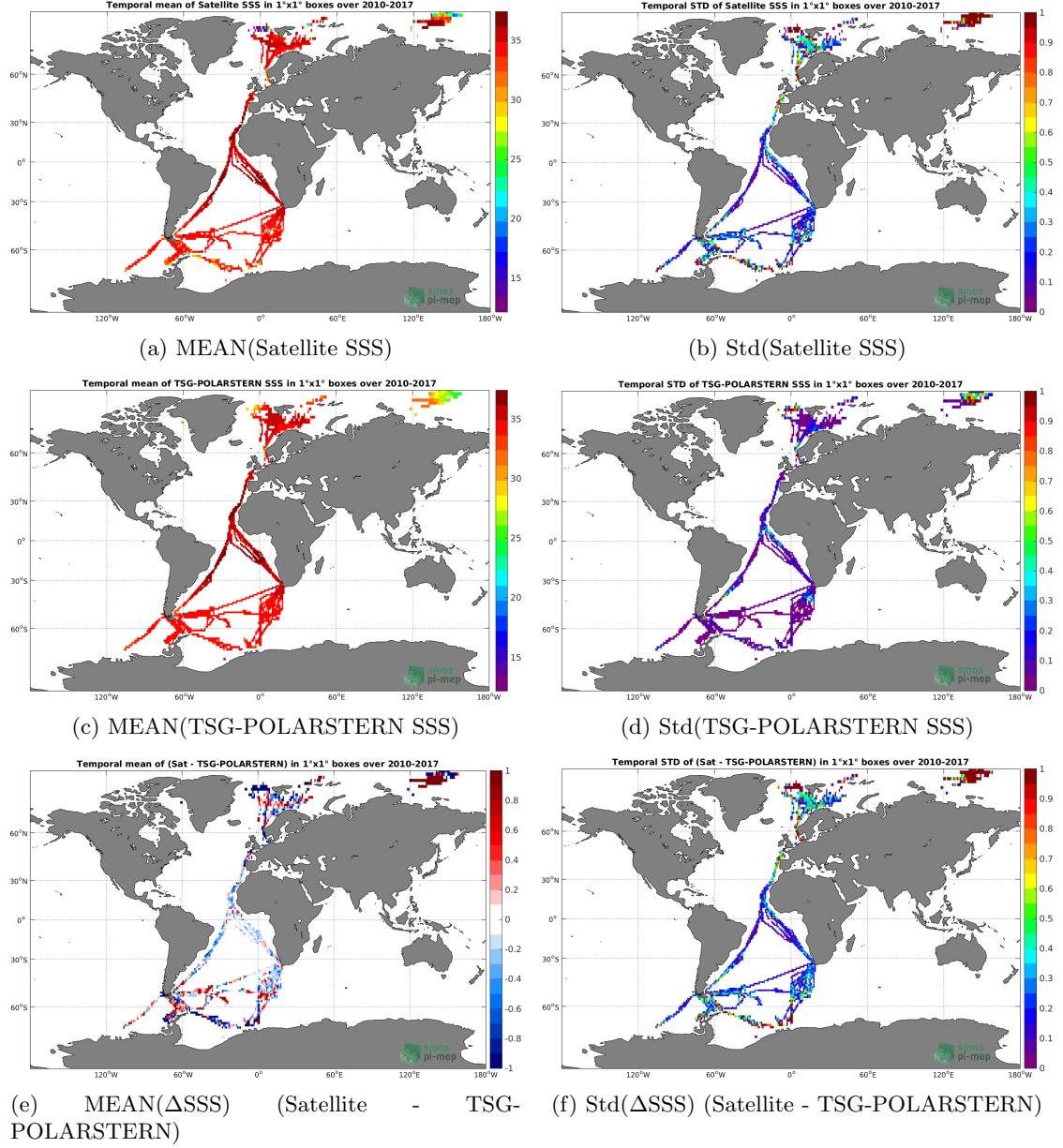
Figure 6: Temporal mean (left) and Std (right) of SSS from SMOS-L3-CATDS-IFREMER-CECOS-V2-MONTHLY-0.25DEG (top), TSG-POLARSTERN (middle), and of \Delta SSS (Satellite - TSG-POLARSTERN). Only match-up pairs are used to generate these maps.
