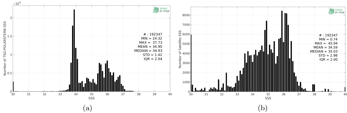
Figure 2: Histograms of SSS from TSG-POLARSTERN (a) and SMOS-L3-CATDS-IFREMER-CECOS-V2-MONTHLY-0.25DEG (b) considering all match-up pairs per bins of 0.1 over the Global Ocean Pi-MEP region and for the full satellite product period.
