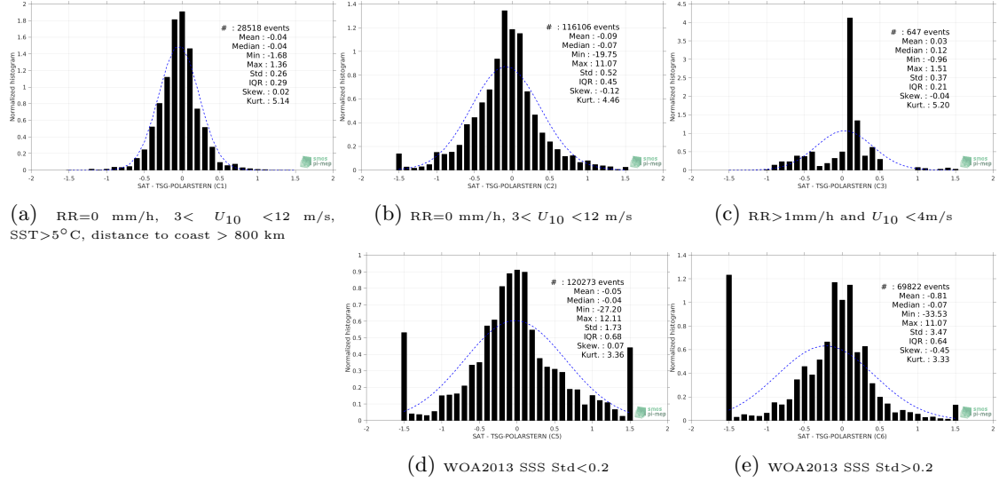
Figure 13: Normalized histogram of \Delta SSS (SMOS-L3-CATDS-IFREMER-CECOS-V2-MONTHLY-0.25DEG - TSG-POLARSTERN) for 5 different subdatasets corresponding to: RR=0 mm/h, 3 < U_{10} < 12 m/s, SST > 5°C, distance to coast > 800 km (a), RR=0 mm/h, 3 < U_{10} < 12 m/s (b), RR > 1mm/h and U_{10} < 4 m/s (c), WOA2013 SSS Std < 0.2 (d), WOA2013 SSS Std > 0.2 (e).
