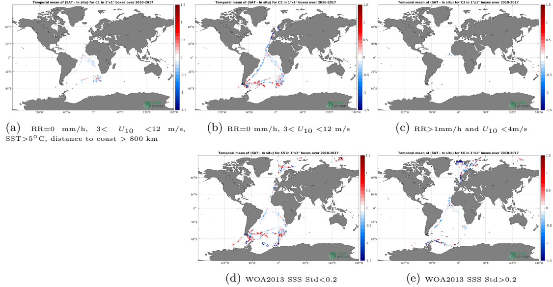
Figure 12: Temporal mean gridded over spatial boxes of size 1^\circ \times 1^\circ of \Delta SSS (SMOS-L3-CATDS-IFREMER-CECOS-V2-MONTHLY-0.25DEG - TSG-POLARSTERN) for 5 different subdatasets corresponding to: RR=0 mm/h, 3 < U_{10} < 12 m/s, SST > 5^\circ C , distance to coast > 800 km (a), RR=0 mm/h, 3 < U_{10} < 12 m/s (b), RR > 1 mm/h and U_{10} < 4 m/s (c), WOA2013 SSS Std < 0.2 (d), WOA2013 SSS Std > 0.2 (e).
