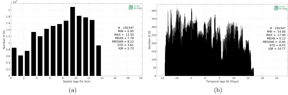
Figure 5: Histograms of the spatial (a) and temporal (b) lags between the time of the TSG-POLARSTERN measurements and the date of the corresponding SMOS-L3-CATDS-IFREMER-CECOS-V2-MONTHLY-0.25DEG SSS product.
