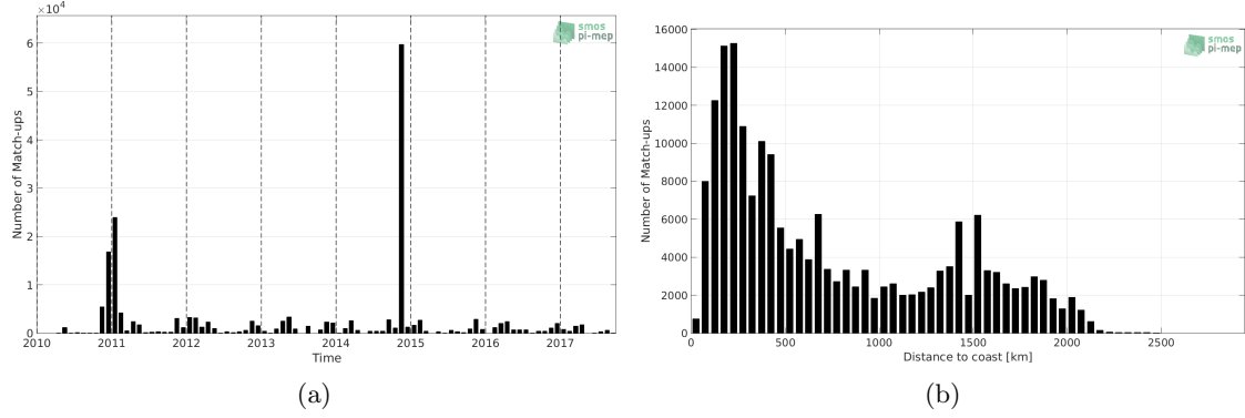
Figure 1: Number of match-ups between TSG-POLARSTERN and SMOS-L3-CATDS-IFREMER-CECOS-V2-MONTHLY-0.25DEG SSS as a function of time (a) and as function of the distance to coast (b) over the Global Ocean Pi-MEP region and for the full satellite product period.
