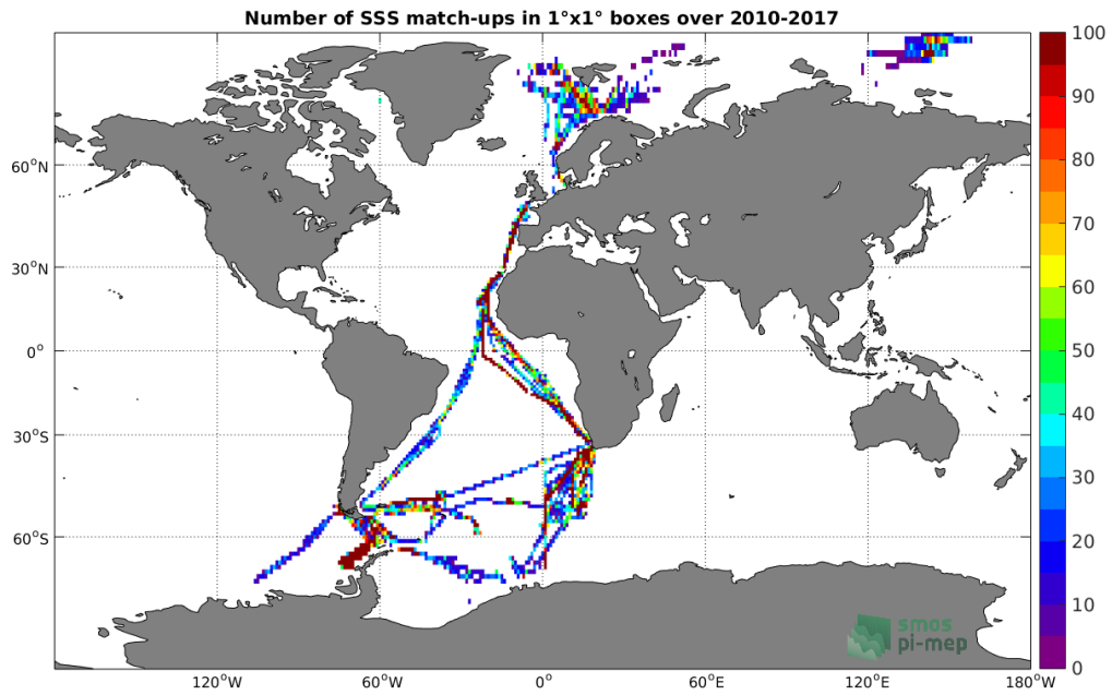
Figure 4: Number of SSS match-ups between TSG-POLARSTERN SSS and the SMOS-L3-CATDS-IFREMER-CECOS-V2-MONTHLY-0.25DEG SSS product for the Global Ocean Pi-MEP region over 1^\circ \times 1^\circ boxes and for the full satellite product period.
