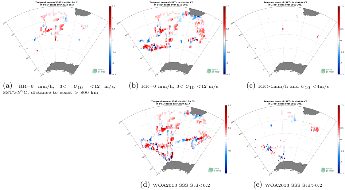
Figure 12: Temporal mean gridded over spatial boxes of size 1^{\circ}\times 1^{\circ} of \Delta\text{SSS} (SMOS SSS L3 v2 - Monthly - 0.25 Deg (CATDS-CECOS-IFREMER) - TSG (NCEI-0170743)) for 5 different subdatasets corresponding to: RR=0 mm/h, 3 < U_{10} < 12 m/s, SST > 5^{\circ}\text{C} , distance to coast > 800 km (a), RR=0 mm/h, 3 < U_{10} < 12 m/s (b), RR > 1\text{mm/h} and U_{10} < 4\text{m/s} (c), WOA2013 SSS Std < 0.2 (d), WOA2013 SSS Std > 0.2 (e).
