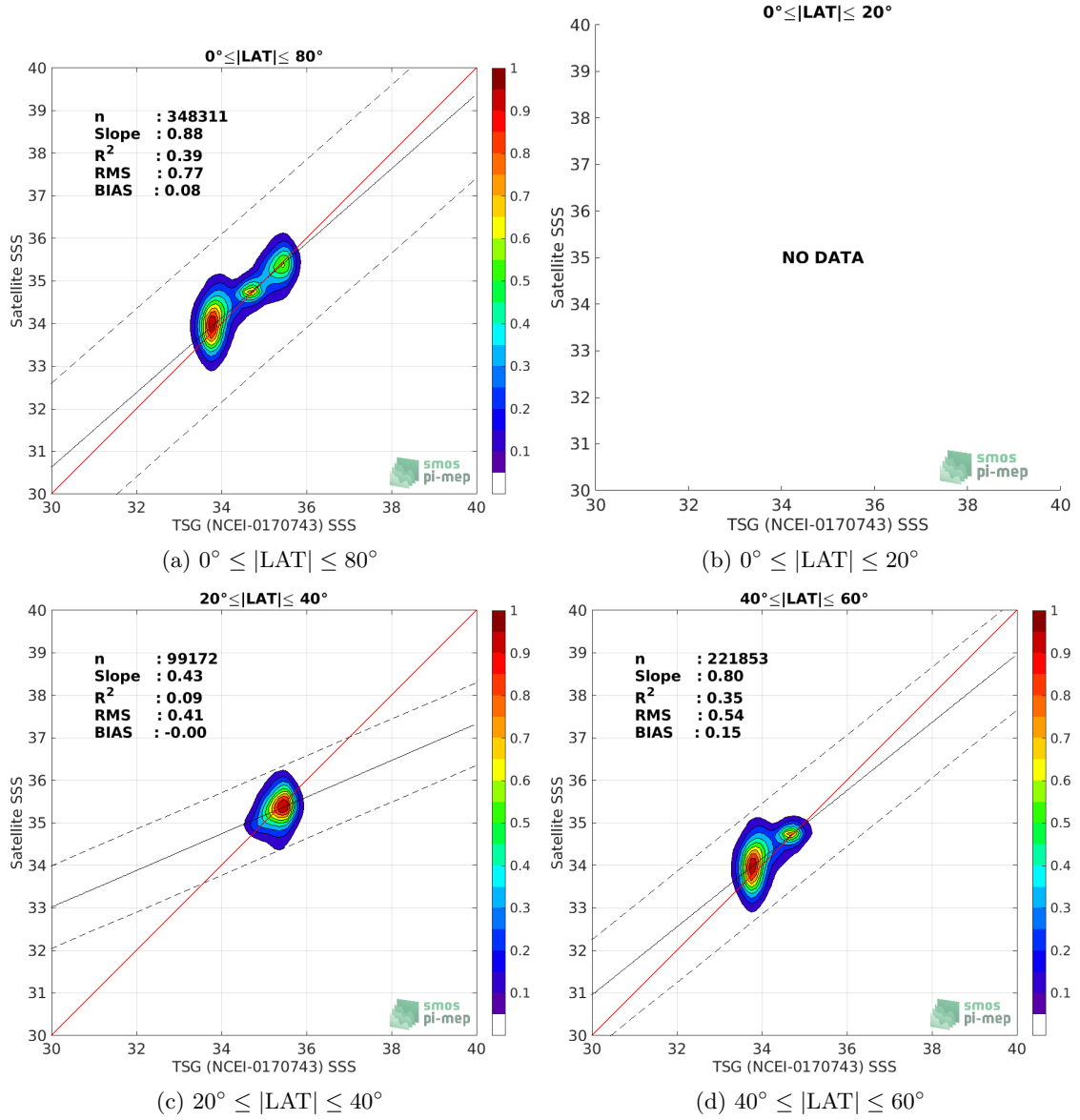
Figure 9: Contour maps of the concentration of SMOS SSS L3 v2 - Monthly - 0.25 Deg (CATDS-CECOS-IFREMER) SSS (y-axis) versus TSG (NCEI-0170743) SSS (x-axis) at match-up pairs for different latitude bands. For each plot, the red line shows x=y . The black thin and dashed lines indicate a linear fit through the data cloud and the \pm 95\% confidence levels, respectively. The number match-up pairs n , the slope and R^2 coefficient of the linear fit, the root mean square (RMS) and the mean bias between satellite and in situ data are indicated for each latitude band in each plots.
