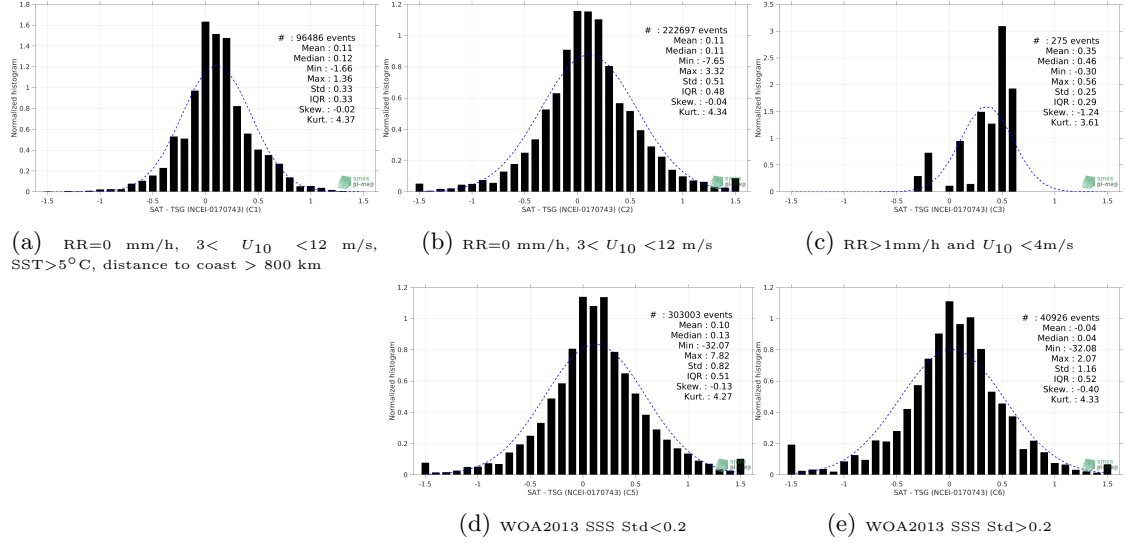
Figure 13: Normalized histogram of \Delta SSS (SMOS SSS L3 v2 - Monthly - 0.25 Deg (CATDS-CECOS-IFREMER) - TSG (NCEI-0170743)) for 5 different subdatasets corresponding to: RR=0 mm/h, 3 < U_{10} < 12 m/s, SST > 5°C, distance to coast > 800 km (a), RR=0 mm/h, 3 < U_{10} < 12 m/s (b), RR > 1mm/h and U_{10} < 4 m/s (c), WOA2013 SSS Std < 0.2 (d), WOA2013 SSS Std > 0.2 (e).
