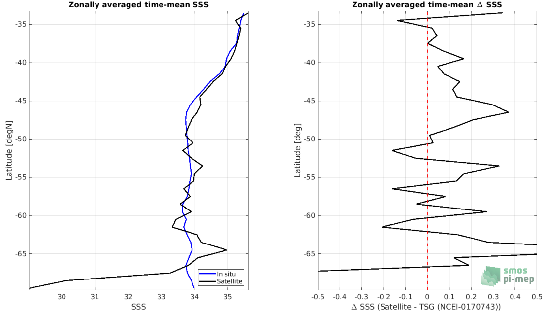
Figure 8: Left panel: Zonal mean SSS from SMOS SSS L3 v2 - Monthly - 0.25 Deg (CATDS-CECOS-IFREMER) satellite product (black) and from TSG (NCEI-0170743) (blue). Right panel: Zonal mean of \Delta SSS (Satellite - TSG (NCEI-0170743)) for all the collected Pi-MEP match-up pairs estimated over the full satellite product period.
