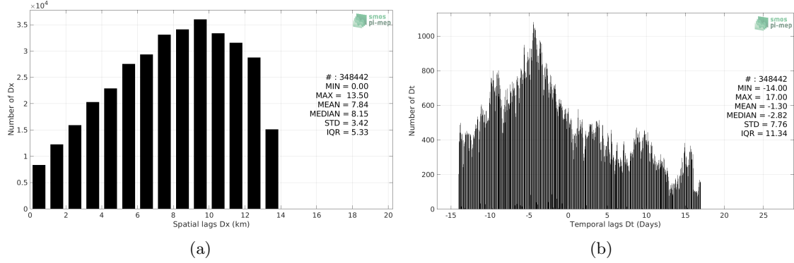
Figure 5: Histograms of the spatial (a) and temporal (b) lags between the location/time of the TSG (NCEI-0170743) measurement and the date of the corresponding SMOS SSS L3 v2 - Monthly - 0.25 Deg (CATDS-CECOS-IFREMER) SSS pixel.
