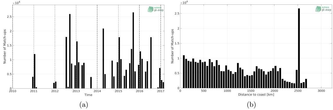
Figure 1: Number of match-ups between TSG (NCEI-0170743) and SMOS SSS L3 v2 - Monthly - 0.25 Deg (CATDS-CECOS-IFREMER) SSS as a function of time (a) and as function of the distance to coast (b) over the Global Ocean Pi-MEP region and for the full satellite product period.
