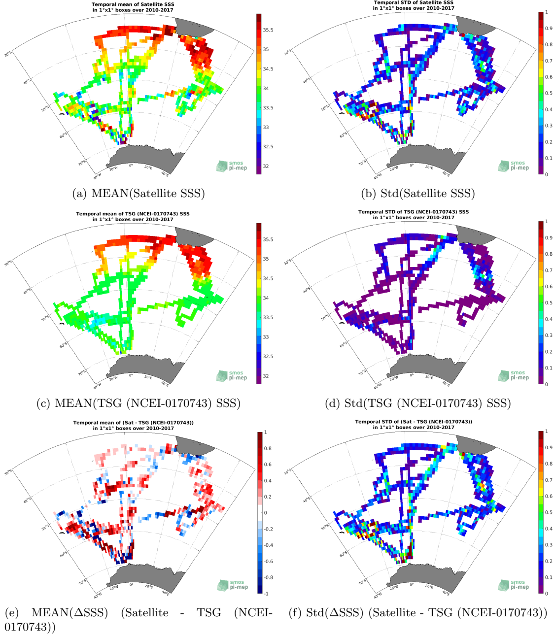
Figure 6: Temporal mean (left) and Std (right) of SSS from SMOS SSS L3 v2 - Monthly - 0.25 Deg (CATDS-CECOS-IFREMER) (top), TSG (NCEI-0170743) (middle), and of \Delta SSS (Satellite - TSG (NCEI-0170743)). Only match-up pairs are used to generate these maps.
