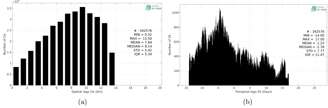
Figure 5: Histograms of the spatial (a) and temporal (b) lags between the time of the TSG (NCEI-0170743) measurements and the date of the corresponding SMOS SSS L3 v2 - Monthly - 0.25 Deg (CATDS-CECOS-IFREMER) SSS product.
