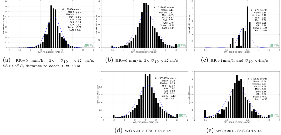
Figure 13: Normalized histogram of \Delta SSS (SMOS-L3-CATDS-IFREMER-CECOS-V2-MONTHLY-0.25DEG - TSG-NCEI-0170743) for 5 different subdatasets corresponding to: RR=0 mm/h, 3 < U_{10} < 12 m/s, SST>5°C, distance to coast > 800 km (a), RR=0 mm/h, 3 < U_{10} < 12 m/s (b), RR>1mm/h and U_{10} < 4 m/s (c), WOA2013 SSS Std<0.2 (d), WOA2013 SSS Std>0.2 (e).
