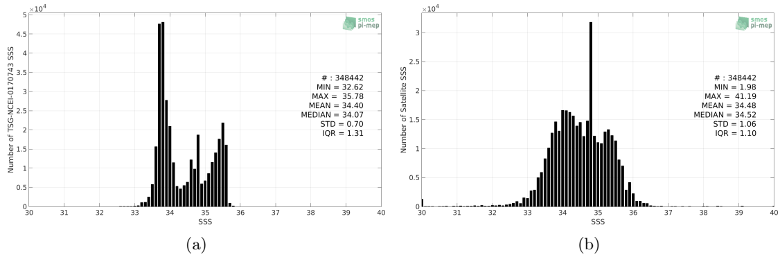
Figure 2: Histograms of SSS from TSG-NCEI-0170743 (a) and SMOS-L3-CATDS-IFREMER-CECOS-V2-MONTHLY-0.25DEG (b) considering all match-up pairs per bins of 0.1 over the Global Ocean Pi-MEP region and for the full satellite product period.
