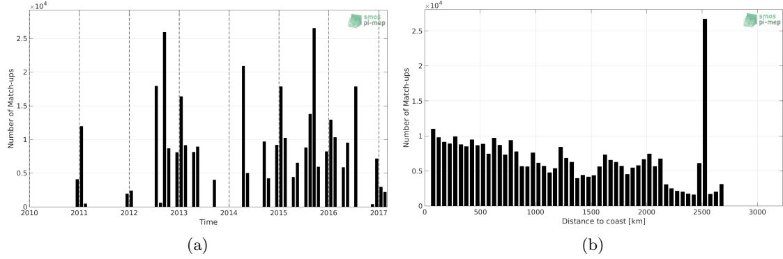
Figure 1: Number of match-ups between TSG-NCEI-0170743 and SMOS-L3-CATDS-IFREMER-CECOS-V2-MONTHLY-0.25DEG SSS as a function of time (a) and as function of the distance to coast (b) over the Global Ocean Pi-MEP region and for the full satellite product period.
