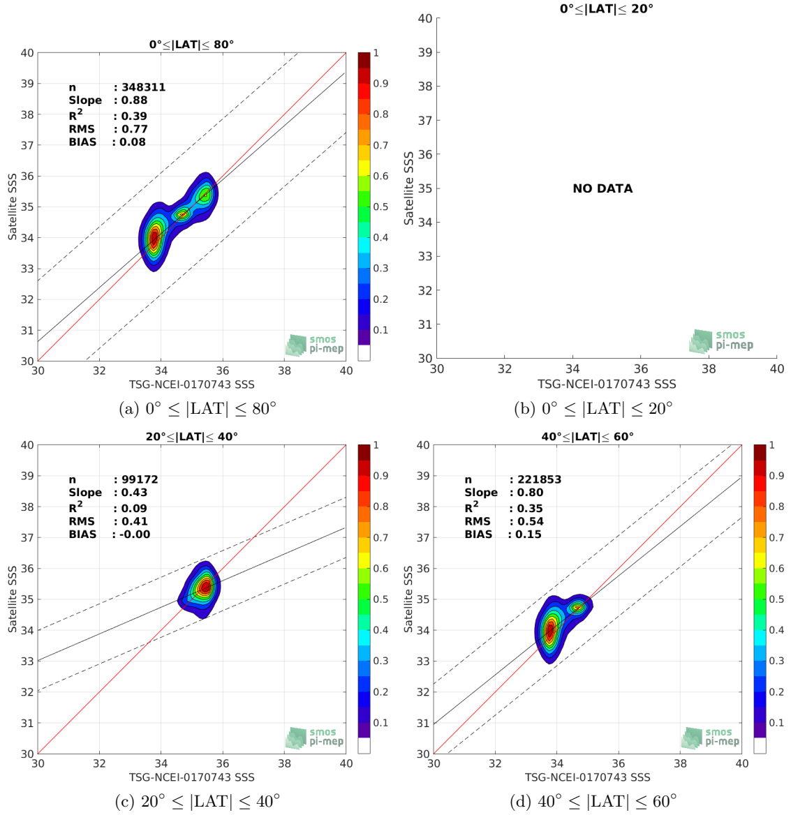
Figure 9: Contour maps of the concentration of SMOS-L3-CATDS-IFREMER-CECOS-V2-MONTHLY-0.25DEG SSS (y-axis) versus TSG-NCEI-0170743 SSS (x-axis) at match-up pairs for different latitude bands. For each plot, the red line shows x=y . The black thin and dashed lines indicate a linear fit through the data cloud and the \pm 95\% confidence levels, respectively. The number match-up pairs n , the slope and R^2 coefficient of the linear fit, the root mean square (RMS) and the mean bias between satellite and in situ data are indicated for each latitude band in each plots.
