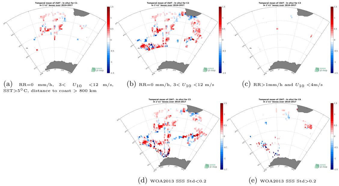
Figure 12: Temporal mean gridded over spatial boxes of size 1^\circ \times 1^\circ of \Delta SSS (SMOS-L3-CATDS-IFREMER-CECOS-V2-MONTHLY-0.25DEG - TSG-NCEI-0170743) for 5 different subdatasets corresponding to: RR=0 mm/h, 3 < U_{10} < 12 m/s, SST >5^\circ\text{C} , distance to coast > 800 km (a), RR=0 mm/h, 3 < U_{10} < 12 m/s (b), RR >1 mm/h and U_{10} < 4 m/s (c), WOA2013 SSS Std <0.2 (d), WOA2013 SSS Std >0.2 (e).
