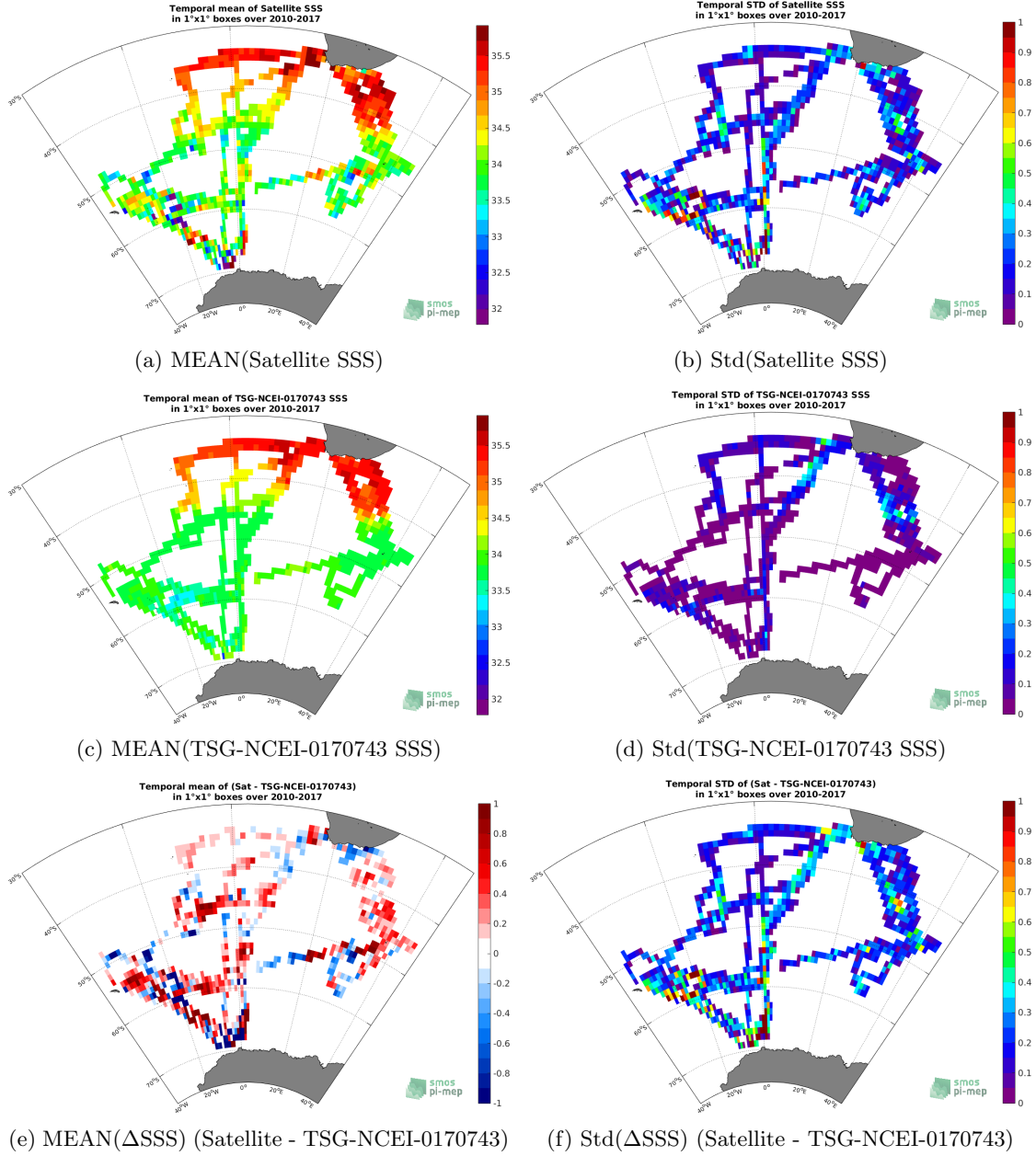
Figure 6: Temporal mean (left) and Std (right) of SSS from SMOS-L3-CATDS-IFREMER-CECOS-V2-MONTHLY-0.25DEG (top), TSG-NCEI-0170743 (middle), and of \Delta SSS (Satellite - TSG-NCEI-0170743). Only match-up pairs are used to generate these maps.
