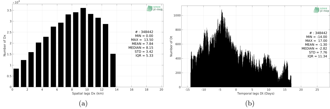
Figure 5: Histograms of the spatial (a) and temporal (b) lags between the time of the TSG-NCEI-0170743 measurements and the date of the corresponding SMOS-L3-CATDS-IFREMER-CECOS-V2-MONTHLY-0.25DEG SSS product.
