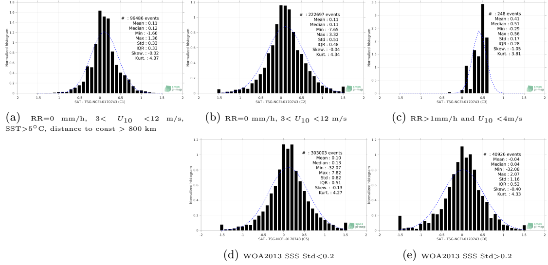
Figure 13: Normalized histogram of \Delta SSS (SMOS-L3-CATDS-IFREMER-CECOS-V2-MONTHLY-0.25DEG - TSG-NCEI-0170743) for 5 different subdatasets corresponding to: RR=0 mm/h, 3 < U_{10} < 12 m/s, SST > 5^\circ C , distance to coast > 800 km (a), RR=0 mm/h, 3 < U_{10} < 12 m/s (b), RR > 1 mm/h and U_{10} < 4 m/s (c), WOA2013 SSS Std < 0.2 (d), WOA2013 SSS Std > 0.2 (e).
