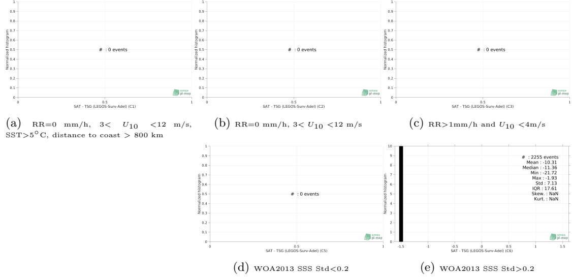
Figure 13: Normalized histogram of \Delta\text{SSS} (SMOS SSS L3 v2 - Monthly - 0.25 Deg (CATDS-CECOS-IFREMER) - TSG (LEGOS-Surv-Adel)) for 5 different subdatasets corresponding to: RR=0 mm/h, 3 < U_{10} < 12 m/s, SST > 5^{\circ}\text{C} , distance to coast > 800 km (a), RR=0 mm/h, 3 < U_{10} < 12 m/s (b), RR > 1\text{mm/h} and U_{10} < 4\text{m/s} (c), WOA2013 SSS Std < 0.2 (d), WOA2013 SSS Std > 0.2 (e).
