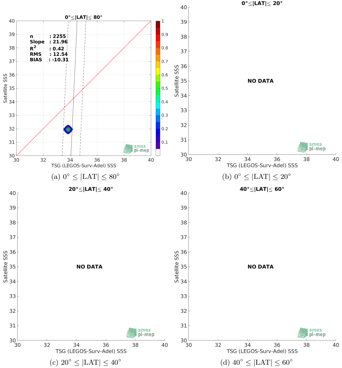
Figure 9: Contour maps of the concentration of SMOS SSS L3 v2 - Monthly - 0.25 Deg (CATDS-CECOS-IFREMER) SSS (y-axis) versus TSG (LEGOS-Surv-Adel) SSS (x-axis) at match-up pairs for different latitude bands. For each plot, the red line shows x=y . The black thin and dashed lines indicate a linear fit through the data cloud and the \pm 95\% confidence levels, respectively. The number match-up pairs n , the slope and R^2 coefficient of the linear fit, the root mean square (RMS) and the mean bias between satellite and in situ data are indicated for each latitude band in each plots.
