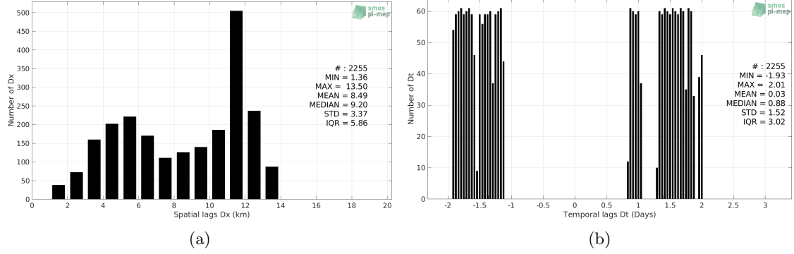
Figure 5: Histograms of the spatial (a) and temporal (b) lags between the location/time of the TSG (LEGOS-Surv-Adel) measurement and the date of the corresponding SMOS SSS L3 v2 - Monthly - 0.25 Deg (CATDS-CECOS-IFREMER) SSS pixel.
