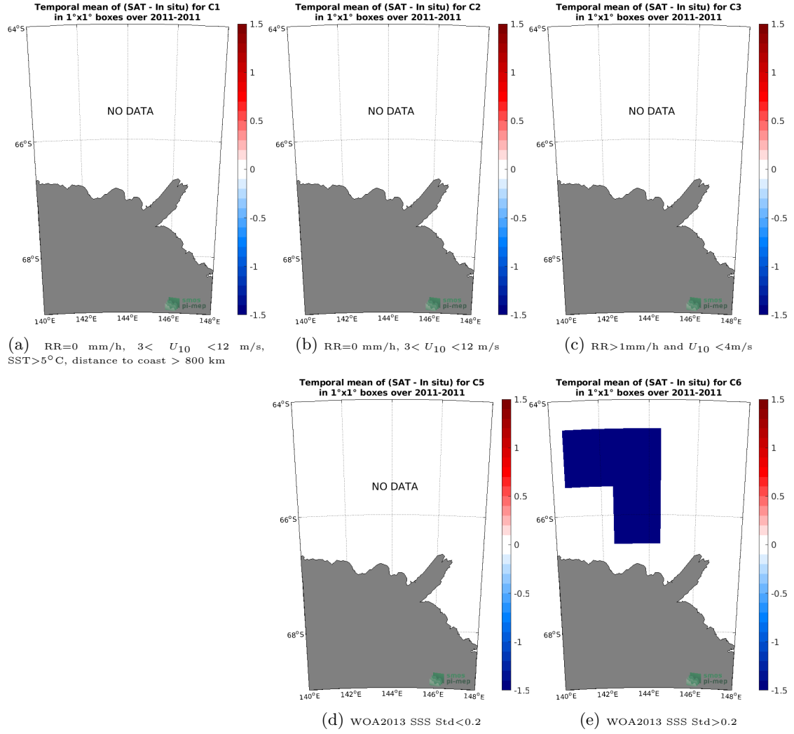
Figure 12: Temporal mean gridded over spatial boxes of size 1°x1° of \Delta SSS (SMOS SSS L3 v2 - Monthly - 0.25 Deg (CATDS-CECOS-IFREMER) - TSG (LEGOS-Surv-Adel)) for 5 different subdatasets corresponding to: RR=0 mm/h, 3 < U_{10} < 12 m/s, SST>5°C, distance to coast > 800 km (a), RR=0 mm/h, 3 < U_{10} < 12 m/s (b), RR>1mm/h and U_{10} < 4 m/s (c), WOA2013 SSS Std<0.2 (d), WOA2013 SSS Std>0.2 (e).
