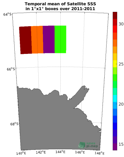
(a) MEAN(Satellite SSS)
