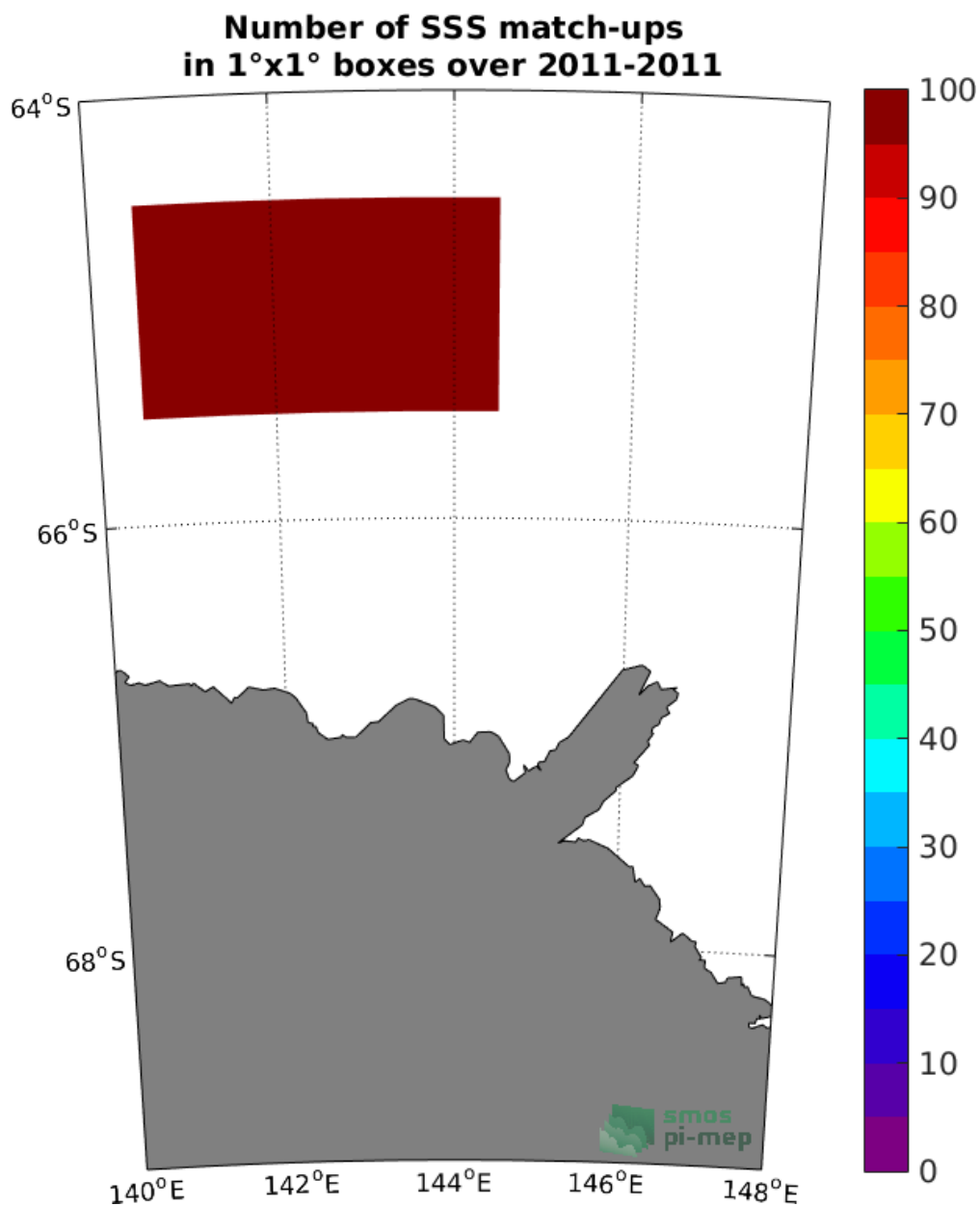
Figure 4: Number of SSS match-ups between TSG (LEGOS-Surv-Adel) SSS and the SMOS SSS L3 v2 - Monthly - 0.25 Deg (CATDS-CECOS-IFREMER) SSS product for the Global Ocean Pi-MEP region over 1°x1° boxes and for the full satellite product period.
