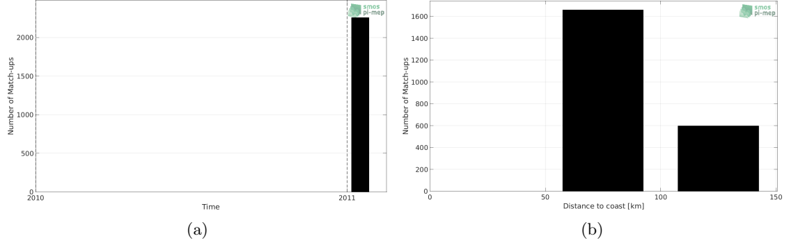
Figure 1: Number of match-ups between TSG (LEGOS-Surv-Adel) and SMOS SSS L3 v2 - Monthly - 0.25 Deg (CATDS-CECOS-IFREMER) SSS as a function of time (a) and as function of the distance to coast (b) over the Global Ocean Pi-MEP region and for the full satellite product period.
