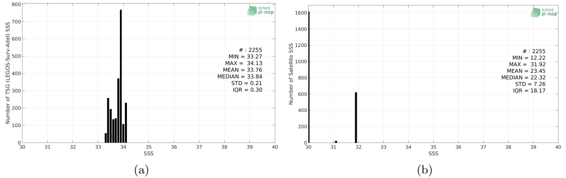
Figure 2: Histograms of SSS from TSG (LEGOS-Surv-Adel) (a) and SMOS SSS L3 v2 - Monthly - 0.25 Deg (CATDS-CECOS-IFREMER) (b) considering all match-up pairs per bins of 0.1 over the Global Ocean Pi-MEP region and for the full satellite product period.
