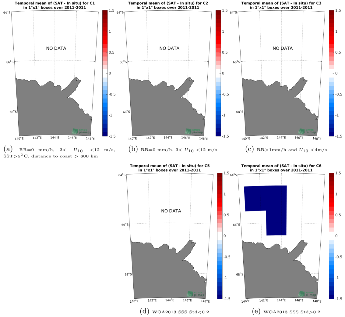
Figure 12: Temporal mean gridded over spatial boxes of size 1°x1° of \Delta\text{SSS} (SMOS SSS L3 v2 - Monthly - 0.25 Deg (CATDS-CECOS-IFREMER) - TSG (LEGOS-Surv-Adel)) for 5 different subdatasets corresponding to: RR=0 mm/h, 3 < U_{10} < 12 m/s, SST > 5^\circ\text{C} , distance to coast > 800 km (a), RR=0 mm/h, 3 < U_{10} < 12 m/s (b), RR > 1 mm/h and U_{10} < 4 m/s (c), WOA2013 SSS Std < 0.2 (d), WOA2013 SSS Std > 0.2 (e).
