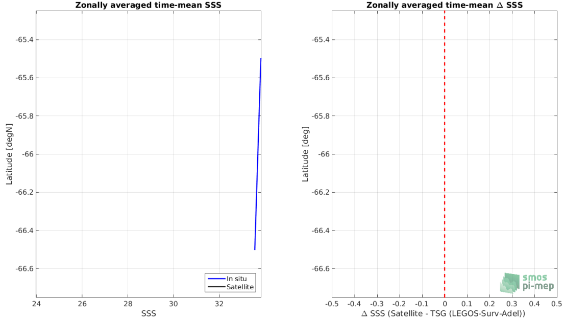
Figure 8: Left panel: Zonal mean SSS from SMOS SSS L3 v2 - Monthly - 0.25 Deg (CATDS-CECOS-IFREMER) satellite product (black) and from TSG (LEGOS-Surv-Adel) (blue). Right panel: Zonal mean of \Delta SSS (Satellite - TSG (LEGOS-Surv-Adel)) for all the collected Pi-MEP match-up pairs estimated over the full satellite product period.
