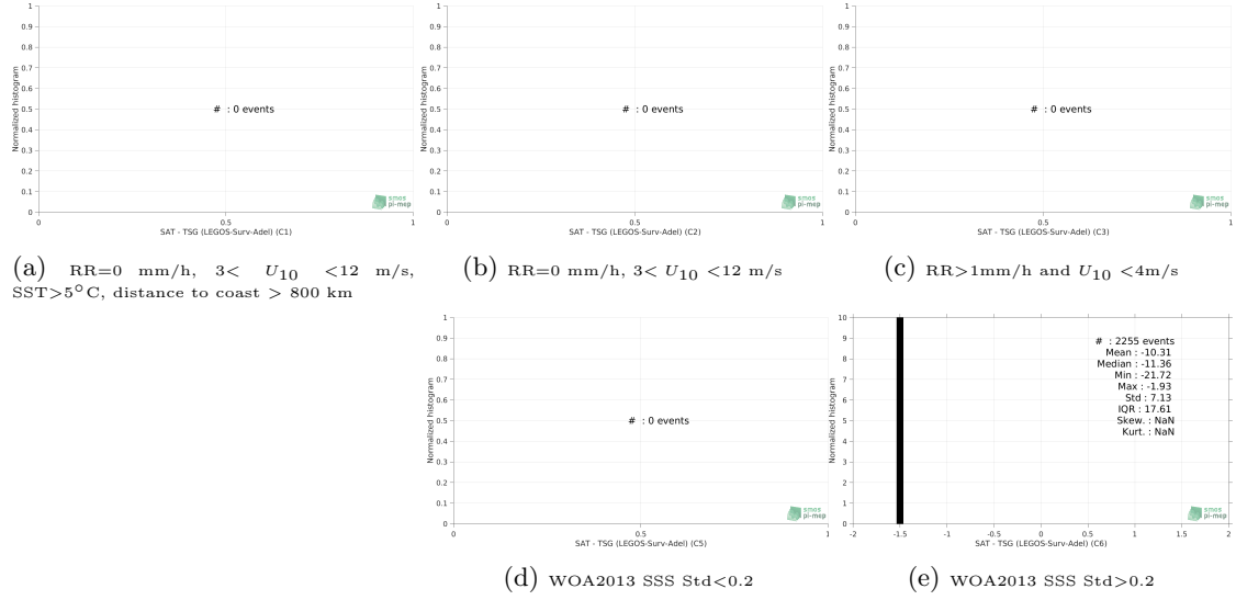
Figure 13: Normalized histogram of \Delta\text{SSS} (SMOS SSS L3 v2 - Monthly - 0.25 Deg (CATDS-CECOS-IFREMER) - TSG (LEGOS-Surv-Adel)) for 5 different subdatasets corresponding to: RR=0 mm/h, 3 < U_{10} < 12 m/s, SST > 5^\circ\text{C} , distance to coast > 800 km (a), RR=0 mm/h, 3 < U_{10} < 12 m/s (b), RR > 1\text{mm/h} and U_{10} < 4\text{m/s} (c), WOA2013 SSS Std <0.2 (d), WOA2013 SSS Std >0.2 (e).
