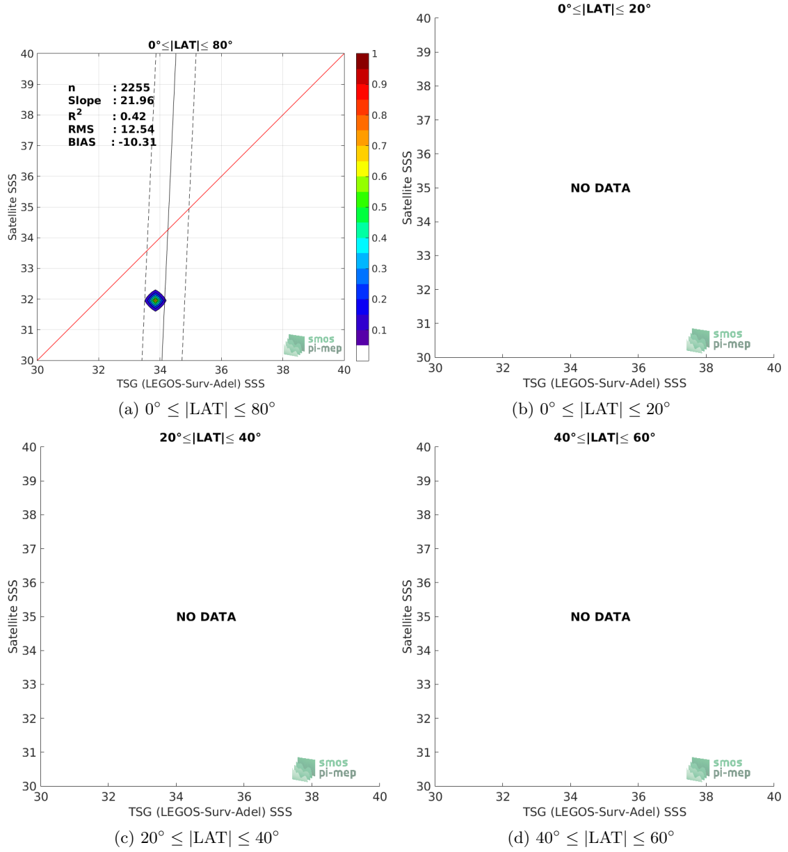
Figure 9: Contour maps of the concentration of SMOS SSS L3 v2 - Monthly - 0.25 Deg (CATDS-CECOS-IFREMER) SSS (y-axis) versus TSG (LEGOS-Surv-Adel) SSS (x-axis) at match-up pairs for different latitude bands. For each plot, the red line shows x=y . The black thin and dashed lines indicate a linear fit through the data cloud and the \pm 95\% confidence levels, respectively. The number match-up pairs n , the slope and R^2 coefficient of the linear fit, the root mean square (RMS) and the mean bias between satellite and in situ data are indicated for each latitude band in each plots.
