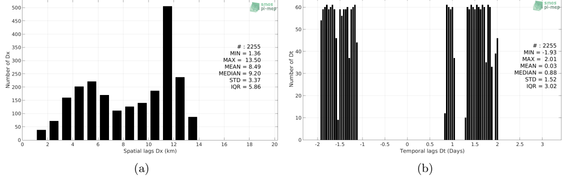
Figure 5: Histograms of the spatial (a) and temporal (b) lags between the time of the TSG (LEGOS-Surv-Adel) measurements and the date of the corresponding SMOS SSS L3 v2 - Monthly - 0.25 Deg (CATDS-CECOS-IFREMER) SSS product.
