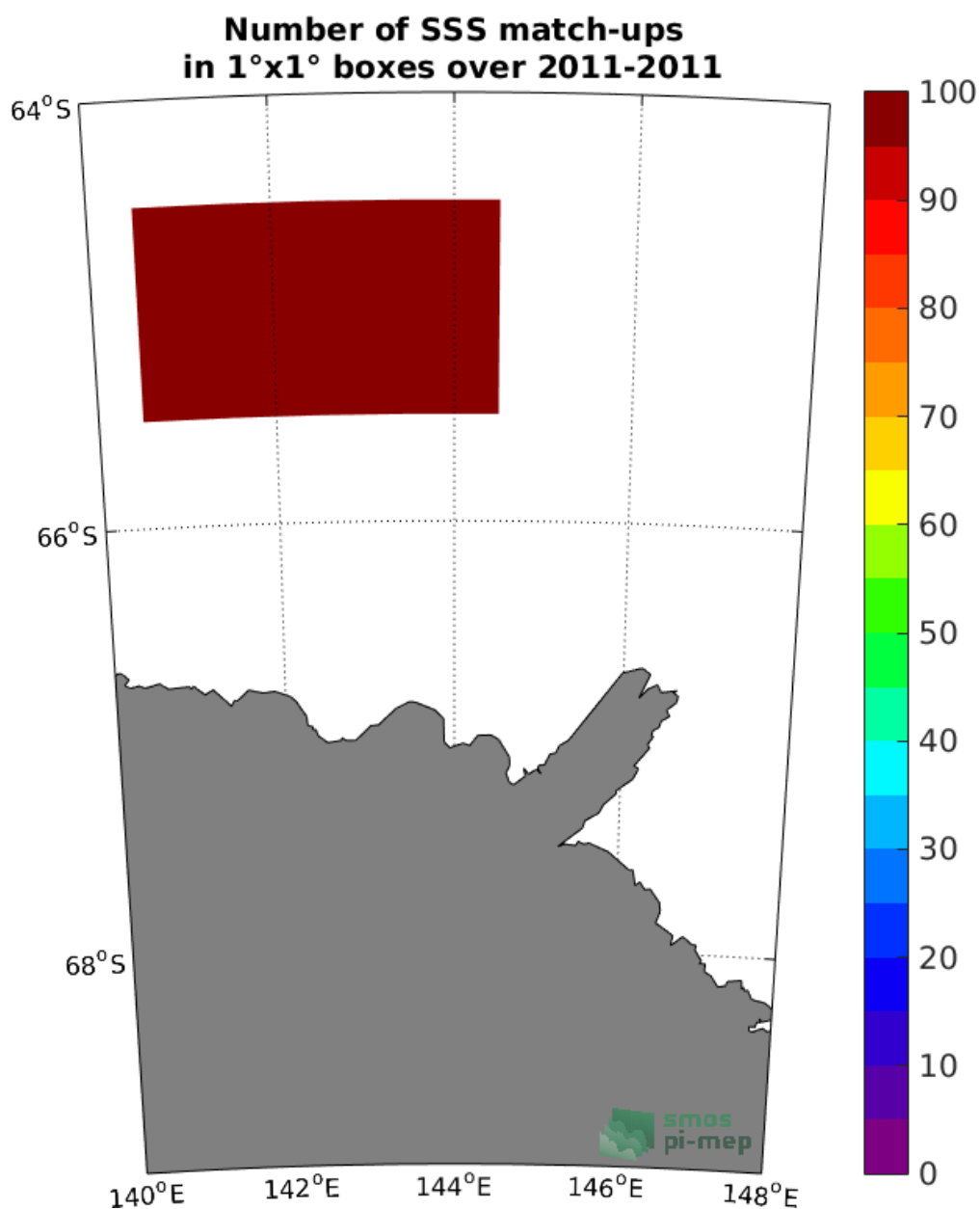
Figure 4: Number of SSS match-ups between TSG-LEGOS-Surv-Adel SSS and the SMOS L3 v2 - Monthly - 0.25 Deg (CATDS-CECOS-IFREMER) SSS product for the Global Ocean Pi-MEP region over 1°x1° boxes and for the full satellite product period.
