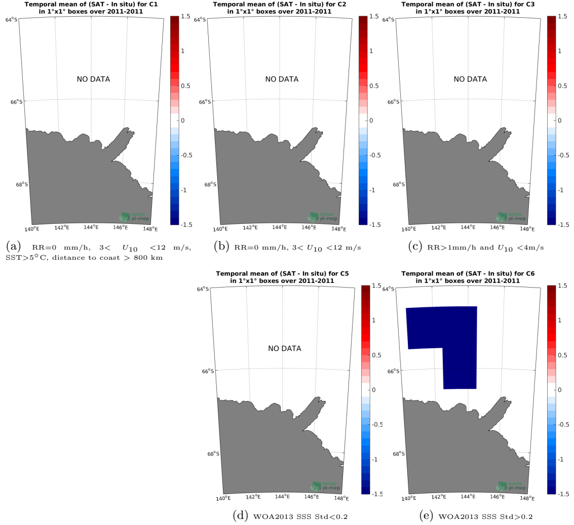
Figure 12: Temporal mean gridded over spatial boxes of size 1^{\circ} \times 1^{\circ} of \Delta\text{SSS} (SMOS L3 v2 - Monthly - 0.25 Deg (CATDS-CECOS-IFREMER) - TSG-LEGOS-Surv-Adel) for 5 different subdatasets corresponding to: RR=0 mm/h, 3 < U_{10} < 12 m/s, SST > 5^{\circ}\text{C} , distance to coast > 800 km (a), RR=0 mm/h, 3 < U_{10} < 12 m/s (b), RR > 1 mm/h and U_{10} < 4 m/s (c), WOA2013 SSS Std < 0.2 (d), WOA2013 SSS Std > 0.2 (e).
