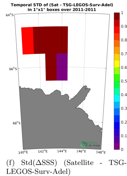
Figure 6: Temporal mean (left) and Std (right) of SSS from SMOS L3 v2 - Monthly - 0.25 Deg (CATDS-CECOS-IFREMER) (top), TSG-LEGOS-Surv-Adel (middle), and of \Delta SSS (Satellite - TSG-LEGOS-Surv-Adel). Only match-up pairs are used to generate these maps.
