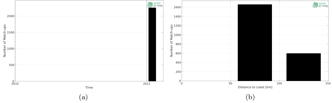
Figure 1: Number of match-ups between TSG-LEGOS-Surv-Adel and SMOS L3 v2 - Monthly - 0.25 Deg (CATDS-CECOS-IFREMER) SSS as a function of time (a) and as function of the distance to coast (b) over the Global Ocean Pi-MEP region and for the full satellite product period.
