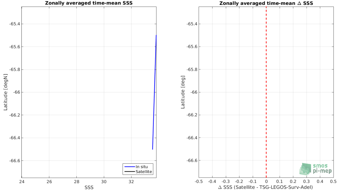
Figure 8: Left panel: Zonal mean SSS from SMOS L3 v2 - Monthly - 0.25 Deg (CATDS-CECOS-IFREMER) satellite product (black) and from TSG-LEGOS-Surv-Adel (blue). Right panel: Zonal mean of \Delta SSS (Satellite - TSG-LEGOS-Surv-Adel) for all the collected Pi-MEP match-up pairs estimated over the full satellite product period.
