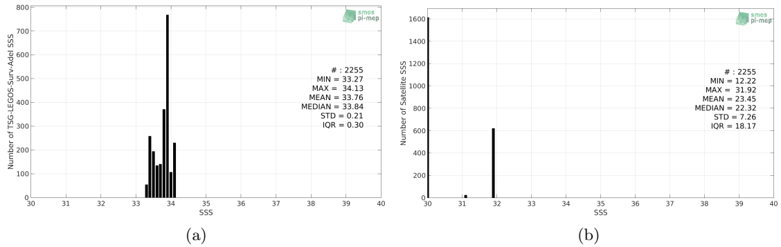
Figure 2: Histograms of SSS from TSG-LEGOS-Surv-Adel (a) and SMOS L3 v2 - Monthly - 0.25 Deg (CATDS-CECOS-IFREMER) (b) considering all match-up pairs per bins of 0.1 over the Global Ocean Pi-MEP region and for the full satellite product period.
