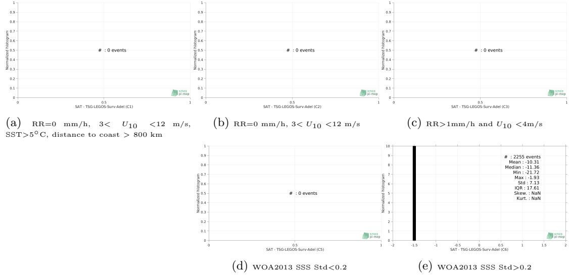
Figure 13: Normalized histogram of \Delta SSS (SMOS L3 v2 - Monthly - 0.25 Deg (CATDS-CECOS-IFREMER) - TSG-LEGOS-Surv-Adel) for 5 different subdatasets corresponding to: RR=0 mm/h, 3 < U_{10} < 12 m/s, SST>5°C, distance to coast > 800 km (a), RR=0 mm/h, 3 < U_{10} < 12 m/s (b), RR>1 mm/h and U_{10} < 4 m/s (c), WOA2013 SSS Std<0.2 (d), WOA2013 SSS Std>0.2 (e).
