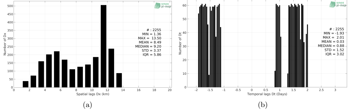
Figure 5: Histograms of the spatial (a) and temporal (b) lags between the time of the TSG-LEGOS-Surv-Adel measurements and the date of the corresponding SMOS L3 v2 - Monthly - 0.25 Deg (CATDS-CECOS-IFREMER) SSS product.
