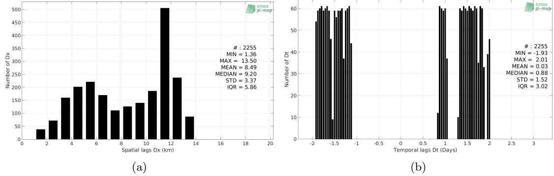
Figure 5: Histograms of the spatial (a) and temporal (b) lags between the time of the TSG-LEGOS-Surv-Adel measurements and the date of the corresponding SMOS-L3-CATDS-IFREMER-CECOS-V2-MONTHLY-0.25DEG SSS product.
