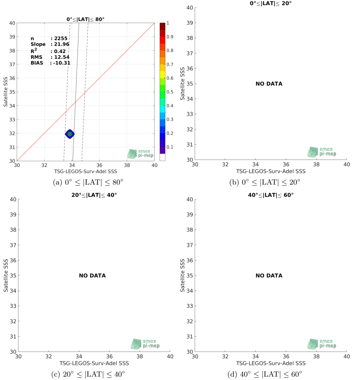
Figure 9: Contour maps of the concentration of SMOS-L3-CATDS-IFREMER-CECOS-V2-MONTHLY-0.25DEG SSS (y-axis) versus TSG-LEGOS-Surv-Adel SSS (x-axis) at match-up pairs for different latitude bands. For each plot, the red line shows x=y . The black thin and dashed lines indicate a linear fit through the data cloud and the \pm 95\% confidence levels, respectively. The number match-up pairs n , the slope and R^2 coefficient of the linear fit, the root mean square (RMS) and the mean bias between satellite and in situ data are indicated for each latitude band in each plots.
