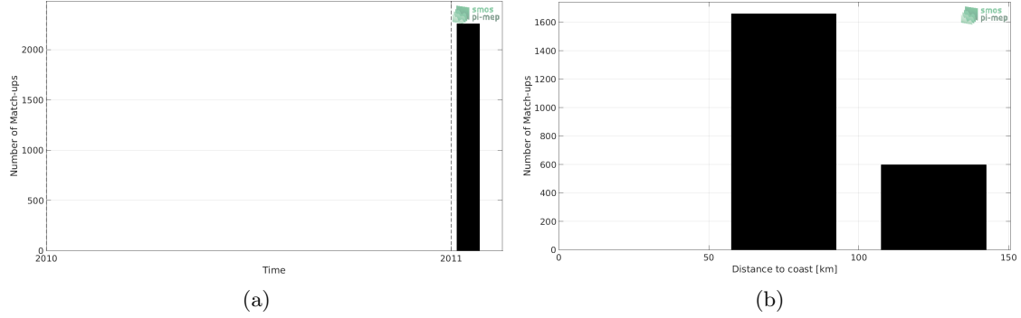
Figure 1: Number of match-ups between TSG-LEGOS-Surv-Adel and SMOS-L3-CATDS-IFREMER-CECOS-V2-MONTHLY-0.25DEG SSS as a function of time (a) and as function of the distance to coast (b) over the Global Ocean Pi-MEP region and for the full satellite product period.
