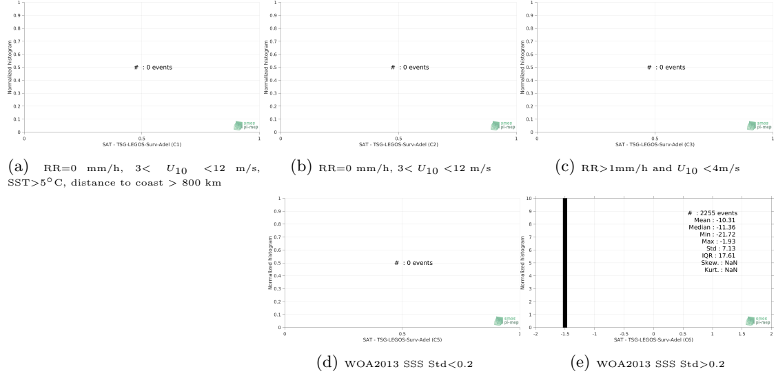
Figure 13: Normalized histogram of \Delta\text{SSS} (SMOS-L3-CATDS-IFREMER-CECOS-V2-MONTHLY-0.25DEG - TSG-LEGOS-Surv-Adel) for 5 different subdatasets corresponding to: RR=0 mm/h, 3 < U_{10} < 12 m/s, SST > 5^\circ\text{C} , distance to coast > 800 km (a), RR=0 mm/h, 3 < U_{10} < 12 m/s (b), RR > 1\text{mm/h} and U_{10} < 4\text{m/s} (c), WOA2013 SSS Std < 0.2 (d), WOA2013 SSS Std > 0.2 (e).
