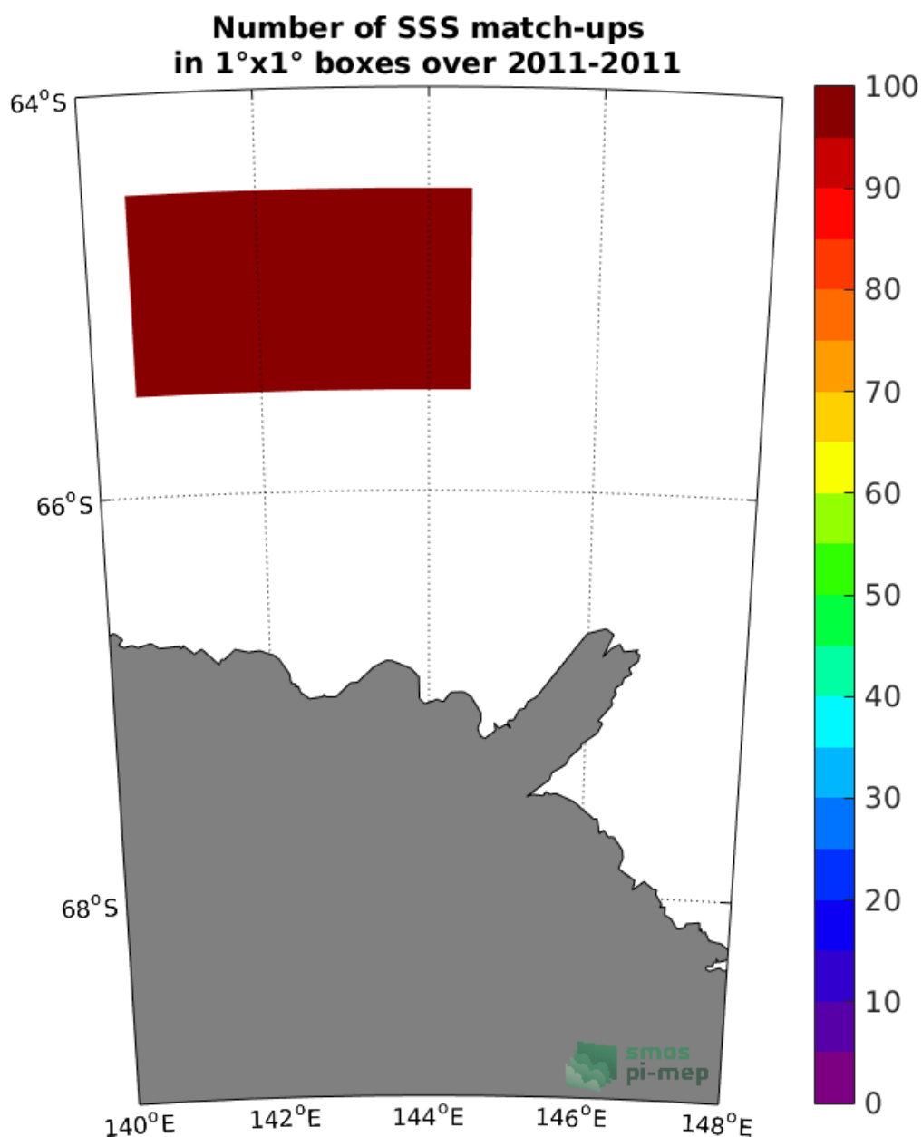
Figure 4: Number of SSS match-ups between TSG-LEGOS-Surv-Adel SSS and the SMOS-L3-CATDS-IFREMER-CECOS-V2-MONTHLY-0.25DEG SSS product for the Global Ocean Pi-MEP region over 1°x1° boxes and for the full satellite product period.
