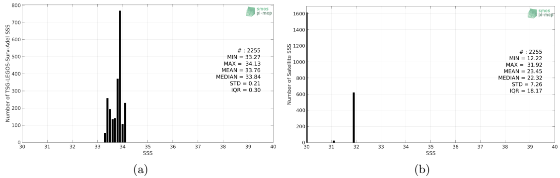
Figure 2: Histograms of SSS from TSG-LEGOS-Surv-Adel (a) and SMOS-L3-CATDS-IFREMER-CECOS-V2-MONTHLY-0.25DEG (b) considering all match-up pairs per bins of 0.1 over the Global Ocean Pi-MEP region and for the full satellite product period.
