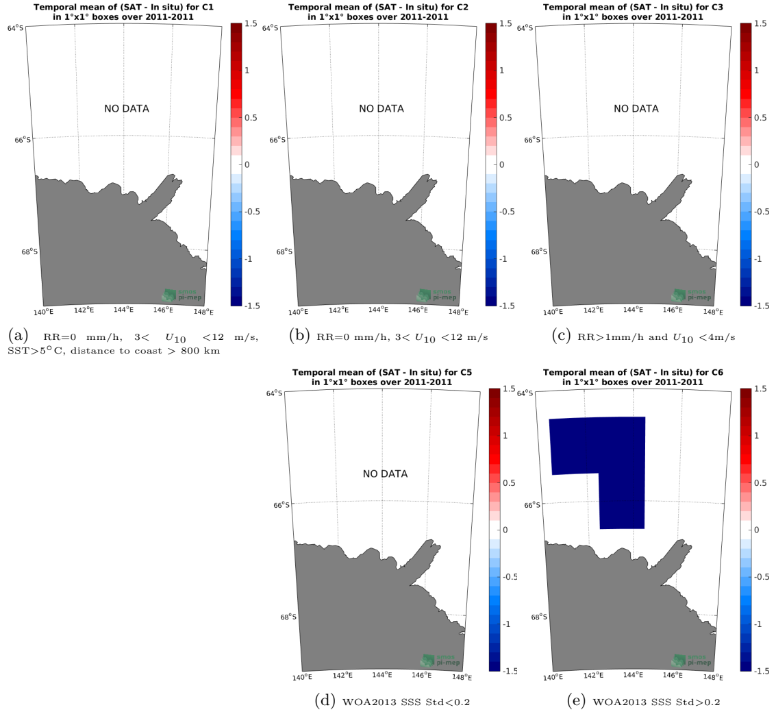
Figure 12: Temporal mean gridded over spatial boxes of size 1^\circ \times 1^\circ of \Delta SSS (SMOS-L3-CATDS-IFREMER-CECOS-V2-MONTHLY-0.25DEG - TSG-LEGOS-Surv-Adel) for 5 different subdatasets corresponding to:RR=0 mm/h, 3 < U_{10} < 12 m/s, SST >5^\circ\text{C} , distance to coast > 800 km (a), RR=0 mm/h, 3 < U_{10} < 12 m/s (b), RR >1 mm/h and U_{10} < 4 m/s (c), WOA2013 SSS Std <0.2 (d), WOA2013 SSS Std >0.2 (e).
