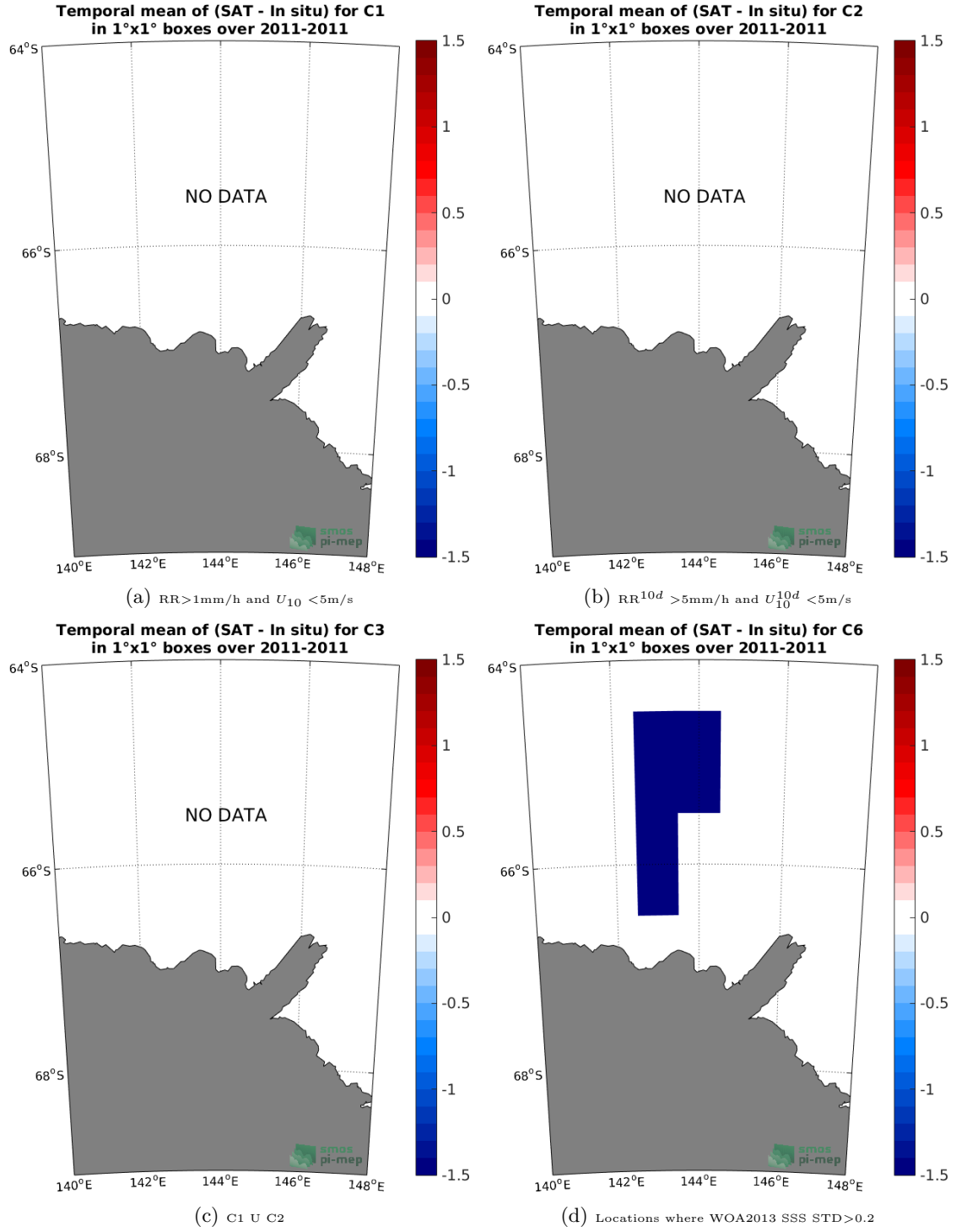
Figure 12: Temporal mean gridded over spatial boxes of size 1^\circ \times 1^\circ of \Delta\text{SSS} (SMOS-L3-CATDS-IFREMER-CECOS-V2-MONTHLY-0.25DEG - TSG-LEGOS-Surv-Adel) for 4 different subdatasets corresponding to: RR > 1\text{mm/h} and U_{10} < 5\text{m/s} (a), RR^{10d} > 5\text{mm/h} and U_{10}^{10d} < 5\text{m/s} (b), C1 U C2 (c), Locations where WOA2013 SSS STD > 0.2 (d).
