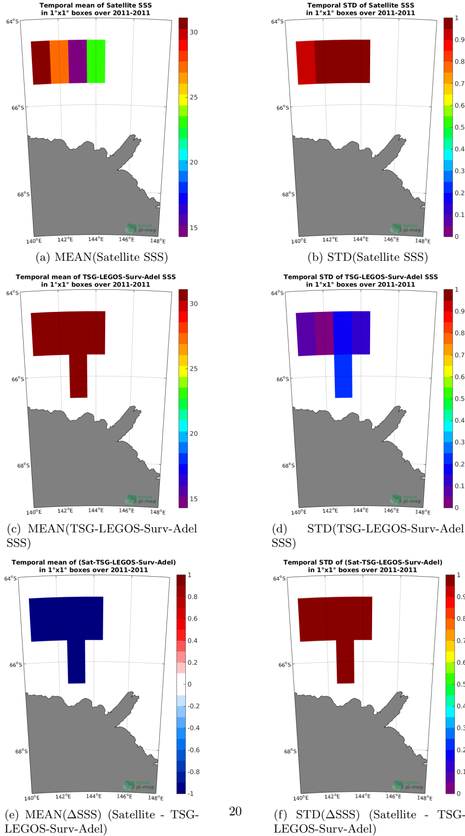
Figure 6: Temporal mean (left) and STD (right) of SSS from SMOS-L3-CATDS-IFREMER-CECOS-V2-MONTHLY-0.25DEG (top), TSG-LEGOS-Surv-Adel (middle), and of \Delta SSS (Satellite - TSG-LEGOS-Surv-Adel). Only match-up pairs are used to generate these maps.
