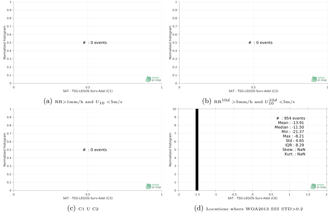
Figure 13: Normalized histogram of \Delta SSS (SMOS-L3-CATDS-IFREMER-CECOS-V2-MONTHLY-0.25DEG - TSG-LEGOS-Surv-Adel) for 6 different subdatasets corresponding to: RR > 1\text{mm/h} and U_{10} < 5\text{m/s} (a), RR^{10d} > 5\text{mm/h} and U_{10}^{10d} < 5\text{m/s} (b), C1 \cup C2 (c), Locations where WOA2013 SSS STD > 0.2 (d).
