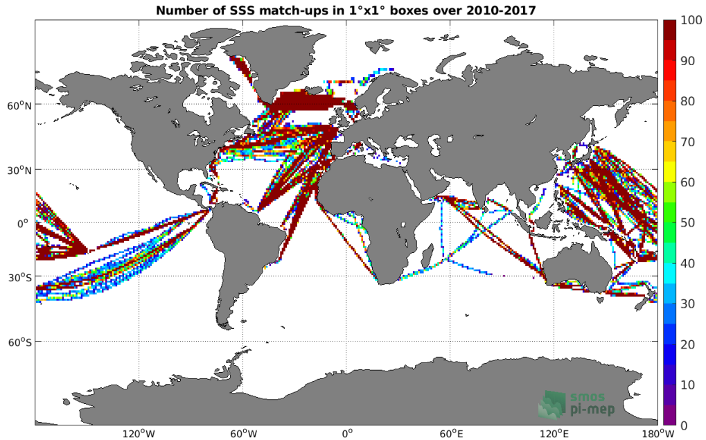
Figure 4: Number of SSS match-ups between TSG (LEGOS-DM) SSS and the SMOS SSS L3 v2 - Monthly - 0.25 Deg (CATDS-CECOS-IFREMER) SSS product for the Global Ocean Pi-MEP region over 1^\circ \times 1^\circ boxes and for the full satellite product period.
