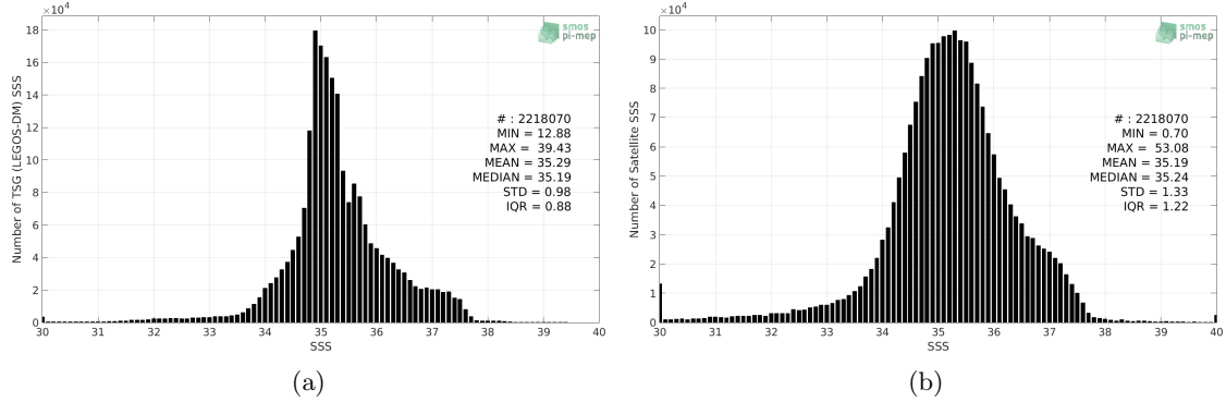
Figure 2: Histograms of SSS from TSG (LEGOS-DM) (a) and SMOS SSS L3 v2 - Monthly - 0.25 Deg (CATDS-CECOS-IFREMER) (b) considering all match-up pairs per bins of 0.1 over the Global Ocean Pi-MEP region and for the full satellite product period.
