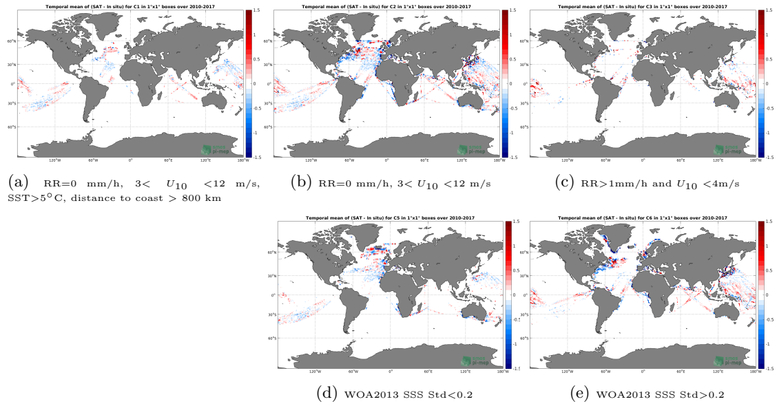
Figure 12: Temporal mean gridded over spatial boxes of size 1^\circ \times 1^\circ of \Delta SSS (SMOS SSS L3 v2 - Monthly - 0.25 Deg (CATDS-CECOS-IFREMER) - TSG (LEGOS-DM)) for 5 different subdatasets corresponding to:RR=0 mm/h, 3 < U_{10} < 12 m/s, SST>5°C, distance to coast > 800 km (a), RR=0 mm/h, 3 < U_{10} < 12 m/s (b), RR>1mm/h and U_{10} < 4 m/s (c), WOA2013 SSS Std<0.2 (d), WOA2013 SSS Std>0.2 (e).
