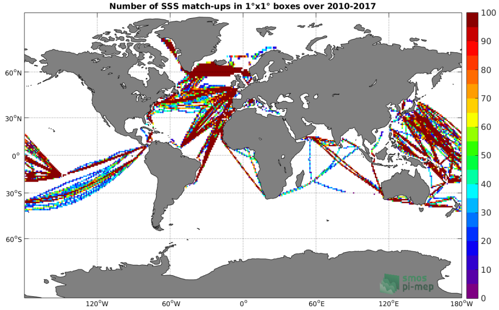
Figure 4: Number of SSS match-ups between TSG (LEGOS-DM) SSS and the SMOS SSS L3 v2 - Monthly - 0.25 Deg (CATDS-CECOS-IFREMER) SSS product for the Global Ocean Pi-MEP region over 1^\circ \times 1^\circ boxes and for the full satellite product period.
