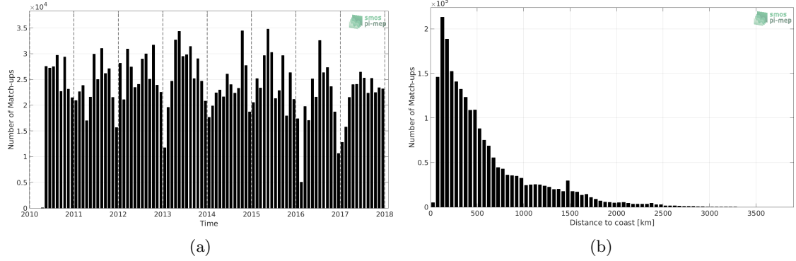
Figure 1: Number of match-ups between TSG (LEGOS-DM) and SMOS SSS L3 v2 - Monthly - 0.25 Deg (CATDS-CECOS-IFREMER) SSS as a function of time (a) and as function of the distance to coast (b) over the Global Ocean Pi-MEP region and for the full satellite product period.
