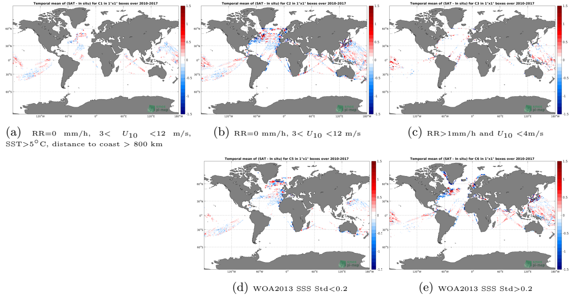
Figure 12: Temporal mean gridded over spatial boxes of size 1^\circ \times 1^\circ of \Delta SSS (SMOS L3 v2 - Monthly - 0.25 Deg (CATDS-CECOS-IFREMER) - TSG-LEGOS-DM) for 5 different subdatasets corresponding to:RR=0 mm/h, 3 < U_{10} < 12 m/s, SST >5^\circ\text{C} , distance to coast > 800 km (a), RR=0 mm/h, 3 < U_{10} < 12 m/s (b), RR >1 mm/h and U_{10} < 4 m/s (c), WOA2013 SSS Std <0.2 (d), WOA2013 SSS Std >0.2 (e).
