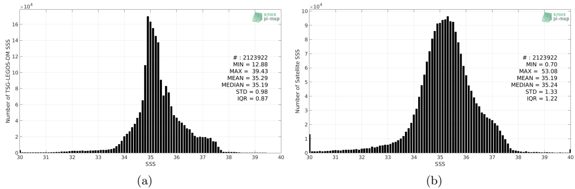
Figure 2: Histograms of SSS from TSG-LEGOS-DM (a) and SMOS L3 v2 - Monthly - 0.25 Deg (CATDS-CECOS-IFREMER) (b) considering all match-up pairs per bins of 0.1 over the Global Ocean Pi-MEP region and for the full satellite product period.
