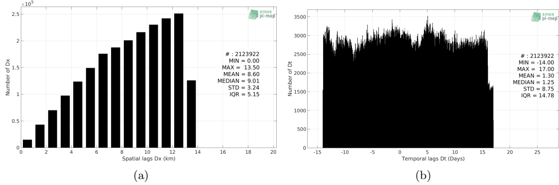
Figure 5: Histograms of the spatial (a) and temporal (b) lags between the time of the TSG-LEGOS-DM measurements and the date of the corresponding SMOS L3 v2 - Monthly - 0.25 Deg (CATDS-CECOS-IFREMER) SSS product.
