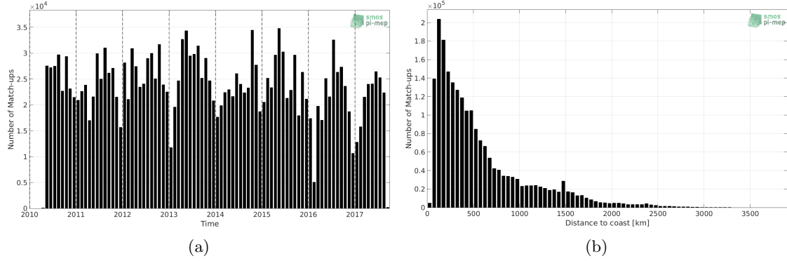
Figure 1: Number of match-ups between TSG-LEGOS-DM and SMOS L3 v2 - Monthly - 0.25 Deg (CATDS-CECOS-IFREMER) SSS as a function of time (a) and as function of the distance to coast (b) over the Global Ocean Pi-MEP region and for the full satellite product period.
