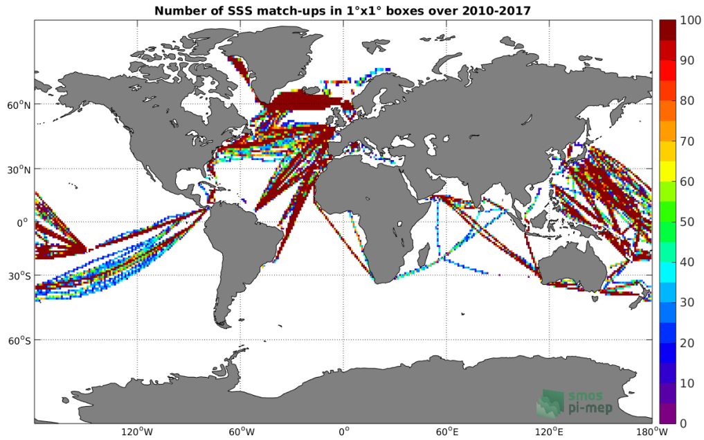
Figure 4: Number of SSS match-ups between TSG-LEGOS-DM SSS and the SMOS L3 v2 - Monthly - 0.25 Deg (CATDS-CECOS-IFREMER) SSS product for the Global Ocean Pi-MEP region over 1°x1° boxes and for the full satellite product period.
