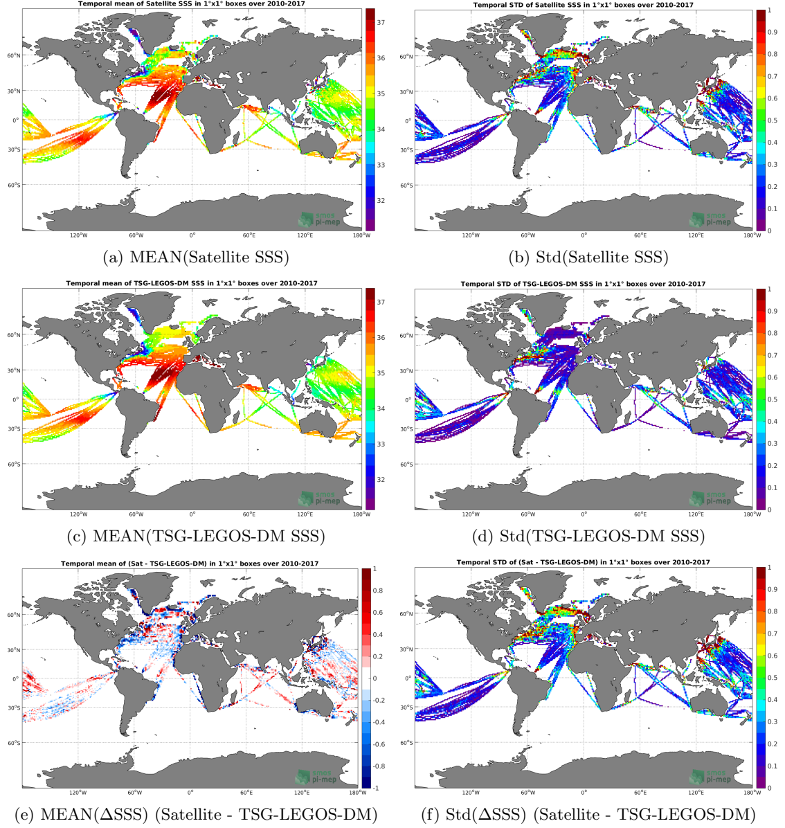
Figure 6: Temporal mean (left) and Std (right) of SSS from SMOS L3 v2 - Monthly - 0.25 Deg (CATDS-CECOS-IFREMER) (top), TSG-LEGOS-DM (middle), and of \Delta SSS (Satellite - TSG-LEGOS-DM). Only match-up pairs are used to generate these maps.
