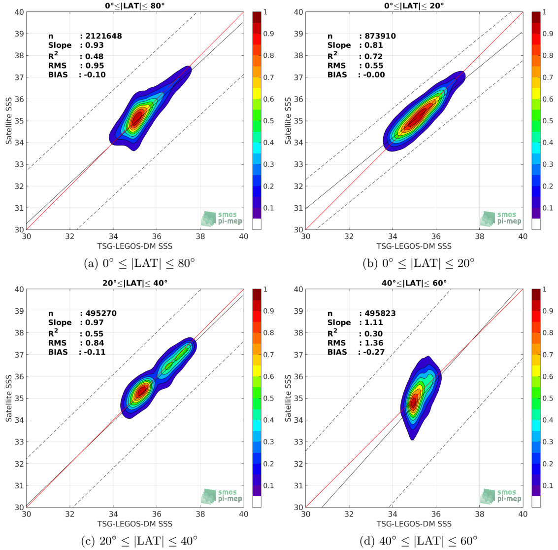
Figure 9: Contour maps of the concentration of SMOS L3 v2 - Monthly - 0.25 Deg (CATDS-CECOS-IFREMER) SSS (y-axis) versus TSG-LEGOS-DM SSS (x-axis) at match-up pairs for different latitude bands. For each plot, the red line shows x=y . The black thin and dashed lines indicate a linear fit through the data cloud and the \pm 95\% confidence levels, respectively. The number match-up pairs n , the slope and R^2 coefficient of the linear fit, the root mean square (RMS) and the mean bias between satellite and in situ data are indicated for each latitude band in each plots.
