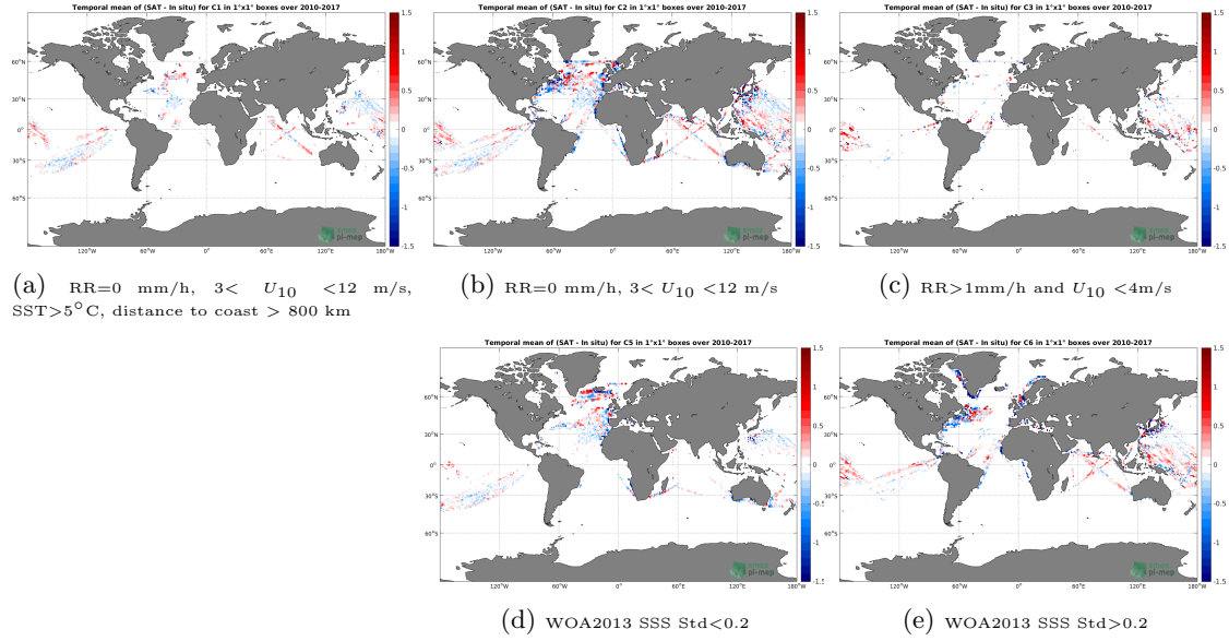
Figure 12: Temporal mean gridded over spatial boxes of size 1^\circ \times 1^\circ of \Delta SSS (SMOS-L3-CATDS-IFREMER-CECOS-V2-MONTHLY-0.25DEG - TSG-LEGOS-DM) for 5 different subdatasets corresponding to: RR=0 mm/h, 3 < U_{10} < 12 m/s, SST > 5^\circ C , distance to coast > 800 km (a), RR=0 mm/h, 3 < U_{10} < 12 m/s (b), RR > 1 mm/h and U_{10} < 4 m/s (c), WOA2013 SSS Std < 0.2 (d), WOA2013 SSS Std > 0.2 (e).
