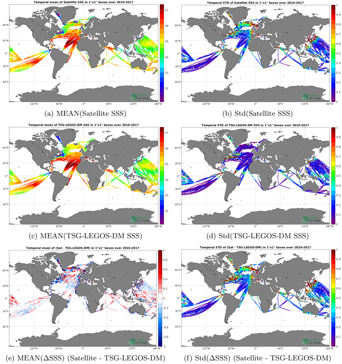
Figure 6: Temporal mean (left) and Std (right) of SSS from SMOS-L3-CATDS-IFREMER-CECOS-V2-MONTHLY-0.25DEG (top), TSG-LEGOS-DM (middle), and of \Delta SSS (Satellite - TSG-LEGOS-DM). Only match-up pairs are used to generate these maps.
