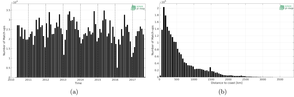
Figure 1: Number of match-ups between TSG-LEGOS-DM and SMOS-L3-CATDS-IFREMER-CECOS-V2-MONTHLY-0.25DEG SSS as a function of time (a) and as function of the distance to coast (b) over the Global Ocean Pi-MEP region and for the full satellite product period.
