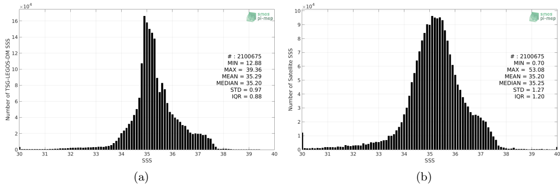
Figure 2: Histograms of SSS from TSG-LEGOS-DM (a) and SMOS-L3-CATDS-IFREMER-CECOS-V2-MONTHLY-0.25DEG (b) considering all match-up pairs per bins of 0.1 over the Global Ocean Pi-MEP region and for the full satellite product period.
