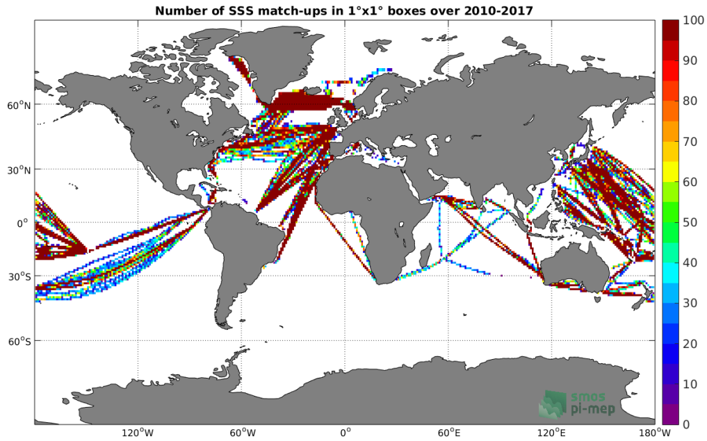
Figure 4: Number of SSS match-ups between TSG-LEGOS-DM SSS and the SMOS-L3-CATDS-IFREMER-CECOS-V2-MONTHLY-0.25DEG SSS product for the Global Ocean Pi-MEP region over 1°x1° boxes and for the full satellite product period.
