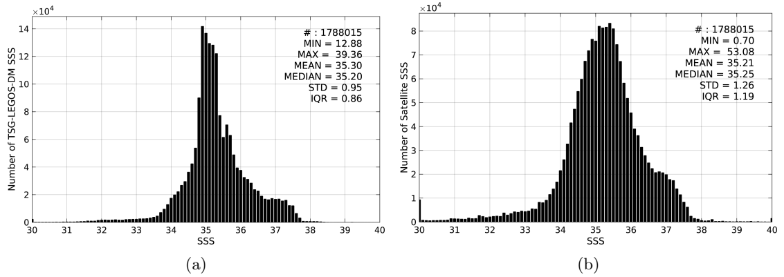
Figure 2: Histograms of SSS from TSG-LEGOS-DM (a) and SMOS-L3-CATDS-IFREMER-CECOS-V2-MONTHLY-0.25DEG (b) considering all match-up pairs per bins of 0.1 over the Global Ocean Pi-MEP region and for the full satellite product period.
