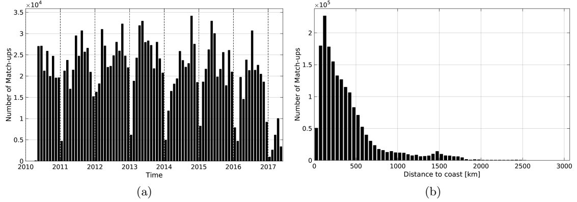
Figure 1: Number of match-ups between TSG-LEGOS-DM and SMOS-L3-CATDS-IFREMER-CECOS-V2-MONTHLY-0.25DEG SSS as a function of time (a) and as function of the distance to coast (b) over the Global Ocean Pi-MEP region and for the full satellite product period.
