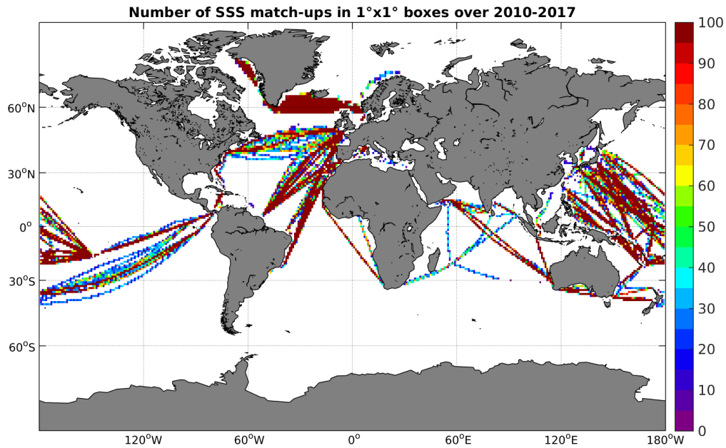
Figure 4: Number of SSS match-ups between TSG-LEGOS-DM SSS and the SMOS-L3-CATDS-IFREMER-CECOS-V2-MONTHLY-0.25DEG SSS product for the Global Ocean Pi-MEP region over 1^\circ \times 1^\circ boxes and for the full satellite product period.
