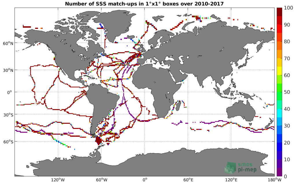
Figure 4: Number of SSS match-ups between TSG (GOSUD-Sailing-ship) SSS and the SMOS SSS L3 v2 - Monthly - 0.25 Deg (CATDS-CECOS-IFREMER) SSS product for the Global Ocean Pi-MEP region over 1^\circ \times 1^\circ boxes and for the full satellite product period.
