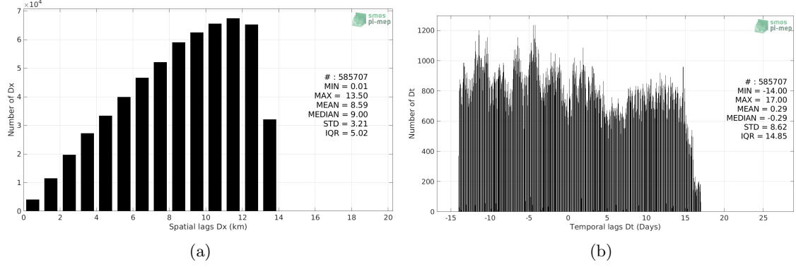
Figure 5: Histograms of the spatial (a) and temporal (b) lags between the location/time of the TSG (GOSUD-Sailing-ship) measurement and the date of the corresponding SMOS SSS L3 v2 - Monthly - 0.25 Deg (CATDS-CECOS-IFREMER) SSS pixel.
