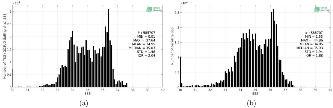
Figure 2: Histograms of SSS from TSG (GOSUD-Sailing-ship) (a) and SMOS SSS L3 v2 - Monthly - 0.25 Deg (CATDS-CECOS-IFREMER) (b) considering all match-up pairs per bins of 0.1 over the Global Ocean Pi-MEP region and for the full satellite product period.
