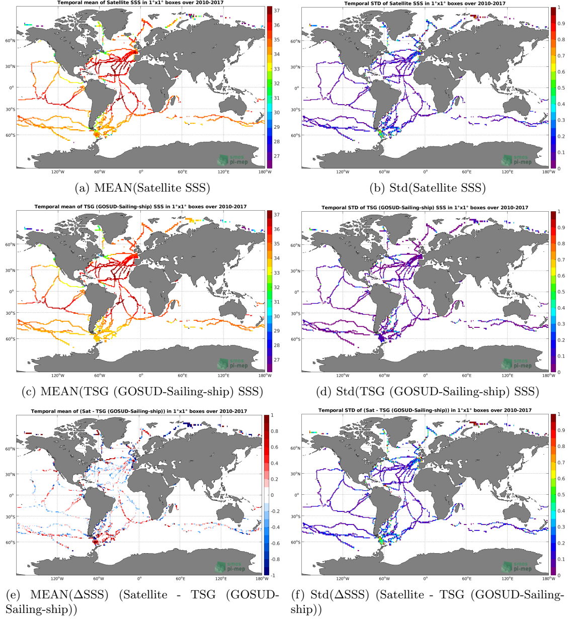
Figure 6: Temporal mean (left) and Std (right) of SSS from SMOS SSS L3 v2 - Monthly - 0.25 Deg (CATDS-CECOS-IFREMER) (top), TSG (GOSUD-Sailing-ship) (middle), and of \Delta SSS (Satellite - TSG (GOSUD-Sailing-ship)). Only match-up pairs are used to generate these maps.
