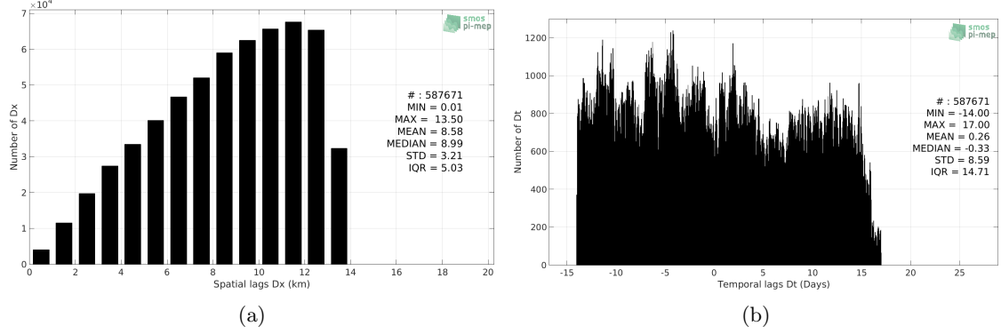
Figure 5: Histograms of the spatial (a) and temporal (b) lags between the time of the TSG (GOSUD-Sailing-ship) measurements and the date of the corresponding SMOS SSS L3 v2 - Monthly - 0.25 Deg (CATDS-CECOS-IFREMER) SSS product.
