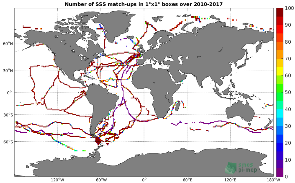
Figure 4: Number of SSS match-ups between TSG (GOSUD-Sailing-ship) SSS and the SMOS SSS L3 v2 - Monthly - 0.25 Deg (CATDS-CECOS-IFREMER) SSS product for the Global Ocean Pi-MEP region over 1°x1° boxes and for the full satellite product period.
