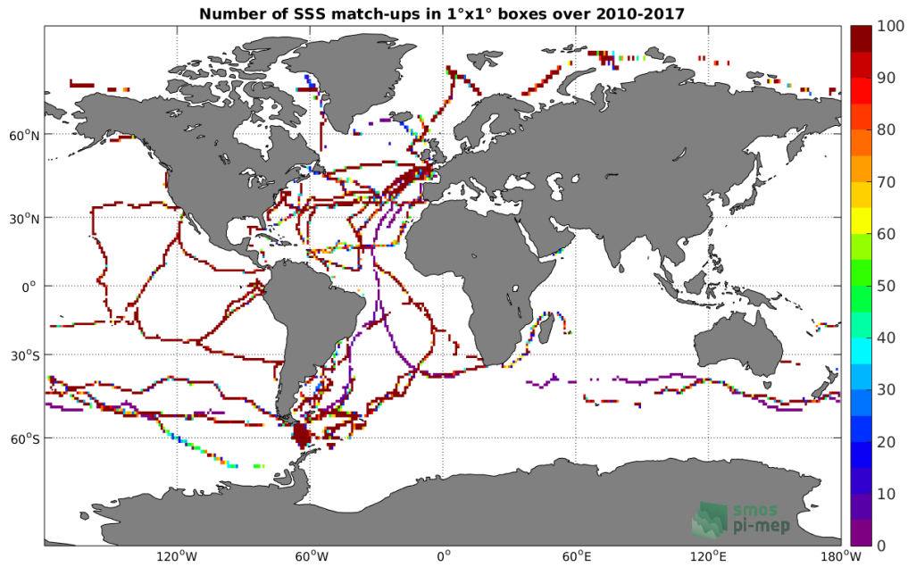
Figure 4: Number of SSS match-ups between TSG-GOSUD-Sailing-ship SSS and the SMOS L3 v2 - Monthly - 0.25 Deg (CATDS-CECOS-IFREMER) SSS product for the Global Ocean Pi-MEP region over 1°x1° boxes and for the full satellite product period.
