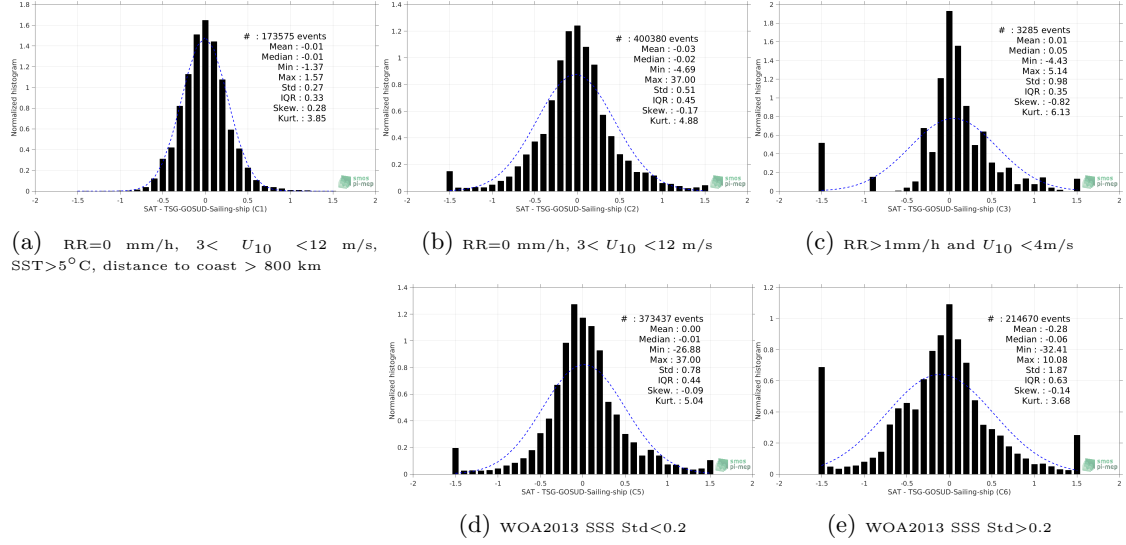
Figure 13: Normalized histogram of \Delta SSS (SMOS L3 v2 - Monthly - 0.25 Deg (CATDS-CECOS-IFREMER) - TSG-GOSUD-Sailing-ship) for 5 different subdatasets corresponding to: RR=0 mm/h, 3 < U_{10} < 12 m/s, SST>5°C, distance to coast > 800 km (a), RR=0 mm/h, 3 < U_{10} < 12 m/s (b), RR>1mm/h and U_{10} < 4 m/s (c), WOA2013 SSS Std<0.2 (d), WOA2013 SSS Std>0.2 (e).
