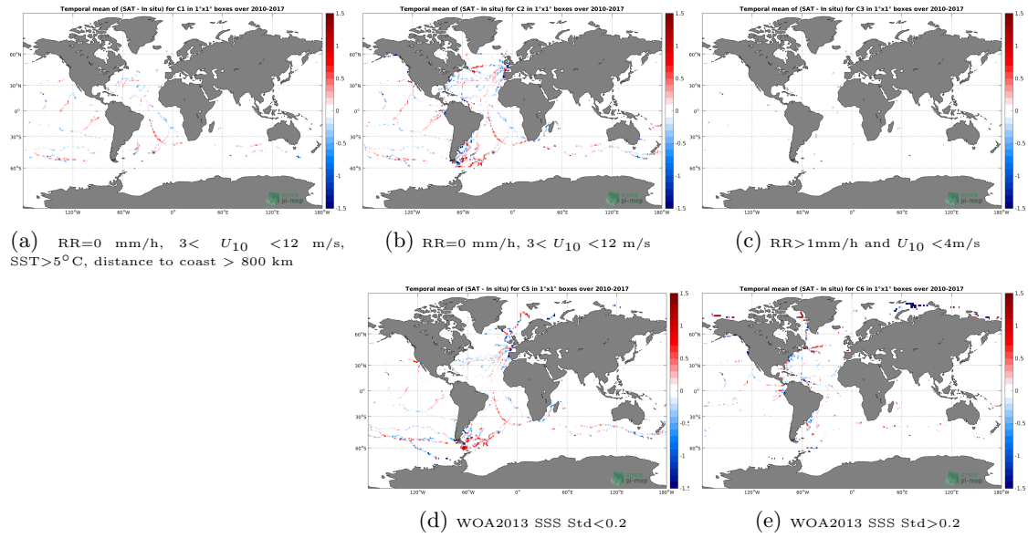
Figure 12: Temporal mean gridded over spatial boxes of size 1^\circ \times 1^\circ of \Delta SSS (SMOS L3 v2 - Monthly - 0.25 Deg (CATDS-CECOS-IFREMER) - TSG-GOSUD-Sailing-ship) for 5 different subdatasets corresponding to:RR=0 mm/h, 3 < U_{10} < 12 m/s, SST >5^\circ\text{C} , distance to coast > 800 km (a), RR=0 mm/h, 3 < U_{10} < 12 m/s (b), RR >1 mm/h and U_{10} < 4 m/s (c), WOA2013 SSS Std <0.2 (d), WOA2013 SSS Std >0.2 (e).
