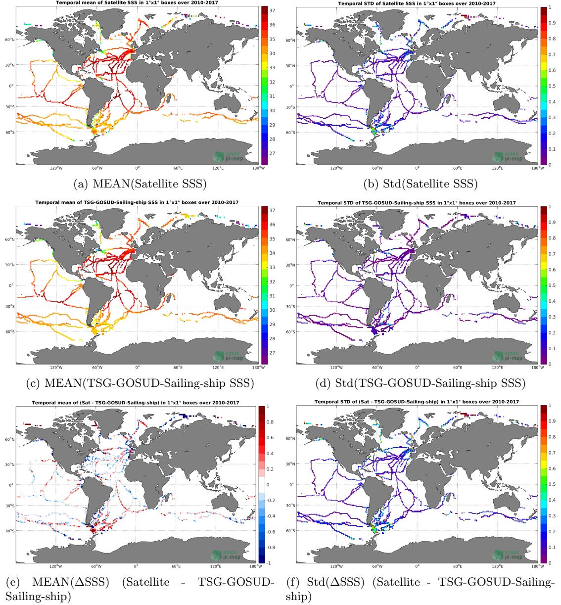
Figure 6: Temporal mean (left) and Std (right) of SSS from SMOS L3 v2 - Monthly - 0.25 Deg (CATDS-CECOS-IFREMER) (top), TSG-GOSUD-Sailing-ship (middle), and of \Delta SSS (Satellite - TSG-GOSUD-Sailing-ship). Only match-up pairs are used to generate these maps.
