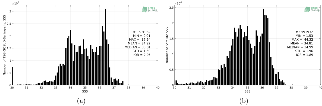
Figure 2: Histograms of SSS from TSG-GOSUD-Sailing-ship (a) and SMOS L3 v2 - Monthly - 0.25 Deg (CATDS-CECOS-IFREMER) (b) considering all match-up pairs per bins of 0.1 over the Global Ocean Pi-MEP region and for the full satellite product period.
