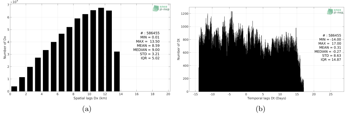
Figure 5: Histograms of the spatial (a) and temporal (b) lags between the time of the TSG-GOSUD-Sailing-ship measurements and the date of the corresponding SMOS-L3-CATDS-IFREMER-CECOS-V2-MONTHLY-0.25DEG SSS product.
