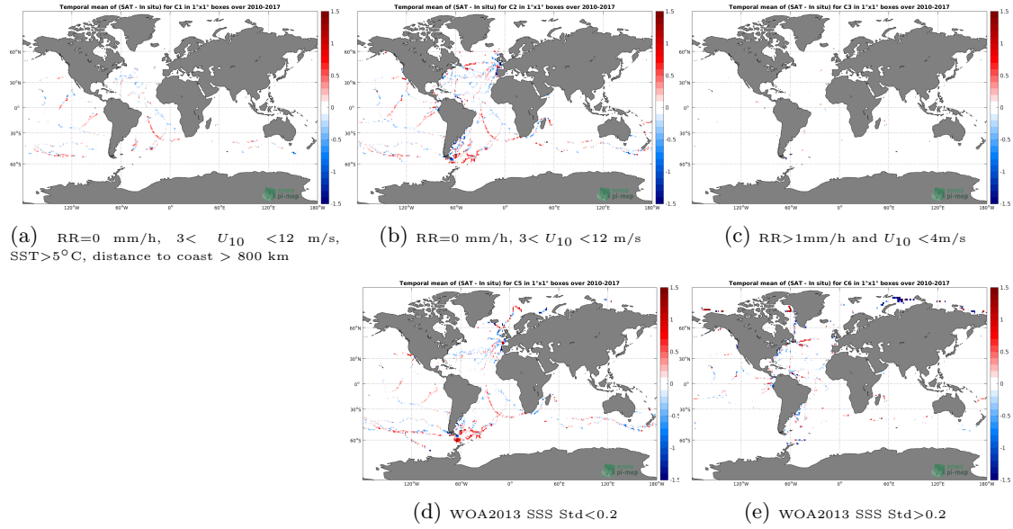
Figure 12: Temporal mean gridded over spatial boxes of size 1^\circ \times 1^\circ of \Delta SSS (SMOS-L3-CATDS-IFREMER-CECOS-V2-MONTHLY-0.25DEG - TSG-GOSUD-Sailing-ship) for 5 different sub-datasets corresponding to: RR=0 mm/h, 3 < U_{10} < 12 m/s, SST>5°C, distance to coast > 800 km (a), RR=0 mm/h, 3 < U_{10} < 12 m/s (b), RR>1mm/h and U_{10} < 4 m/s (c), WOA2013 SSS Std<0.2 (d), WOA2013 SSS Std>0.2 (e).
