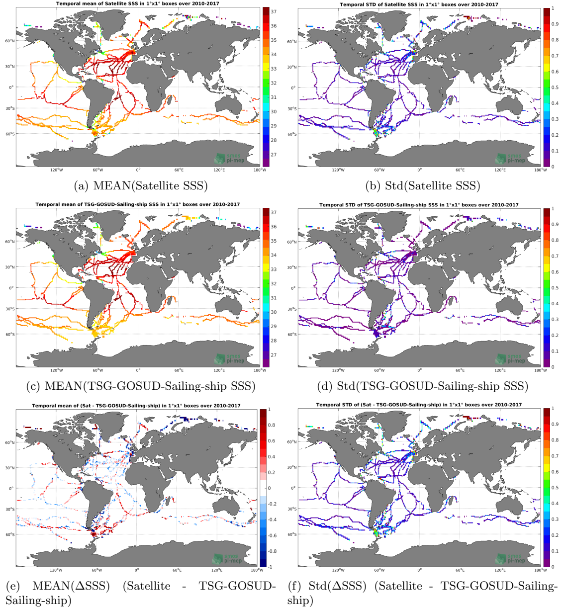
Figure 6: Temporal mean (left) and Std (right) of SSS from SMOS-L3-CATDS-IFREMER-CECOS-V2-MONTHLY-0.25DEG (top), TSG-GOSUD-Sailing-ship (middle), and of \Delta SSS (Satellite - TSG-GOSUD-Sailing-ship). Only match-up pairs are used to generate these maps.
