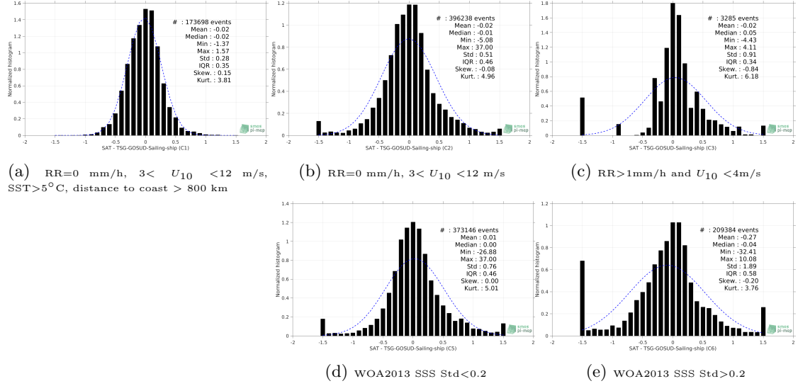
Figure 13: Normalized histogram of \Delta\text{SSS} (SMOS-L3-CATDS-IFREMER-CECOS-V2-MONTHLY-0.25DEG - TSG-GOSUD-Sailing-ship) for 5 different subdatasets corresponding to: RR=0 mm/h, 3 < U_{10} < 12 m/s, SST > 5^\circ\text{C} , distance to coast > 800 km (a), RR=0 mm/h, 3 < U_{10} < 12 m/s (b), RR > 1\text{mm/h} and U_{10} < 4\text{m/s} (c), WOA2013 SSS Std < 0.2 (d), WOA2013 SSS Std > 0.2 (e).
