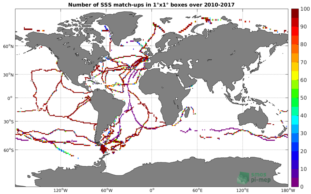
Figure 4: Number of SSS match-ups between TSG-GOSUD-Sailing-ship SSS and the SMOS-L3-CATDS-IFREMER-CECOS-V2-MONTHLY-0.25DEG SSS product for the Global Ocean Pi-MEP region over 1^\circ \times 1^\circ boxes and for the full satellite product period.
