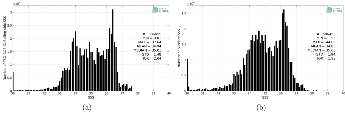
Figure 2: Histograms of SSS from TSG-GOSUD-Sailing-ship (a) and SMOS-L3-CATDS-IFREMER-CECOS-V2-MONTHLY-0.25DEG (b) considering all match-up pairs per bins of 0.1 over the Global Ocean Pi-MEP region and for the full satellite product period.
