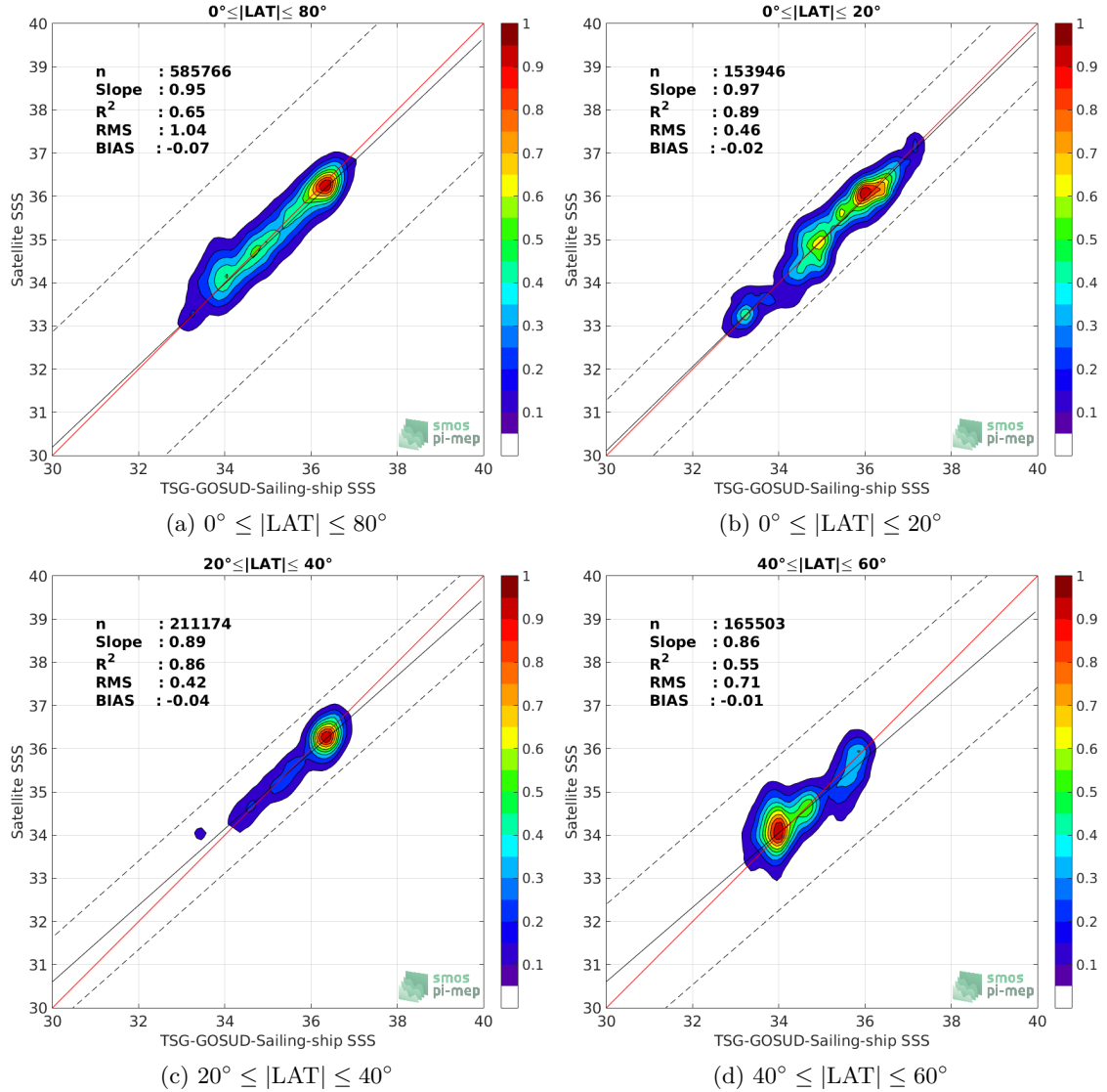
Figure 9: Contour maps of the concentration of SMOS-L3-CATDS-IFREMER-CECOS-V2-MONTHLY-0.25DEG SSS (y-axis) versus TSG-GOSUD-Sailing-ship SSS (x-axis) at match-up pairs for different latitude bands. For each plot, the red line shows x=y . The black thin and dashed lines indicate a linear fit through the data cloud and the \pm 95\% confidence levels, respectively. The number match-up pairs n , the slope and R^2 coefficient of the linear fit, the root mean square (RMS) and the mean bias between satellite and in situ data are indicated for each latitude band in each plots.
