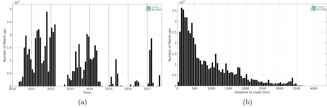
Figure 1: Number of match-ups between TSG-GOSUD-Sailing-ship and SMOS-L3-CATDS-IFREMER-CECOS-V2-MONTHLY-0.25DEG SSS as a function of time (a) and as function of the distance to coast (b) over the Global Ocean Pi-MEP region and for the full satellite product period.
