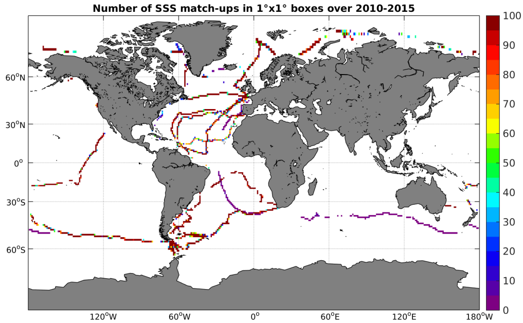
Figure 4: Number of SSS match-ups between TSG-GOSUD-Sailing-ship SSS and the SMOS-L3-CATDS-IFREMER-CECOS-V2-MONTHLY-0.25DEG SSS product for the Global Ocean Pi-MEP region over 1°x1° boxes and for the full satellite product period.
