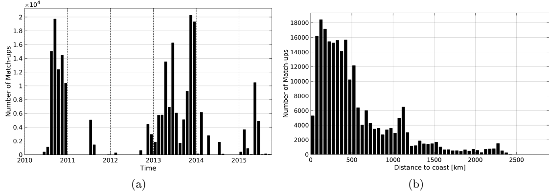
Figure 1: Number of match-ups between TSG-GOSUD-Sailing-ship and SMOS-L3-CATDS-IFREMER-CECOS-V2-MONTHLY-0.25DEG SSS as a function of time (a) and as function of the distance to coast (b) over the Global Ocean Pi-MEP region and for the full satellite product period.
